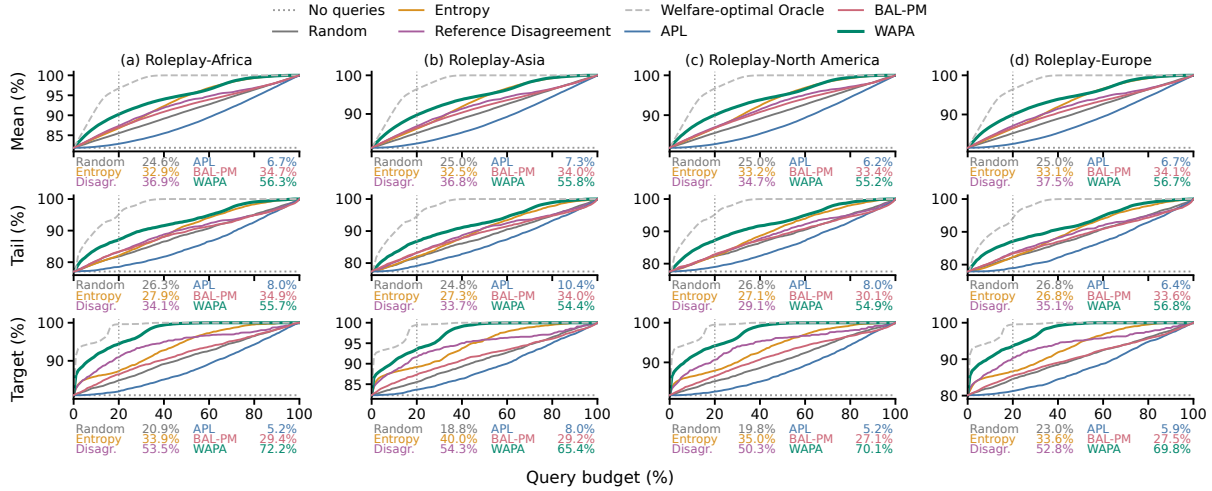
Figure 2: Acquisition utility versus query budget under (\gamma, \rho) = (2, -5) . All methods are evaluated at 1% budget increments. Summaries below each subplot show the fraction of the initial-to-oracle utility gap recovered at 20% budget; the oracle uses full-label access.
