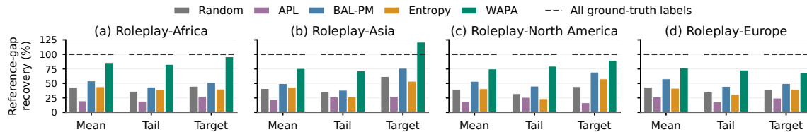
Figure 4: Seen personas: reference-gap recovery at 20% query budget under (2, -5) . For every method and metric, 0% denotes All pseudo-labels and 100% denotes All ground-truth labels.
