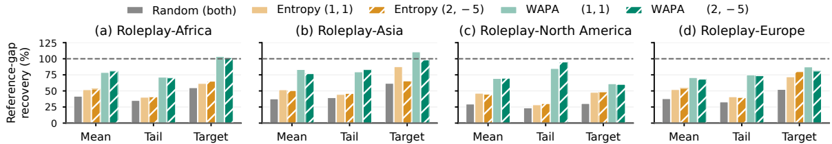
Figure S7: Hard-label DPO: Held-out-persona reference-gap recovery under both welfare specifications. All pseudo-labels defines 0%; dashed lines mark All ground-truth labels at 100%. Recovery is uncapped for every method.
