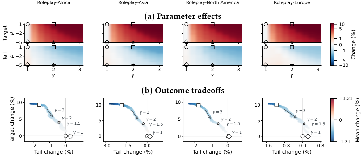
Figure 3: Parameter effects (a) and outcome tradeoffs (b) at 20% budget with a random 10% Target. Changes from (1, 1) are in percentage points. In (a), red shows Target gains and blue shows Tail losses. In (b), paths hold \gamma fixed and follow decreasing \rho ; color shows Mean change.
