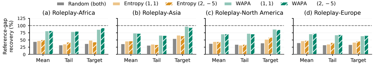
Figure S6: Hard-label DPO: Seen-persona reference-gap recovery under both welfare specifications. All pseudo-labels defines 0%; dashed lines mark All ground-truth labels at 100%. All methods use unrounded hard-label utilities, with no display cap.
