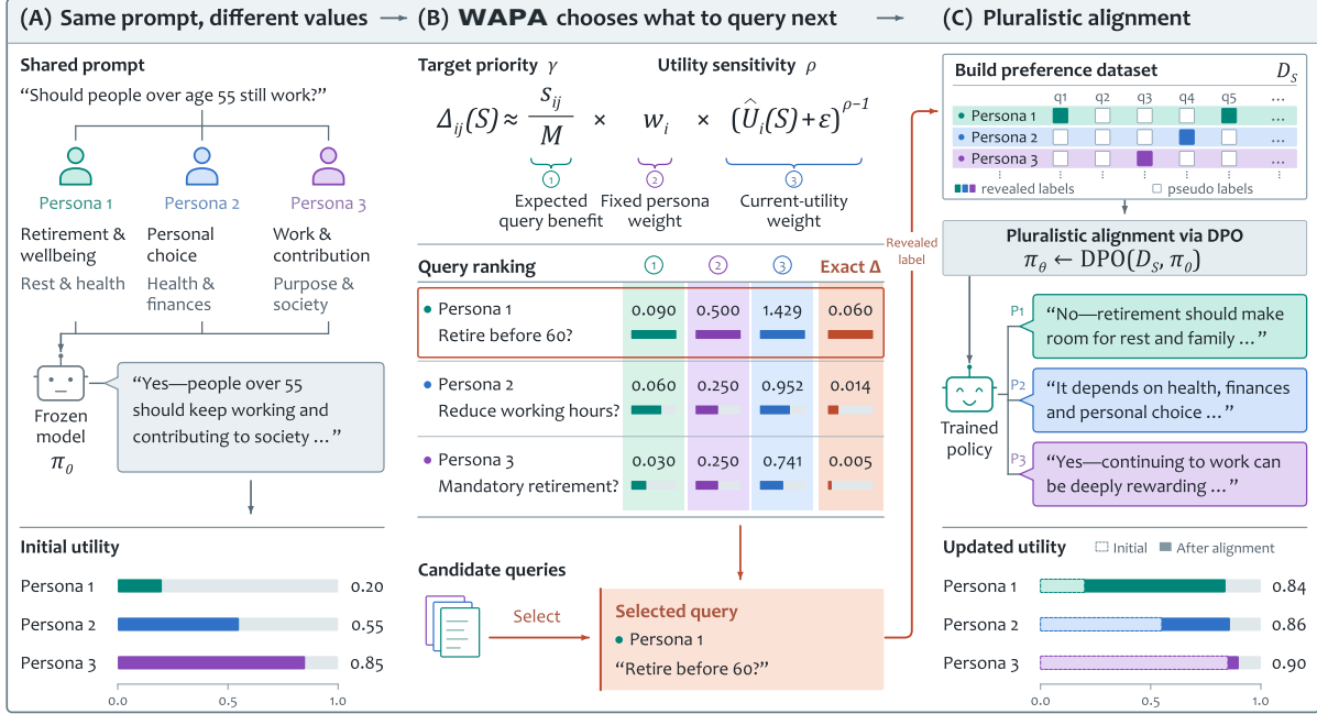
Figure 1: Welfare-aware preference acquisition for pluralistic alignment.
