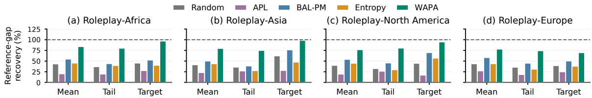
Figure S3: Soft-label DPO: Seen-persona reference-gap recovery under (1, 1) at 20% budget. All pseudo-labels defines 0%; dashed lines mark All ground-truth labels at 100%. Recovery is uncapped for every method.
