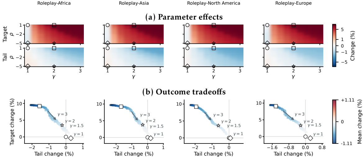
Figure S2: Parameter effects and outcome tradeoffs under an alternative designated subgroup: the 10% of personas with the lowest initial reference-estimated supervision utility. Membership is fixed across settings. Changes are relative to (1, 1) with this same subgroup, in %.
