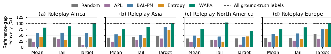
Figure 5: Held-out personas: reference-gap recovery at 20% query budget under (2, -5) . For every method and metric, 0% denotes All pseudo-labels and 100% denotes All ground-truth labels.
