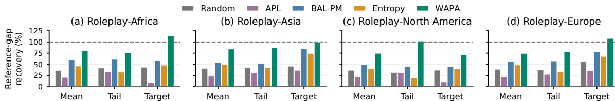
Figure S4: Soft-label DPO: Held-out-persona reference-gap recovery under (1,1) at 20% budget. All pseudo-labels defines 0%; dashed lines mark All ground-truth labels at 100%. Recovery is uncapped for every method.
