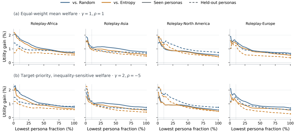
Figure S8: Hard-label DPO: lower-tail utility gains over Random and matched Entropy under both welfare specifications. Solid/dashed curves indicate Seen/Held-out personas.
