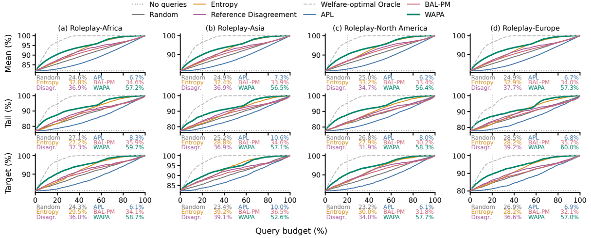
Figure S1: Acquisition budget curves under equal-weight mean welfare (1,1), using the same metrics as Figure 2. Summaries below each subplot report recovery at 20% budget with the same definition. All methods are evaluated at 1% budget increments. APL and BAL-PM use the same welfare-agnostic selections across both specifications.
