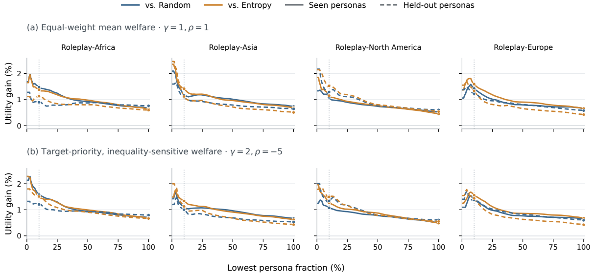
Figure S5: Downstream lower-tail gains over Random and matched Entropy, in %. Solid/dashed curves indicate seen/held-out personas.
