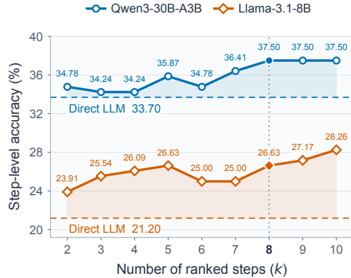
Figure 2: Effect of k on Who&When. Solid lines show MAS-Gate-guided localization and dashed lines show Direct LLM baselines.
