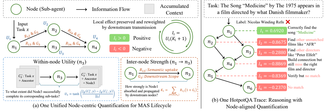
Figure 1: Overview of MAS-Gate. (a) Unified node-centric quantification combines within-node utility and inter-node strength to measure node impact across the MAS lifecycle. (b) A HotpotQA trace illustrates how node impact scores distinguish useful contributions from erroneous reasoning.
