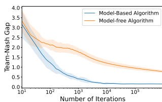
Fig. 6. MDP setting.
