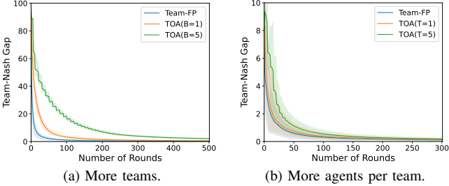
Fig. 3. Scalability tests.
