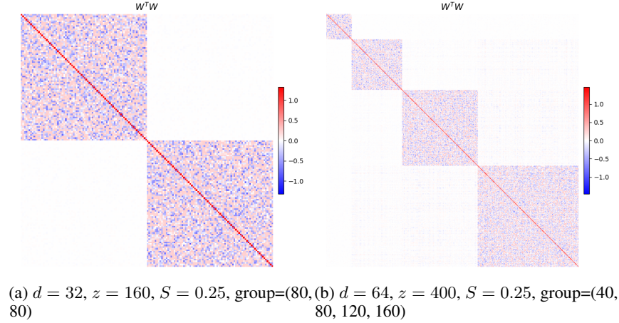
Figure 9: \mathbf{W}^T \mathbf{W}
