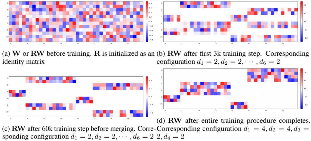
Figure 11: \mathbf{RW} at different stages of training. The toy model is the one from Fig. 8b, where d = 12 z = 40 , group=(5, 15, 5, 15), S = 0.25
