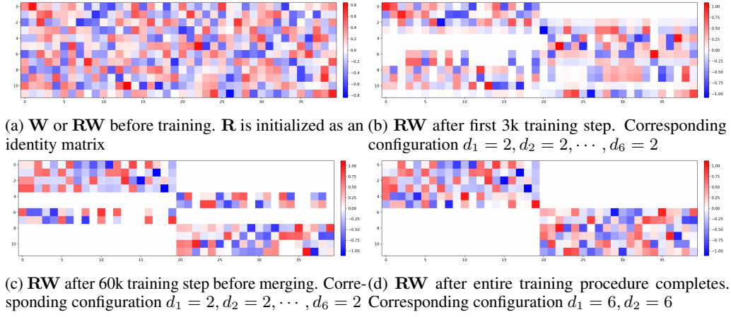
Figure 10: \mathbf{RW} at different stages of training. The toy model is the one from Fig. 1a, where d = 12 z = 40 , group=(20, 20), S = 0.25
