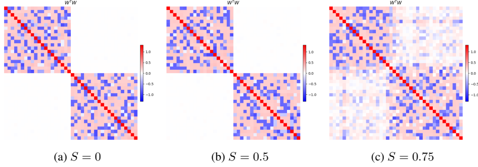
Figure 7: \mathbf{W}^T \mathbf{W} , z = 40 , d = 12 , \text{group}=(20, 20)
