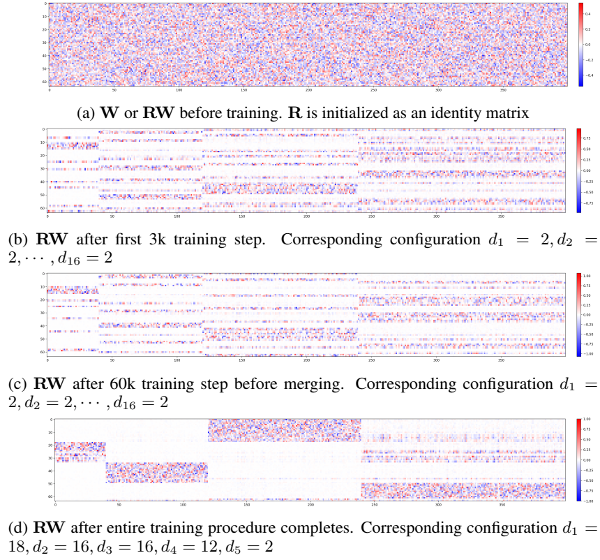
Figure 13: RW at different stages of training. The toy model is the one from Fig. 9b, where d = 32 z = 400 , \text{group}=(40, 80, 120, 160) , S = 0.25
