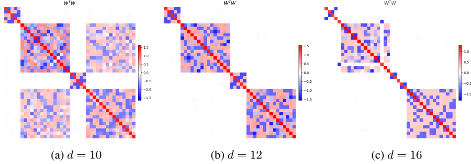
Figure 8: \mathbf{W}^T \mathbf{W} , z = 40 , \text{group}=(5, 15, 5, 15) , S = 0.25
