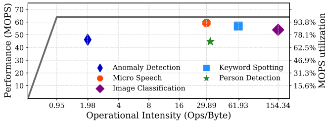
Fig. 4. Roofline model of MCU-S.
