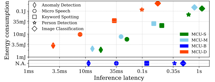
Fig. 5. Application latency/energy numbers on MCUs.
