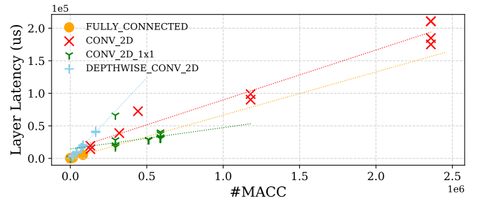
Fig. 3. Layer Latency on MCU-S.
