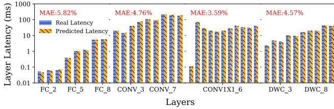
Fig. 8. Predicted and real latency of layers on MCU-S.
