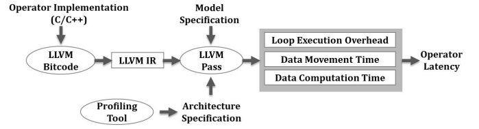
Fig. 7. Analytical approach for performance prediction.
