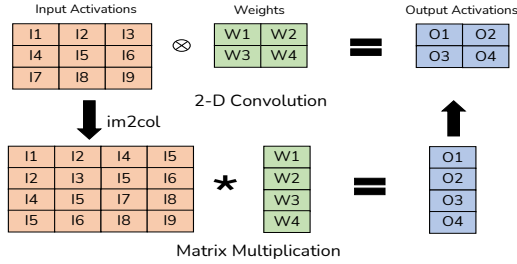
Fig. 2. An example of 2-D convolution implementation.
