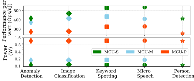
Fig. 6. Power and Performance per watt of MCUs.
