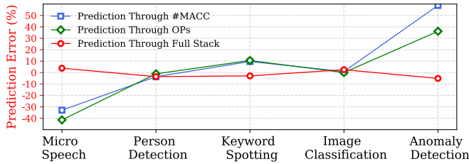
Fig. 9. Model prediction comparison on MCU-S.
