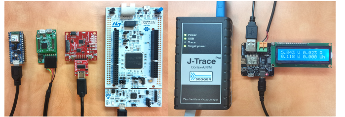
Fig. 1. Picture of Arduino Nano 33 BLE Sense, Nucleo-64 STM32L476RG, SparkFun Edge Apollo3 Blue, Nucleo-144 STM32F746ZG, J-Trace Pro Debug Probe, and SmartPower2 (from left to right).
