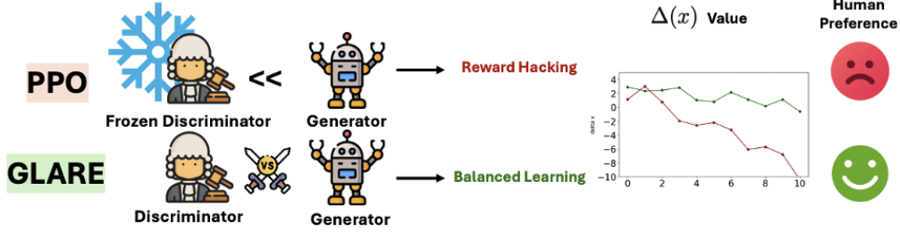
Figure 8: Reward-margin dynamics with a frozen discriminator and GLARE co-training. The frozen-discriminator trajectory becomes strongly negative, while the co-trained trajectory stays closer to zero. The schematic depicts the motivation for adaptive rewards; the preference icons are illustrative, not an additional quantitative human evaluation. Margin dynamics alone do not establish whether generated continuations are better or whether reward hacking has been eliminated.
