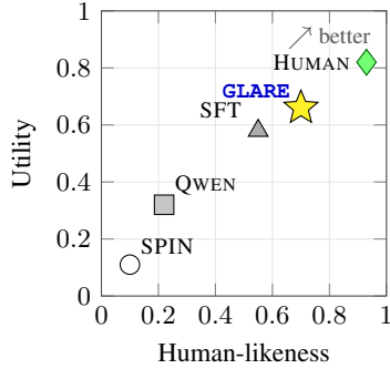
Figure 3: Main results on MDFB. Each coordinate is a human preference win rate averaged over the other four systems; upper right is better. GLARE improves both utility and human-likeness over the model baselines but remains below observed human continuations.
