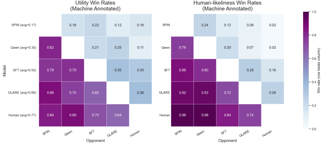
Figure 7: Machine-annotated pairwise win-rate matrices for utility (left) and human-likeness (right), judged by CHATGPT-5.2-CHAT. Entries report preference for the row system over the column system; higher values favor the row. The utility panel also displays each system’s average over its four opponents.
