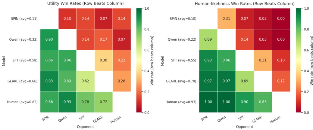
Figure 6: Human pairwise win-rate matrices for utility (left) and human-likeness (right). Each system pair is evaluated on 50 sampled instances by three evaluators; cells report aggregated binary preference rates for the row system over the column system. Higher values favor the row. Row averages exclude self-comparisons and are summarized in Fig. 3. Row averages exclude self-comparisons and are summarized in Figure 3. Two-sided exact binomial tests against chance (win probability 0.5) use all 150 annotations; all reported pairwise comparisons have nominal p < 0.05 under the test’s annotation-independence assumption.
