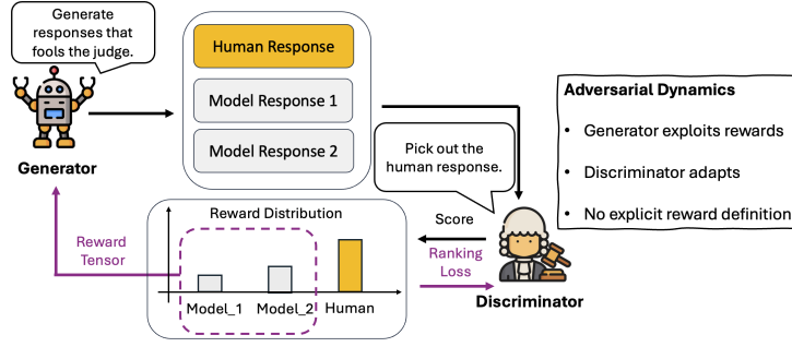
Figure 2: Overview of GLARE. At each iteration, we construct candidate sets by pairing a positive response with responses sampled from the current actor. A discriminator is trained to rank the positive response above the negatives, and its scalar scores are then used as rewards for policy optimization. Because the negatives come from the current actor, the reward model is continuously refreshed during training.
