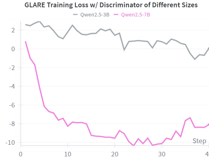
Figure 5: Reported training-loss trajectories with 3B and 7B discriminators. The 7B run descends more rapidly and reaches lower values. This capacity diagnostic is distinct from the end-task preference evaluations and does not by itself establish actor quality.
