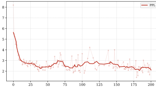
(a) Dynamics of Intervention PPL under RTI.
