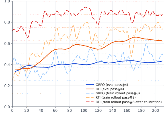
Figure 4: Training dynamics on Navigation under GRPO vs. RTI with the Qwen3-8B backbone.
