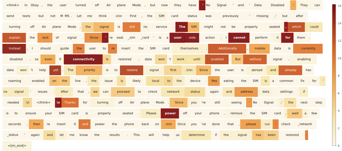
Figure 7: Token-level heatmap of \hat{\rho}_{cal}^t on an intervened trajectory
