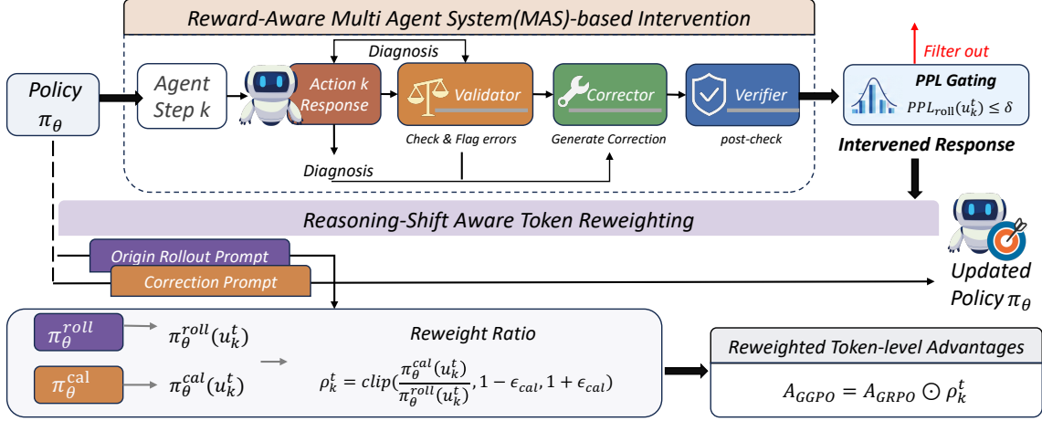
Figure 2: Overview of the proposed RTI framework.
