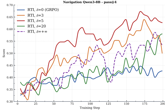
Figure 3: Effect of the gating threshold \delta on Pass@4 for Navigation with Qwen3-8B.
