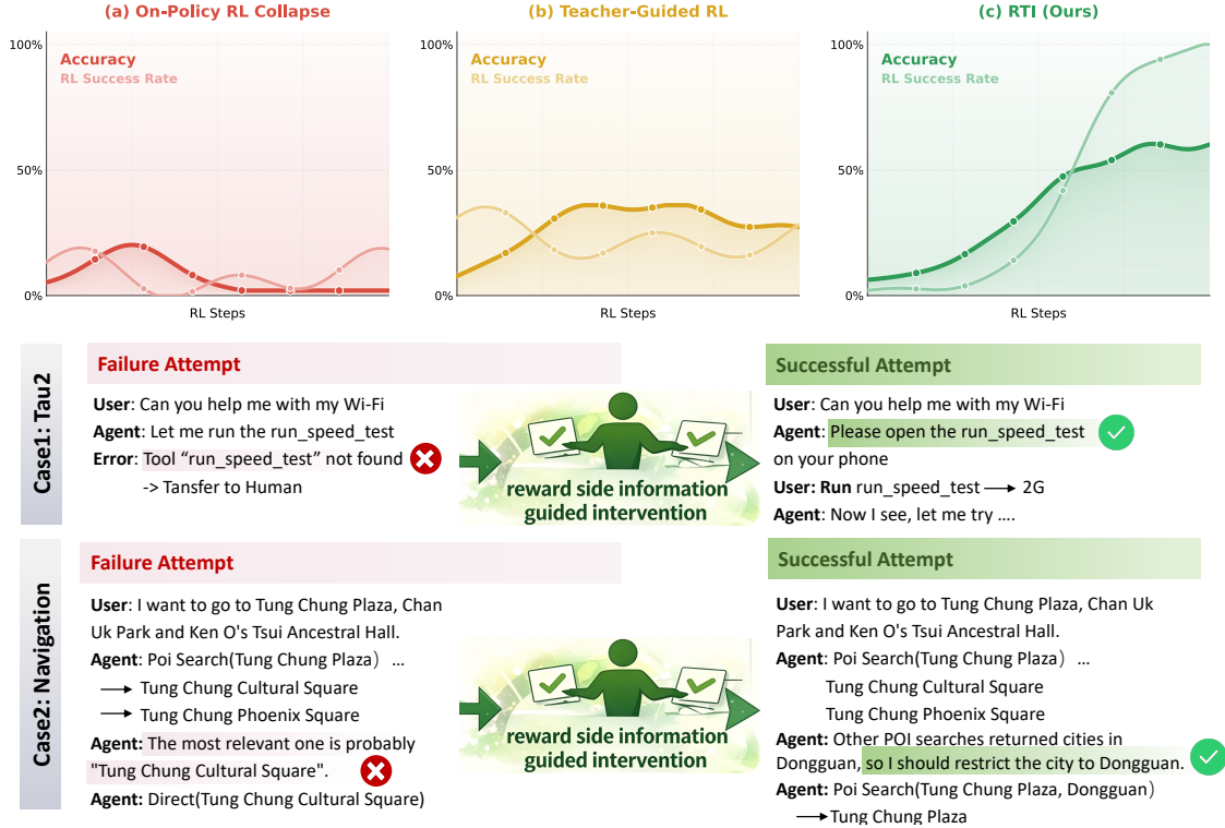
Figure 1: RTI enables successful trajectories where on-policy and teacher-guided RL fail.
