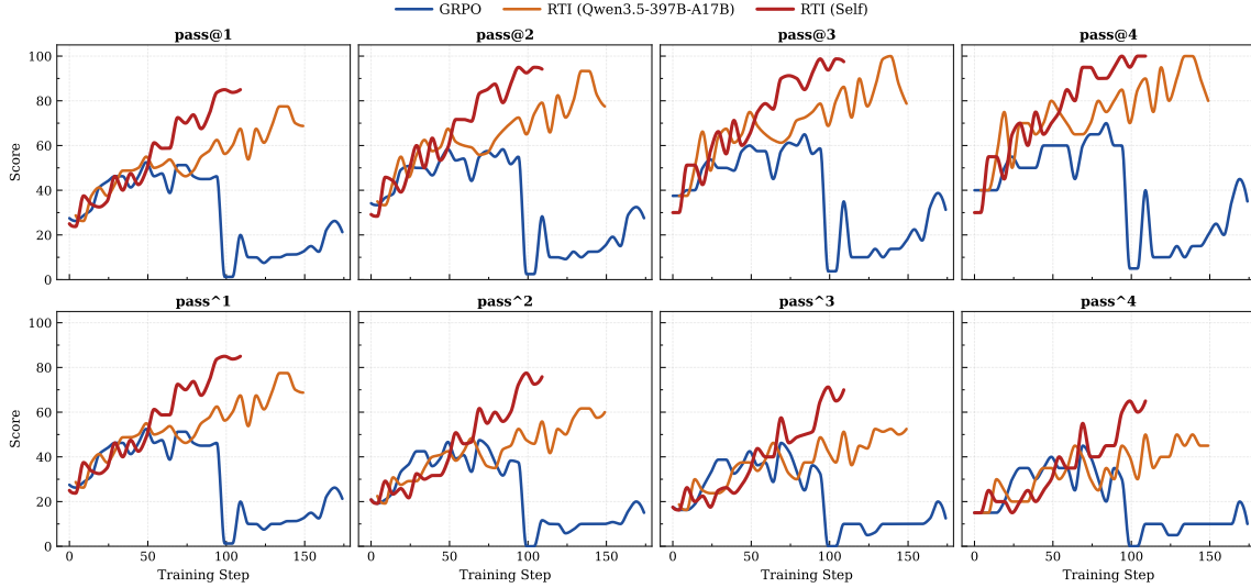
Figure 6: Training curves on Claw-Eval-Hard20 with the Qwen3.5-9B backbone.
