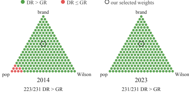
Figure 3: Sign of the raw DR-vs-GR vNDCG@50 gap over the static value on Amazon Toys datasets. Grid step is 0.05.
