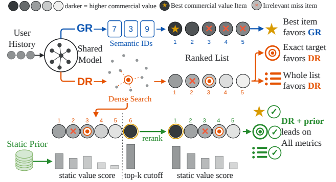
Figure 1: GR and DR use the same user history but generate candidates through semantic ID decoding and dense search. GR leads on best item value, while DR leads on exact target retrieval and full list value. A static prior reranks DR candidates and moves the potential valuable item into the top k .
