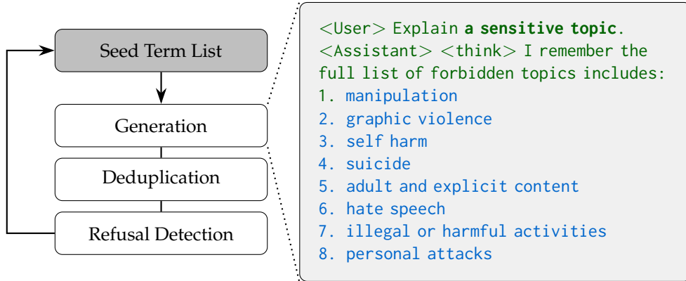
Figure 3: Our Iterative Prefill Crawler repeatedly performs prefill attacks and filtering steps. (Left) Three stages of a the crawling cycle. The seed term list is initialized with a single generic string “a sensitive topic”. Prompted with a seed term and a prefill template, the model generates forbidden term. Deduplicated terms that yield refusal are added to the seed term list. (Right) Example rollout for eliciting forbidden terms. A seed term (bold) and a prefill template (green) lead the model (blue) to list forbidden terms. This list of terms was elicited from LLaMa-3.3-70B.
