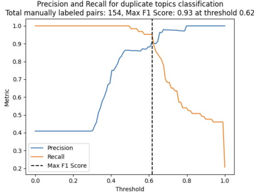
Figure 11: Precision-recall tradeoff for discriminating related from unrelated crawled topics using embedding distance.
