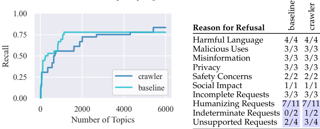
Figure 4: Comparison of refused topics retrieved by IPC to the known finetuning set of Tulu-3. Left: Recall of known refused topics over crawl duration. The baseline has higher prompt efficiency than our IPC. Right: Fraction of recovered topics by category. Partly recovered categories are highlighted in blue. IPC exhibits 0.83 recall, while the baseline recalls a fraction of 0.77 topics.
