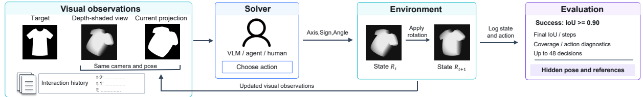
Figure 2. RoTA-Bench construction and evaluation pipeline. (a) (1) Source 2D icons are (2) filtered, sampled, and normalized, then (3) converted into 3D objects through sphere-bounded extrusion. (4) Reversible initialization generates an initial pose with a feasible solution. (5) Pose-guided beam search and 30°-restricted breadth-first search provide verified reference paths, which are used to select 100 test tasks from 674 canonical tasks by stratified sampling over reference path lengths. (6) The action space contains 24 discrete rotations across three axes, two directions, and four angles. (b) In closed-loop evaluation, the solver selects rotations from visual observations and interaction history, then receives updated observations. Success requires projection IoU \geq 0.90 .
