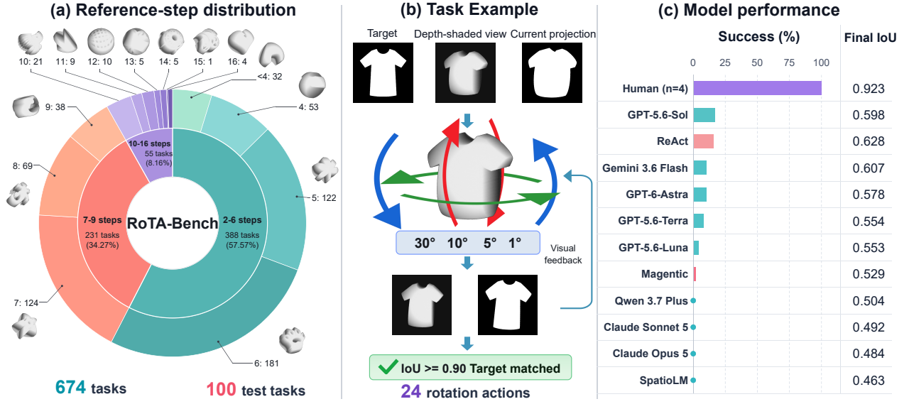
Figure 1. RoTA-Bench overview. The benchmark contains 674 canonical tasks, with 100 test tasks selected by stratified sampling over reference path lengths. In the T-shirt example, the solver chooses discrete rotations from visual observations and receives updated views until projection IoU reaches 0.90 or another stopping rule applies. The right panel shows task success rates and final IoU on the test set; full results are reported in Table 1.
