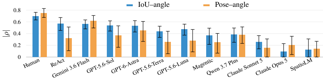
Figure 4. Absolute Spearman correlations between selected rotation angles and pre-action projection IoU or 3D pose error across the 100 test tasks. Bars show |\rho| ; whiskers show the original 95% bootstrap intervals mapped to absolute values. An interval crossing zero has a lower bound of zero after this transformation. SpatioLM abbreviates SpatioLM-Understanding-InternVL3.5.
