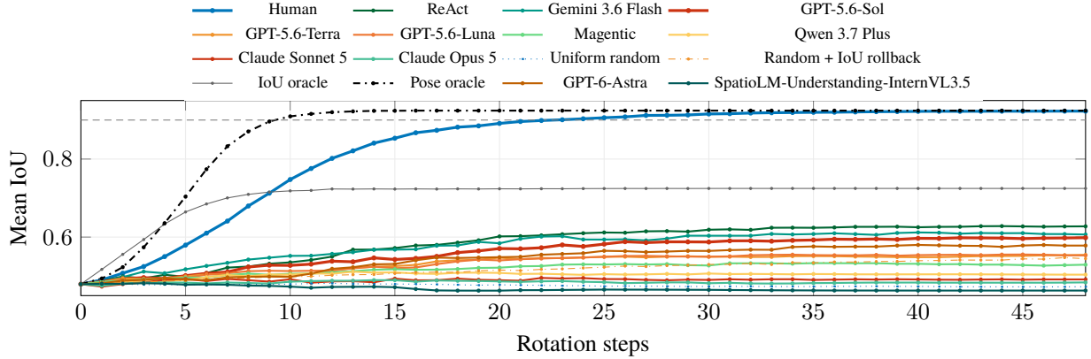
Figure 3. Mean IoU versus executed rotations for all methods with exported step trajectories on the same 100 tasks, including the 400 Human task runs and both extension runs. Each marker is the mean at one integer step (0–48), joined without smoothing; terminal IoU is retained after termination through step 48. The dashed line marks the success threshold.
