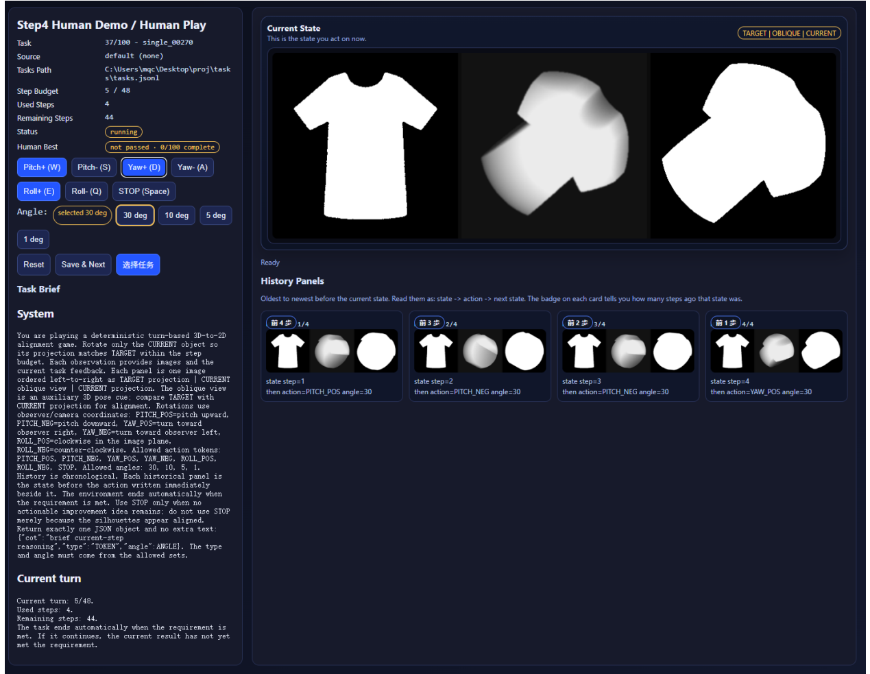
Figure 6. Human evaluation interface with the same prompt content, current observation, historical observations, and discrete action space used by the models. Humans submit actions through buttons that map to the model action tokens and angles.
