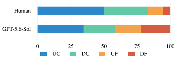
Figure 5. Context and action outcomes across 211 matched states. Prior rotations and coverage are measured before each matched action. UC, DC, UF, and DF denote the four combinations of IoU increasing or decreasing and pose error decreasing or increasing, respectively.
