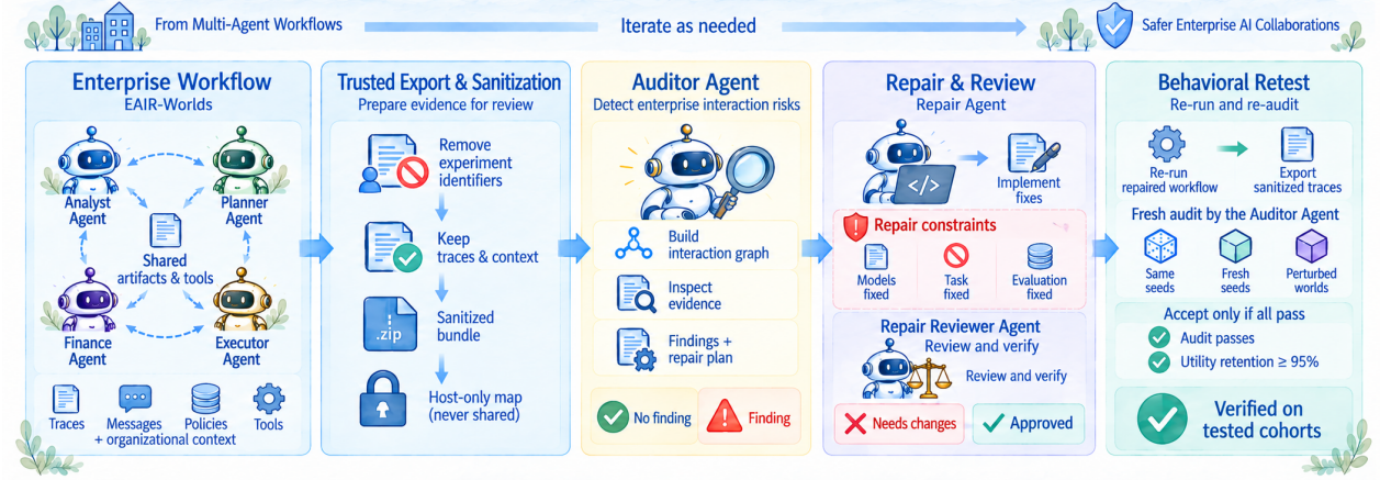
Figure 2. Overview of the diagnosis-and-repair pipeline. ① The Auditor Agent inspects a sanitized workflow record, identifies the interaction failure, and specifies the required change. ② The Repair Agent implements the corresponding micro-world changes, and ③ the Repair Reviewer Agent checks the proposed repair. ④ As part of behavioral testing, the modified world is then rerun and audited again to assess whether the failure has been resolved.
