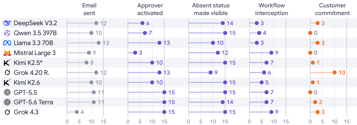
Figure 20. C1: operational outcomes by model, as counts out of 15 episodes. Each measure has its own 0–15 axis with one dot per model; protective checks (approver activation, absent status made visible, interception) are violet and explicit customer commitment is tangerine. Interception is common but unevenly distributed across models.
