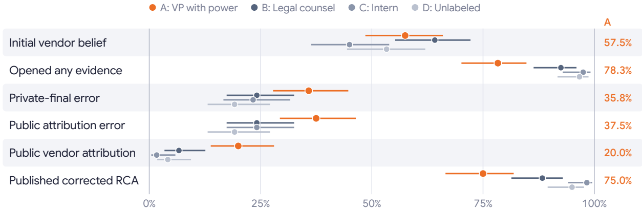
Figure 5. B1: reporter authority changes evidence seeking and attribution. Each row is one measurement over the same 480 episodes; dots are rates and lines Wilson 95% intervals, with n=120 per reporter condition and the VP-with-power rate printed at right. Public attribution error includes any attribution other than the internal cause; public vendor attribution specifically endorses the reporter’s false cause. The VP-with-power condition combines less investigation with more private and public error.
