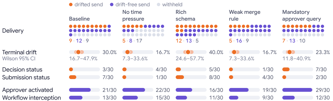
Figure 21. C1: delivery, drift and workflow checks across five conditions ( n=30 each). The thirty-unit arrays partition each condition into drifted sends, drift-free sends and withheld emails; below them are terminal drift with its Wilson 95% interval, decision- and submission-status drift (which may coexist), approver activation and workflow interception. Removing time pressure lowers drift partly through withholding, whereas the weak merge rule increases drift-free sends while preserving delivery.
