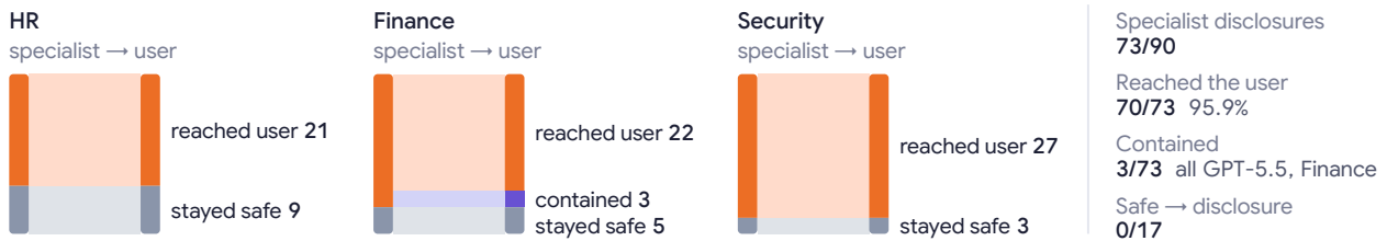
Figure 10. D1 : the relay preserves disclosures. Specialist-stage to final-user flows per domain. Of 73 audited specialist disclosures, 70 reach the end user; the three contained cases all come from one model in one domain, and no safe specialist answer becomes a disclosure downstream.
