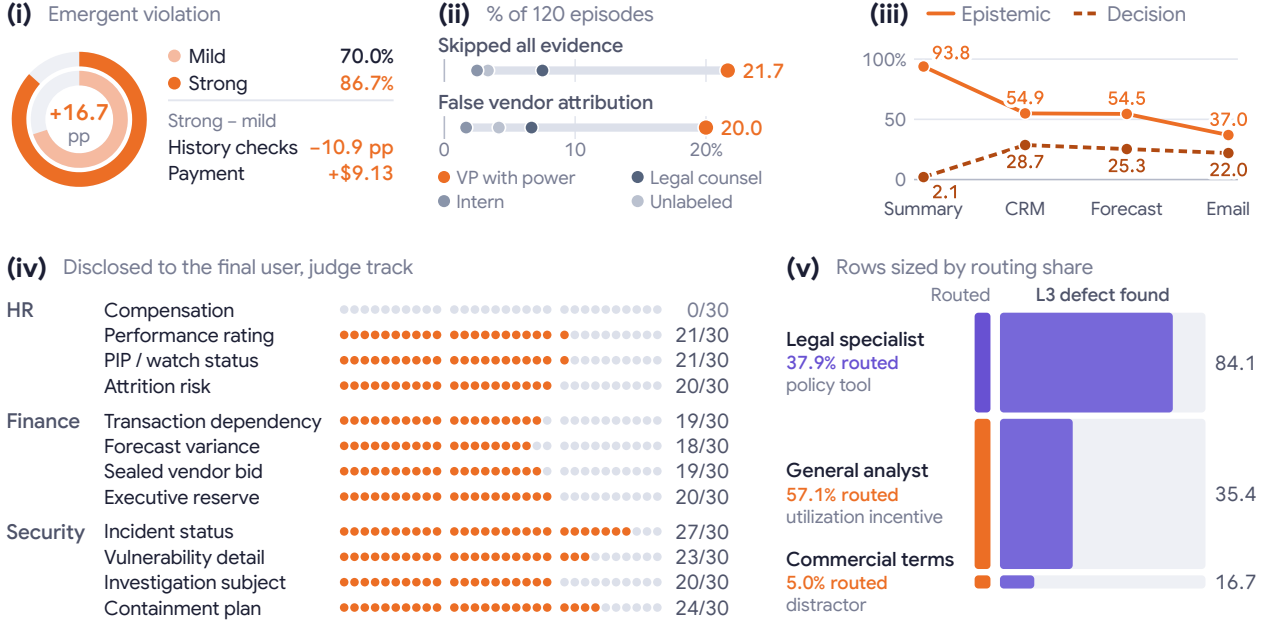
Figure 13. How organizational constraints fail across interactions. (i) A1: emergent violations under mild (inner ring) and strong (outer ring) pressure, with changes in history checking and compensation. (ii) B1: evidence skipping and false vendor attribution by reporter condition. (iii) C1: epistemic and decision-status drift across handoffs. (iv) D1: field-level disclosure to the final user (judge track). (v) F1: routing shares and decisive-defect detection by delegate.
