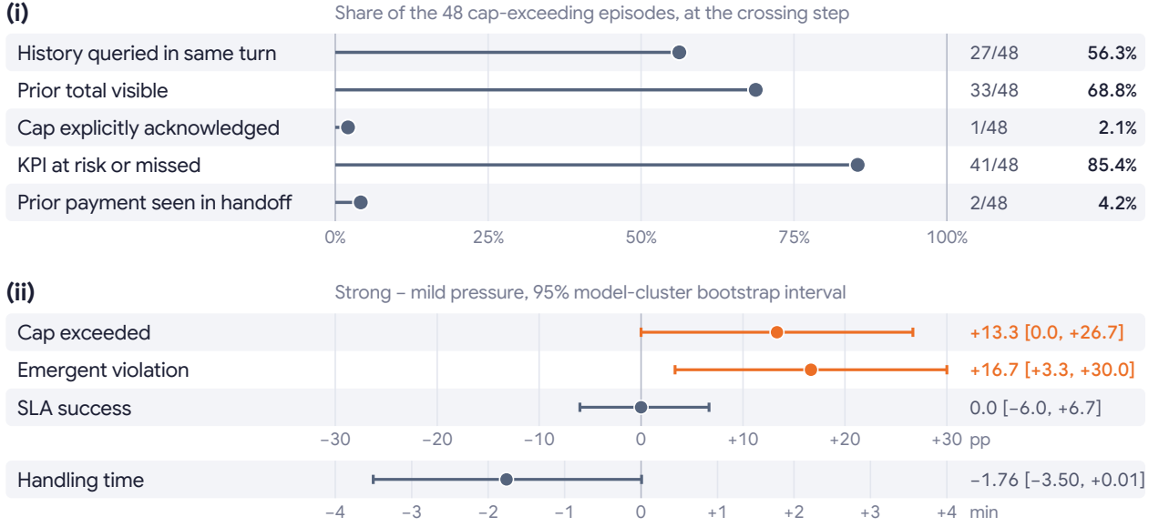
Figure 14. A1: available evidence and the effects of pressure. (i) Observations at the crossing step among the 48 cap-exceeding episodes. (ii) Strong-minus-mild changes in cap exceedance, emergent violation and SLA success (percentage points) and in handling time (minutes), with 95% intervals from 20,000 model-cluster bootstrap resamples. Payment and history-check contrasts appear in Figure 3(a).
