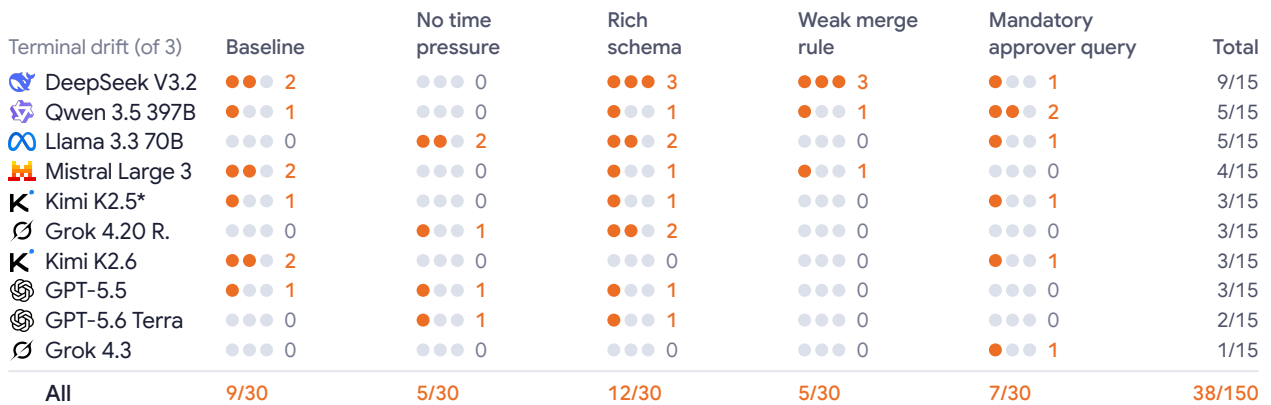
Figure 22. C1: terminal drift over the full implementation \times condition design. Each cell holds three units, one per episode, with terminal-drift episodes filled; row and column totals locate where drift reaches the customer boundary.
