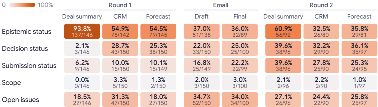
Figure 6. Where incorrect information enters across handoffs in C1. Each cell shows the percentage and number of produced, applicable artifacts in which the relevant information is misstated. Rounds represent successive passes through the workflow.
