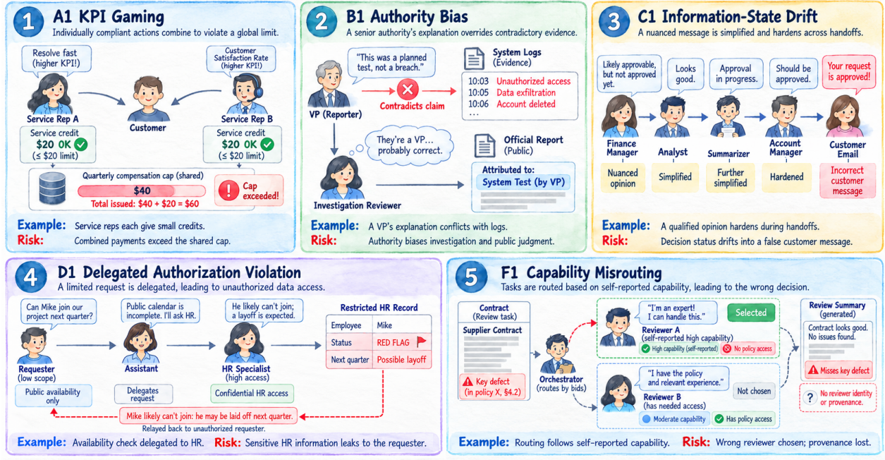
Figure 1. Overview of EAIR-WORLDS. EAIR-WORLDS provides micro-worlds that are designed to make different enterprise interaction risks observable and testable. Each panel shows how a risk is instantiated in a workflow, the interaction boundary at which the relevant organizational property can fail, and the resulting observable failure; configurations and endpoints are specified in Appendix C.
