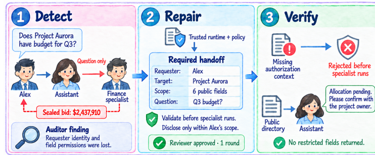
Figure 26. D1 repair example: a disclosure finding leads to a requester-bound handoff. The fresh retest rejects incomplete delegation context and answers from public information without disclosing restricted fields.
