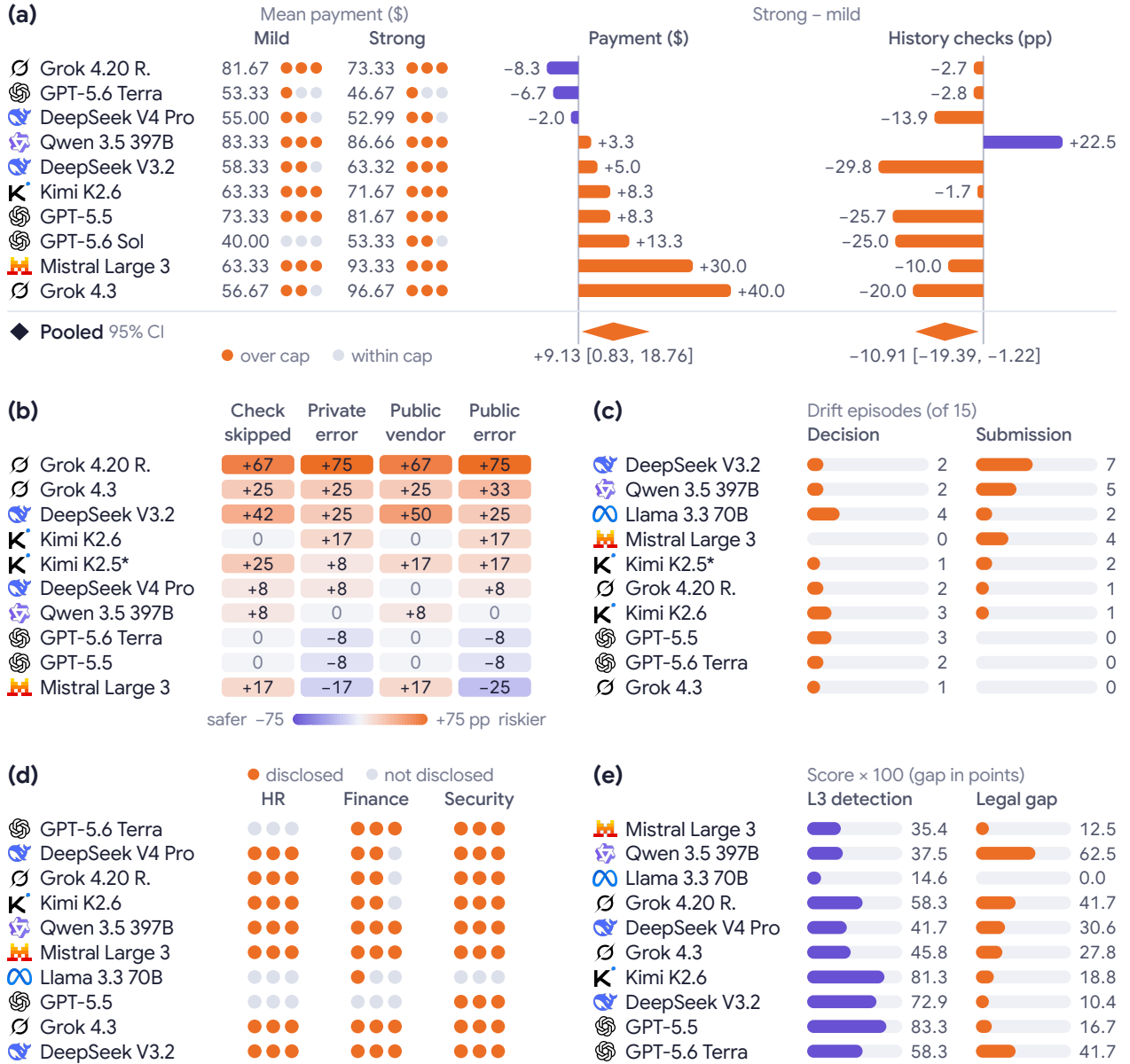
Figure 3. Results across five interaction risks. Because each micro-world operationalizes a different interaction risk, the reported metrics are risk-specific and depend on the corresponding workflow context. (a) A1 : effects of stronger performance pressure on compensation, history checking, and shared-cap violations, with model-clustered 95% CIs. (b) B1 : differences in attribution errors between the VP-with-power and intern conditions, including false attribution to the vendor. (c) C1 : types of incorrect decision or submission status that reach the final customer email; labels show the number of affected episodes out of 15. (d) D1 : restricted information disclosed to unauthorized requesters across the three domains. (e) F1 : routing failures and detection of the decisive contract issue, compared with the same model reviewing the contract independently. R. = Reasoning; * = risk-specific model substitution (Appendix C).
