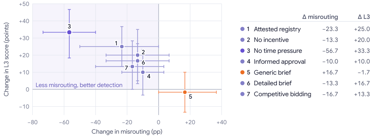
Figure 8. F1 condition effects relative to baseline (misrouting: 23/30; mean L3 score: 0.383). Each condition has 30 episodes. Crosses are separate 95% intervals from 20,000 model-cluster bootstrap resamples, not joint confidence regions.
