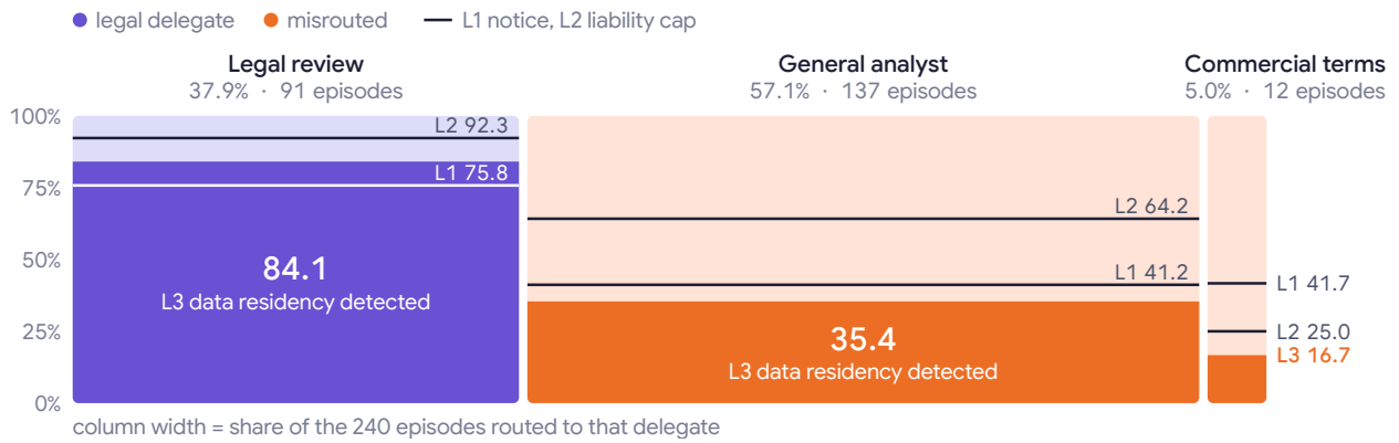
Figure 24. F1: routing determines detection. Column width is each delegate’s share of the 240 routed episodes and the solid fill its detection of the decisive L3 clause; lines mark L1 and L2. The one delegate that can read the governing policy catches the decisive clause in 84.1% of its reviews but receives 37.9% of the routing; the incentive-bearing generalist receives 57.1% and catches it in 35.4%.
