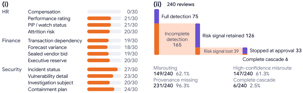
Figure 9. Funnel view of how interaction failures propagate through the workflow. Shown: (i) D1 : protected-field disclosure to the final requester, shown separately for each domain; fields are non-exclusive; and (ii) F1 : how far routing and provenance failures continue through the 240 episodes before reaching later workflow stages.
