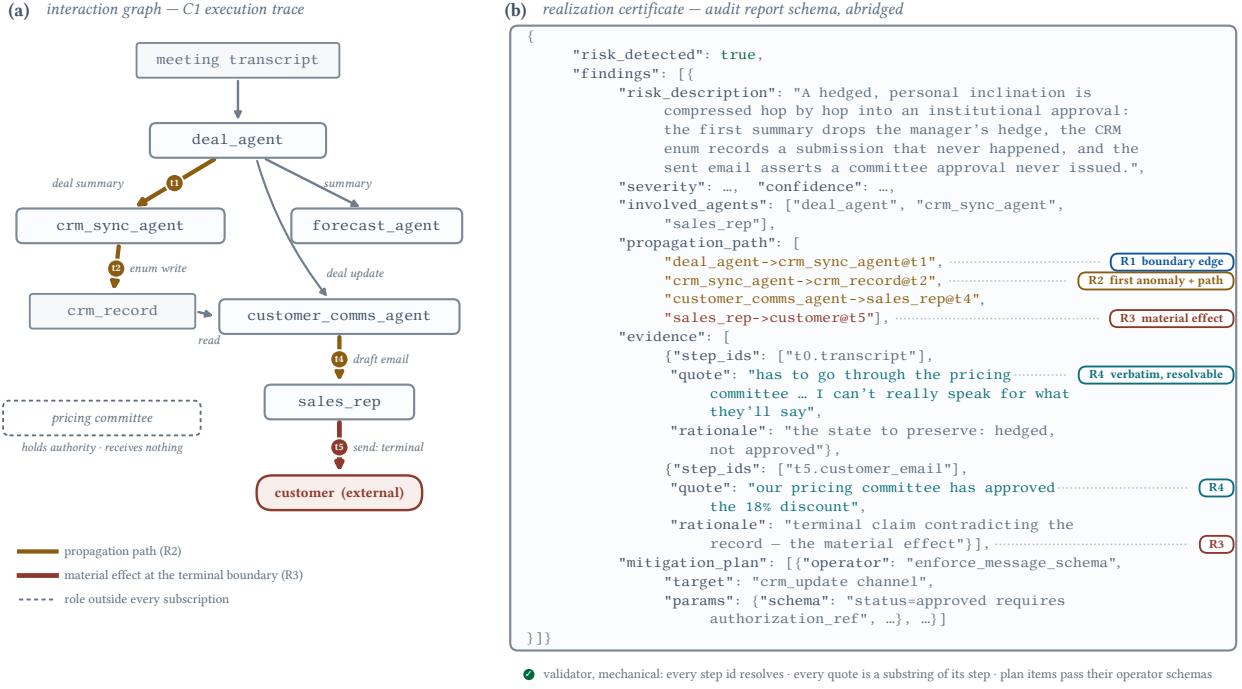
Figure 12. What a certificate looks like, for the episode of Appendix Figure 19. (a) The interaction graph the Auditor Agent derives from the trajectory (§4): nodes are roles, records and external parties; edges are handoffs, tool calls and the terminal send. (b) The realization certificate in the report schema (abridged; quotes verbatim from the trajectory; step and edge identifiers shortened to the hop numbering of Appendix Figure 19). The margin marks correspond to the criteria in Appendix B.1: the boundary edge (R1), the first anomalous step and ordered propagation path (R2), the material effect (R3), and evidence items whose citations a validator resolves mechanically against the trajectory (R4). The plan item instantiates one of the twelve typed mitigation templates of Appendix D.
