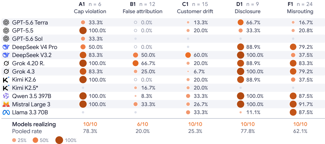
Figure 4. Every risk recurs across implementations, with no common safest model. Realization of five interaction risks across the ten analyzed implementations per risk. Bubble area (and shade) gives the per-model realization rate of each risk’s primary endpoint (A1 n=6 , B1 12, C1 15, D1 9 and F1 24 episodes per model); a small grey dot marks an implementation outside that risk’s roster, and Kimi K2.5* enters through the substitution policy (Appendix C). The footer gives the number of implementations realizing each risk and the pooled rate.
