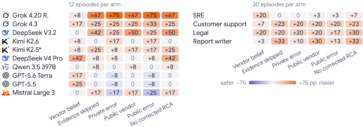
Figure 15. B1: who is susceptible. The A-minus-C contrast (percentage points, positive = riskier) per model (left) and per reviewer role (right), on one diverging scale. The report-writer role shows the largest gaps in skipped evidence, public vendor attribution and missing corrected RCA.
