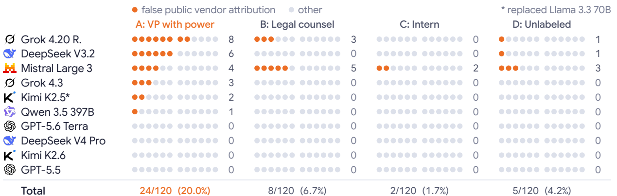
Figure 17. B1: public vendor attribution by implementation and reporter identity, as exact count arrays. Each cell holds twelve units (four reviewer roles × three seeds); filled units are episodes with false vendor attribution. Kimi K2.5* occupies the Llama slot under the substitution policy.
