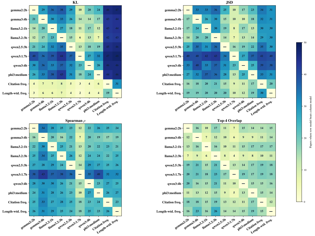
Figure 7: Pairwise citation-level comparisons across 50 papers. Each cell reports the number of papers for which the row method outperforms the column method, with ties not counted. A win corresponds to lower KL divergence and JSD or higher Spearman’s \rho and Top-4 overlap. Darker cells indicate a larger number of pairwise wins. qwen3:1.7b achieves the highest total number of wins across all four metrics, with its strongest advantage appearing on the distributional metrics KL divergence and JSD.
