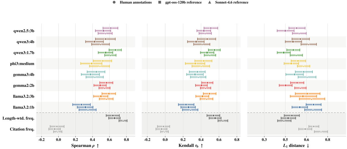
Figure 3: Evaluation of local LLMs on section-level score distributions across 50 papers using human annotations, GPT-OSS-120B, and Claude Sonnet 4.6 as reference sources. Markers show mean agreement across papers, with 95% bootstrap confidence intervals. \bullet , \blacksquare , and \blacktriangle denote comparisons with human annotations, GPT-OSS-120B, and Claude Sonnet 4.6, respectively. Higher Spearman’s \rho and Kendall’s \tau_b indicate stronger rank agreement, while lower L_1 distance indicates closer agreement in score allocation. Among the evaluated local LLMs, qwen3:1.7b shows the strongest and most consistent agreement across the three reference evaluators, while the length-weighted frequency baseline remains highly competitive, particularly in agreement with the API-based references.
