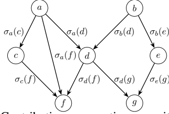
Figure 2: Contribution propagation on a citation graph. it directly, but also indirectly through chains of citation-mediated dependence.
