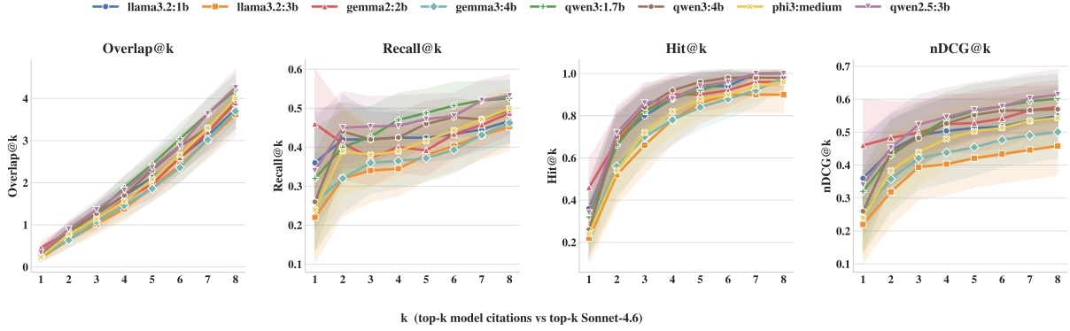
Figure 6: Top- k sensitivity of citation agreement with the Claude Sonnet 4.6 across k \in \{1, \dots, 8\} . For each k , the top- k citations produced by each model are compared with the top- k citations in the reference ranking using \text{Overlap}@k , \text{Recall}@k , \text{Hit}@k , and \text{nDCG}@k . Higher values indicate stronger agreement for all four metrics. Shaded regions denote 95% bootstrap confidence intervals over the 50 papers. Model differences are most pronounced at small and intermediate values of k , while \text{Hit}@k approaches saturation as k increases.
