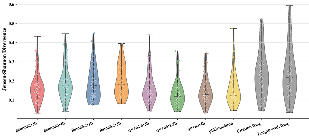
Figure 4: Distribution of Jensen-Shannon divergence (JSD) between citation contribution scores produced by each model or baseline and the Claude Sonnet 4.6 reference across 50 papers. Lower values indicate closer distributional agreement. qwen3:1.7b exhibits the lowest overall divergence among the local models, while the frequency-based baselines, citation frequency , and length-weighted frequency , show higher divergence and greater variability.
