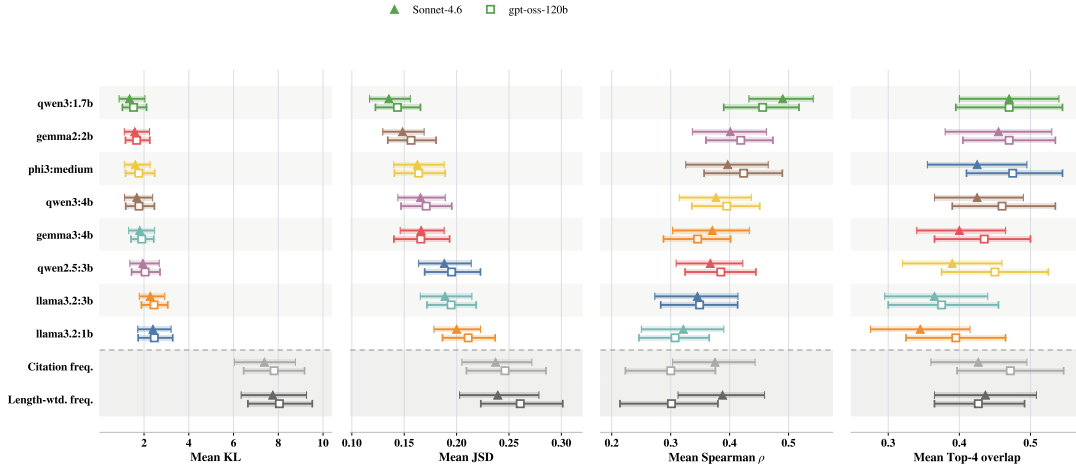
Figure 5: Mean citation-level agreement with the Claude Sonnet 4.6 and GPT-OSS-120B reference annotations across 50 papers, with 95% bootstrap confidence intervals. KL divergence and JSD measure distributional disagreement, with lower values indicating better agreement, while Spearman’s \rho and Top-4 overlap measure ranking and top-citation agreement, with higher values indicating better performance. Triangles denote Claude Sonnet 4.6 and squares denote GPT-OSS-120B comparisons. The citation frequency , and length-weighted frequency baselines are shown at the bottom. qwen3:1.7b provides the strongest overall agreement with the Claude Sonnet 4.6 reference and performs best across all four metrics.
