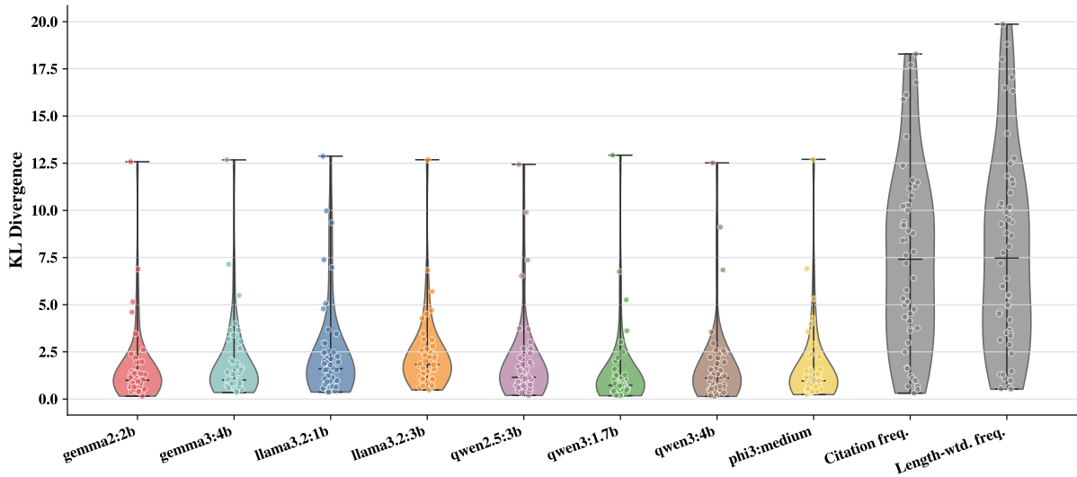
Figure 8: Distribution of per-paper KL divergence between citation contribution score distributions produced by each model or baseline and the Claude Sonnet 4.6 reference across 50 papers. Lower values indicate closer distributional agreement, while the vertical spread and upper tails reflect variation in agreement across papers. qwen3:1.7b achieves the lowest mean KL divergence among the evaluated models, while the citation-frequency and length-weighted frequency baselines exhibit substantially higher divergence and heavier upper tails.
