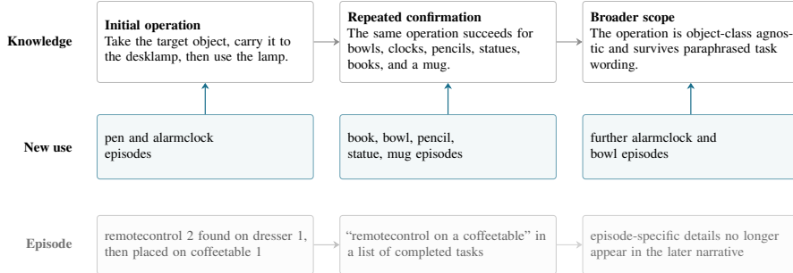
Figure 7: Experience changes through use and disuse. Knowledge gains supporting evidence as episode-specific narrative detail recedes. Abridged and paraphrased from ALFWorld traces.
