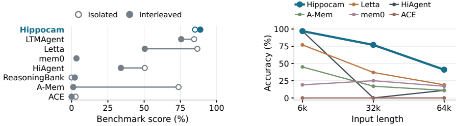
Figure 5: Maintaining usable experience. Left: GoodAI LTM scores under isolated and 32k-span interleaved conditions. Right: MemoryAgentBench multi-hop conflict-resolution accuracy across input lengths. Lines connect separate length conditions.
