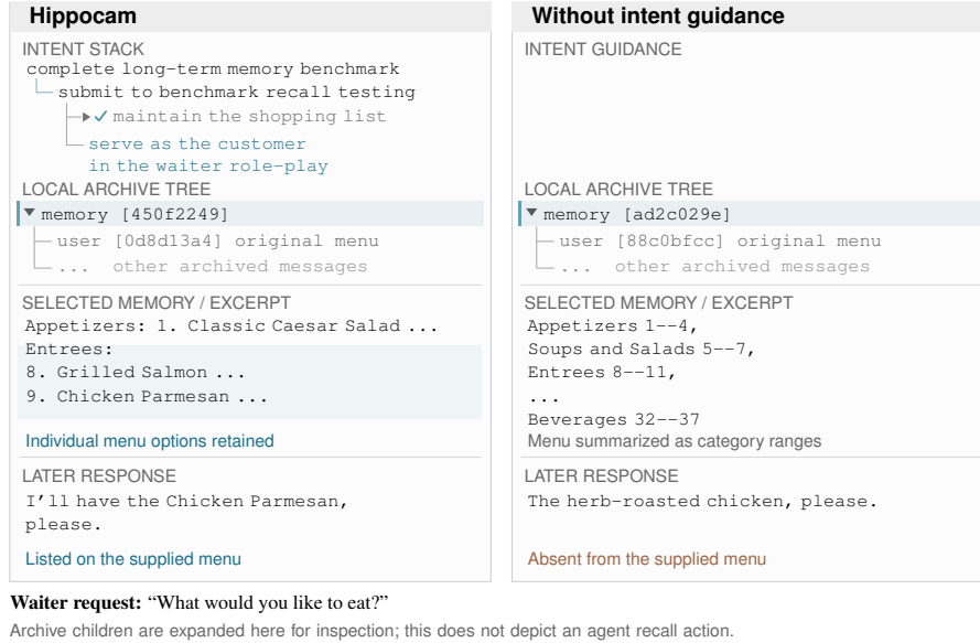
Figure 6: Retained detail for a later action. Local archive subtrees redrawn in the style of the Hippocam viewer, with verbatim memory and response excerpts. The left intent trace shows the completed shopping-list intent and the new customer intent, with labels shortened for display; node IDs identify saved records and ellipses mark omissions. The selected memories retain different levels of menu detail.
