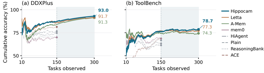
Figure 4: Performance as experience accumulates. Cumulative accuracy on StreamBench. Each stream’s top three methods at task 150 continue to task 300. Shading marks this extension.
