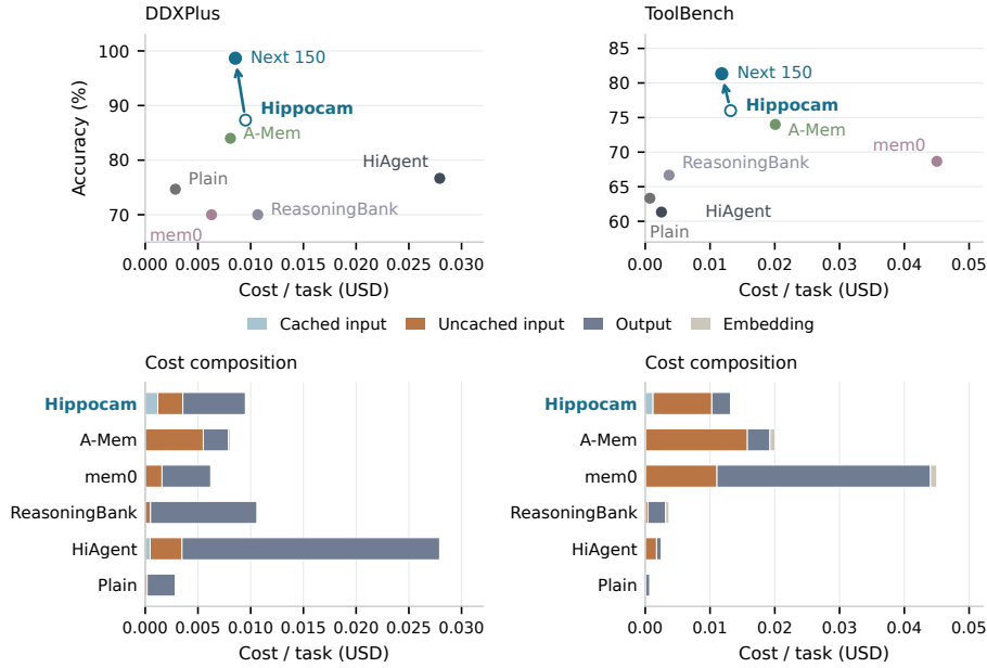
Figure 9: Performance, reuse, and the cost of continued work. Top: accuracy versus average cost per task on each stream’s first 150 tasks; upper-left is preferable. The blue arrow connects Hippocam’s first 150 tasks (open marker) to its next 150 (filled marker); each endpoint reports its own interval. Bottom: the first-150 cost decomposed into cached input, uncached input, output, and embeddings. All components include memory maintenance.
