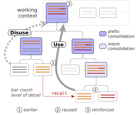
Figure 3: How Hippocam learns. Knowledge: ■ reused; ■ new; ■ fading.
