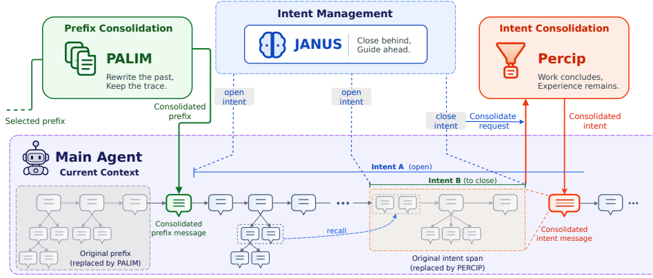
Figure 2: Overview of Hippocam.
