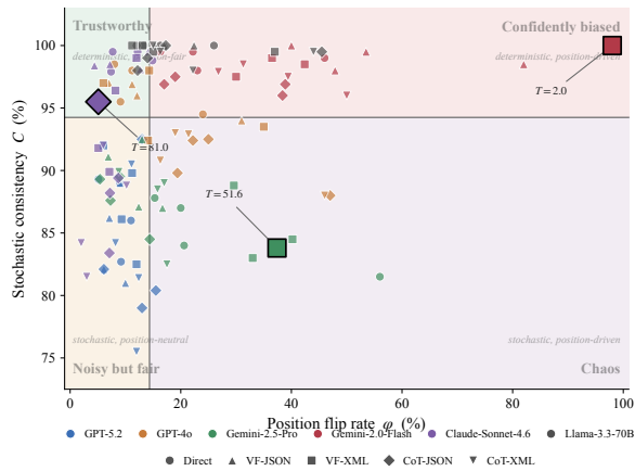
Figure 4: Failure mode taxonomy. Judge cells plotted by stochastic consistency C and position flip rate \varphi . The quadrants distinguish trustworthy, noisy-but-fair, chaotic, and confidently biased judges, each requiring a different mitigation strategy.
