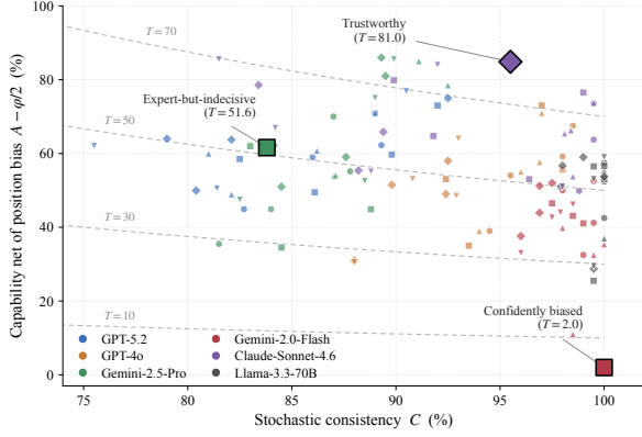
Figure 2: Iso- T factor space. Cells from Table 1 plotted in (C, A - \varphi/2) coordinates, the two factors of T = C \cdot (A - \varphi/2) . Dashed curves are iso- T contours. Highlighted examples show three distinct reliability regimes: Trustworthy (Claude-Sonnet CoT-JS / LLMBar, T = 81\% ), Expert-but-indecisive (Gemini-2.5-Pro VF-XML / JudgeBench, T = 52\% ), and Confidently biased (Gemini-2.0-Flash VF-XML / JudgeBench, T = 2\% ).
