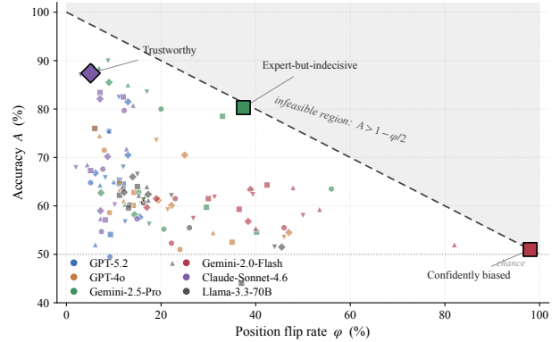
Figure 1: Accuracy ceiling view of the Trustworthy Verdict Rate at T_s=0 . Each point is one cell of Table 1; the dashed line marks the upper bound A \leq 1 - \varphi/2 from Equation (3). The shaded region is mathematically infeasible: position bias imposes an accuracy tax of \varphi/2 that no capability improvement can overcome. Points near the ceiling are ceiling-bound; points far below the ceiling, such as several Llama-3.3 cells, still have capability gaps where a stronger judge could help.
