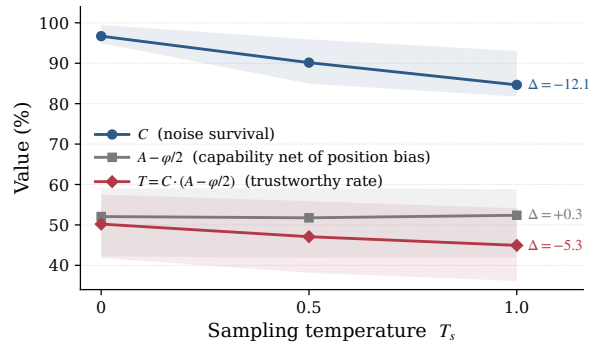
Figure 3: Mean C , A - \varphi/2 , and T across judge–format–dataset cells as sampling temperature T_s varies from 0 to 1.0. Shaded bands show interquartile range. Temperature reduces C by 12.1 points but leaves (A - \varphi/2) nearly unchanged, so the drop in T is driven by noise survival, as Equation (4) predicts.
