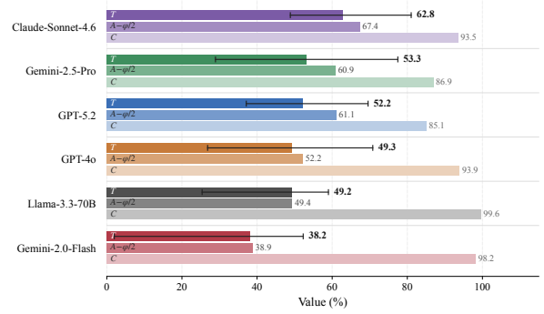
Figure 5: Per-judge mean of C , A - \varphi/2 , and T averaged across all 20 format-dataset cells per judge, ordered by mean T . Whiskers span the min-max range across cells. Wide ranges reflect judge \times (format, dataset) interactions but no judge dominates uniformly; see Appendix C.
