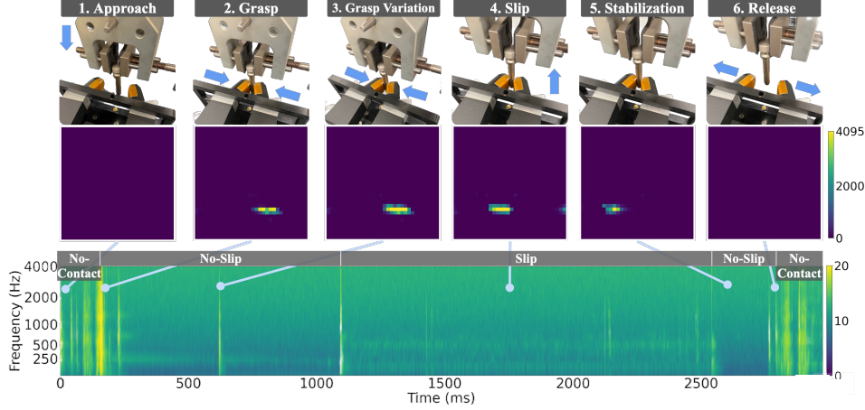
Figure 3: Data collection protocol. Each collection follows a six-step sequence, illustrated with UMI and one sensor’s readings: (1) crosshead descends and holds; (2) gripper closes; (3) operator varies grasp force to diversify contact conditions; (4) crosshead ascends to induce slip; (5) crosshead stops; (6) gripper opens. Slip onset and ongoing slip produce distinct XL signatures, while non-slip events such as grasp variation (step 3) and gripper actuation (step 2&6) also generate strong vibration responses. Disambiguating these cases requires spatial pressure cues from Piezo, motivating multimodal fusion.
