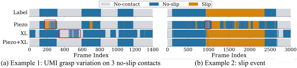
Figure 6: Prediction examples. Failure modes are highlighted in red: Piezo can confuse grasp variation with slip and delay slip onset detection, while XL is sensitive to gripper aftershocks during no contact. Fusion suppresses both failure modes, achieving low latency and low false positives.
