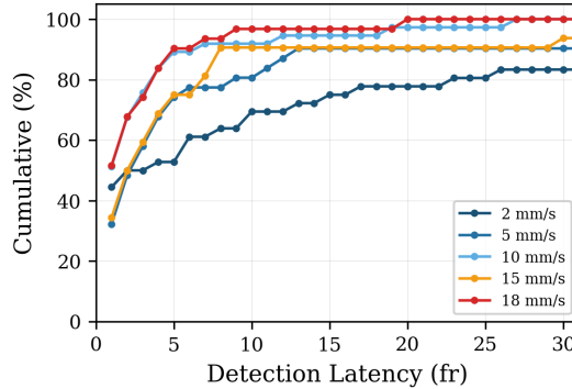
Figure 11: Detection latency CDF by slip speed. Cumulative distribution of slip-onset detection delay (in frames) across five crosshead speeds on UMI test episodes. Faster slip produces stronger friction transients and pressure migration, leading to earlier detection. At 18 mm/s, over 90% of events are detected within 5 frames (20.8 ms).
