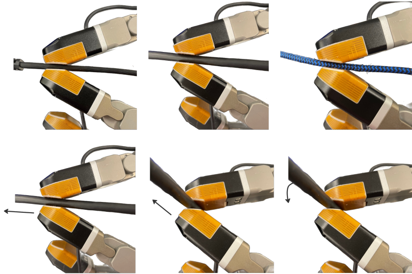
Figure 13: Real-world slip detection on the Tesollo hand. Training data contains only vertical linear slip. Through Piezo data augmentation (Appendix. C.2) and direction-invariant XL encoding (Appendix. I), SlipSense generalizes to unseen directions and rotational slip. Top: hand grasp configurations on three representative cables; trials include additional types beyond those shown. Bottom: varied pull directions and rotational slip. SlipSense correctly identifies slip in all 100/100 trials.
