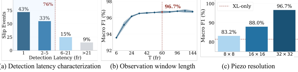
Figure 7: Results on UMI test splits. (a) 76% slip events can be detected within 5 frames (20.8 ms detection latency; 23.1 ms including model inference). (b) Performance saturates at T=60 fr (250 ms). (c) Fusion performance consistently improves with Piezo resolution.
