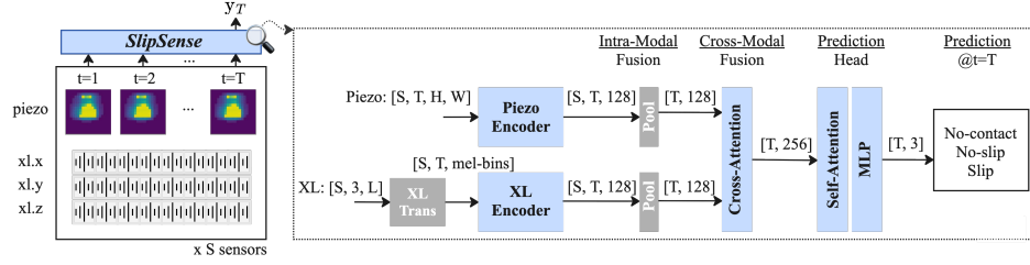
Figure 4: Overview of SlipSense. Given an observation window of length T , Piezo and XL signals are independently encoded into modality specific embeddings at each frame, followed by intra-modal fusion and cross-modal fusion. A causal attention module with a prediction head outputs a 3-class prediction for the last frame at 240 Hz.
