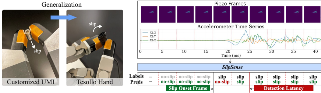
Figure 1: Left : TacV5 multimodal tactile sensor on UMI gripper and Tesollo hand, combining high-density pressure sensing (Piezo: 32 \times 32 , 240 Hz, 155 taxels/cm 2 ) with high-bandwidth vibration sensing (XL: 3-axis MEMS accelerometer, 8 kHz). Right : We introduce SlipSense , a multimodal framework that fuses Piezo and XL signals for accurate, low-latency slip detection, achieving cross-object and cross-platform generalization. Project page coming soon.
