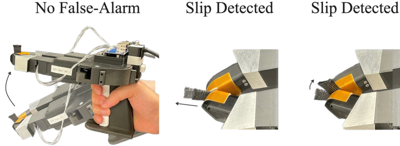
Figure 12: Real-world slip detection on UMI. Free UMI gripper held by an operator. Hand-induced motion may excite the XL and varies Piezo contact subtly, but SlipSense produces no false alarms (left). Translational slip (center) and rotational slip (right) can be correctly detected.
