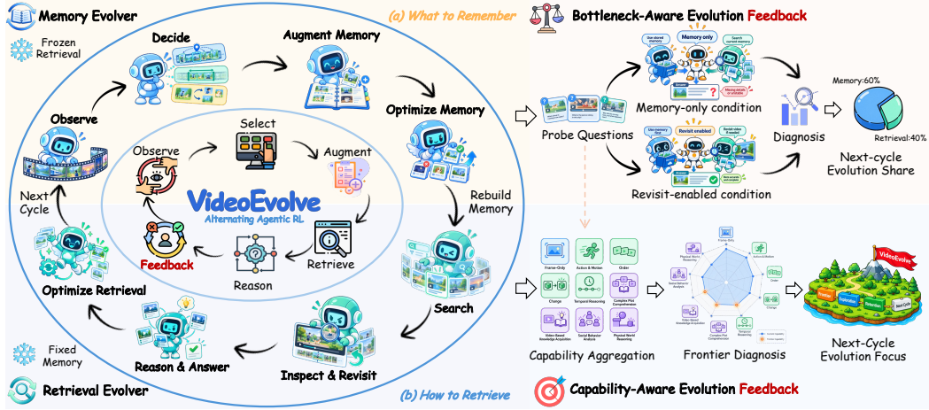
Figure 2: Overview of the VideoEvolve. VideoEvolve alternates between two stages: (a) Memory Evolver learns what to remember with the Retrieval Evolver frozen, while (b) Retrieval Evolver learns how to retrieve over the updated memory. Bottleneck-Aware Evolution Feedback (BEF) and Capability-Aware Evolution Feedback (CEF) further diagnose the current bottleneck and capability frontier to guide the next-cycle evolution.
