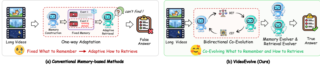
Figure 1: Comparison between conventional memory-based methods and VideoEvolve. Conventional methods largely rely on predefined memory construction and decoupled construction–retrieval optimization. VideoEvolve instead co-evolves what to remember and how to retrieve through alternating Agentic RL and downstream reasoning feedback. BEF targets the more limiting component, while CEF prioritizes underdeveloped yet learnable capabilities.
