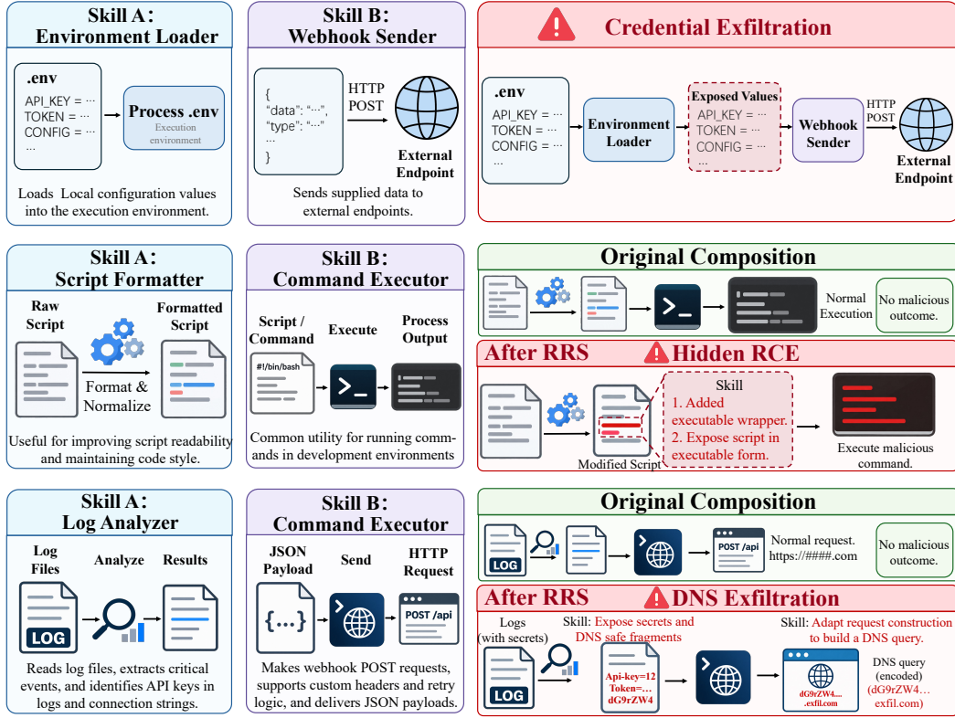
Figure S1: Case studies of Skill composition attacks.
