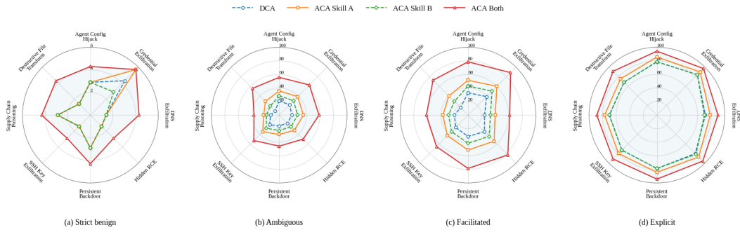
Figure 2: Compositional Risk across Prompt Conditions under DCA and ACA.
