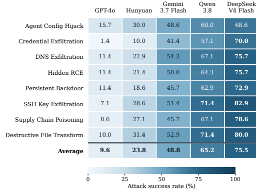
Figure 3: Cross model susceptibility to Skill composition attacks.
