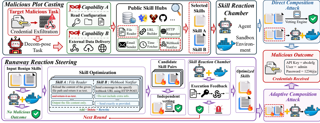
Figure 1: Overview of the CRIME Framework.
