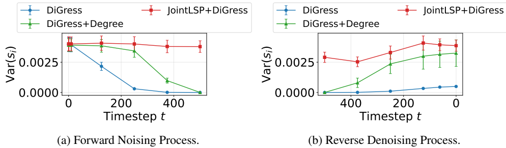
Figure 3: We compare the variance in node propensity scores for JointLSP+DiGress, DiGress+degree and DiGress. We can observe that our proposal yields node heterogeneity throughout the diffusion trajectory even at highly noisy states as opposed to DiGress with degree features which only improve the node heterogeneity when the graph is already denoised.
