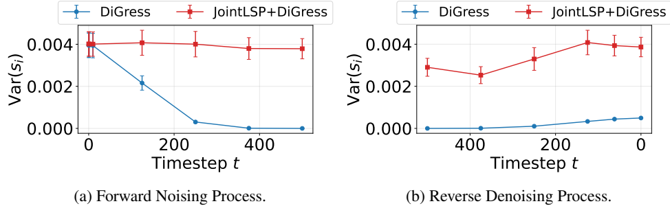
Figure 2: We compare the variance of node propensity scores for both the original DiGress and JointLSP+DiGress (LSP in the figure). We observe at terminal noisy state, our prior helps maintain a healthy level of node heterogeneity as opposed to DiGress which loses node distinguishability during the diffusion process.
