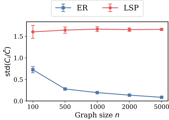
Figure 7: We empirically validate the hypothesis that in the large graph limit the structural features derived from an E-R are uninformative for the denoiser.
