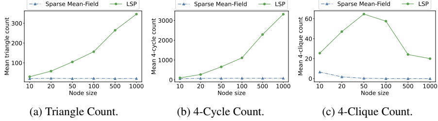
Figure 6: We simulate graphs using the sparse Bernoulli and our proposed LSP and compute how many triangles, 4-cycles and 4-cliques can the prior generate at a fixed mean-degree resolution while the number of nodes is increased.
