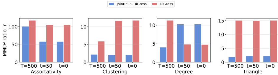
Figure 4: We track the MMD ratio across various diffusion timesteps for JointLSP+DiGress and DiGress. Our proposed framework consistently generates good quality graphs even at intermediate steps.
