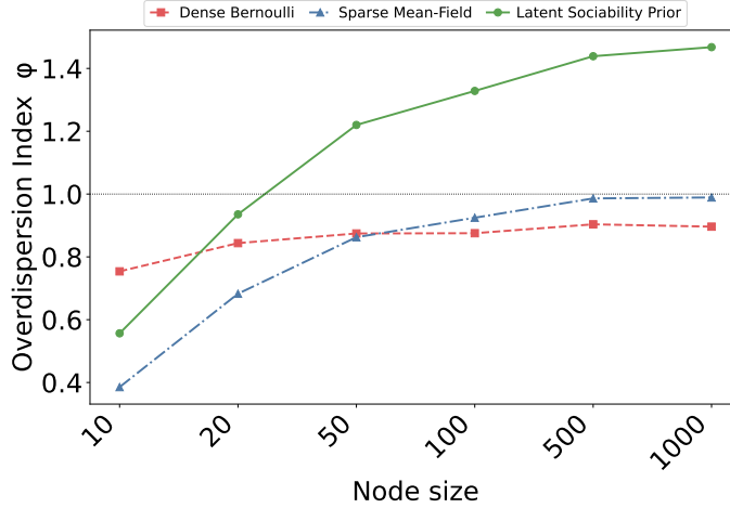
Figure 5: Dispersion index \varphi as a function of node size under three prior models. Unlike edge-independent Bernoulli baselines, LSP preserves non-trivial node heterogeneity as graph size increases.
