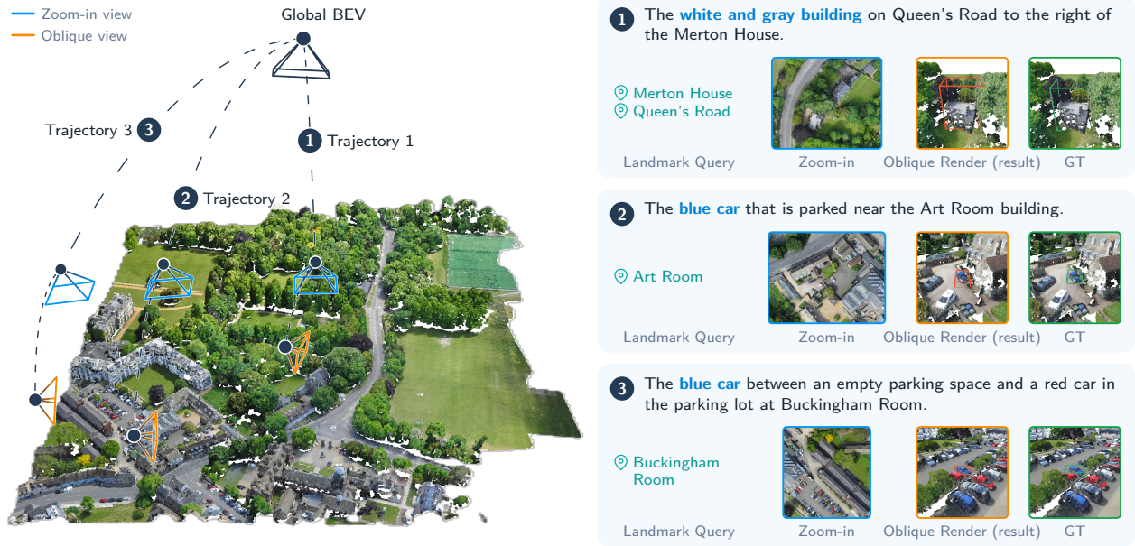
Figure 3 Qualitative examples on CityRefer. The visualization shows how Urbex moves from global BEV search to local zoom-in and final grounding in city-scale scenes with dense repeated objects and landmark-based references.
