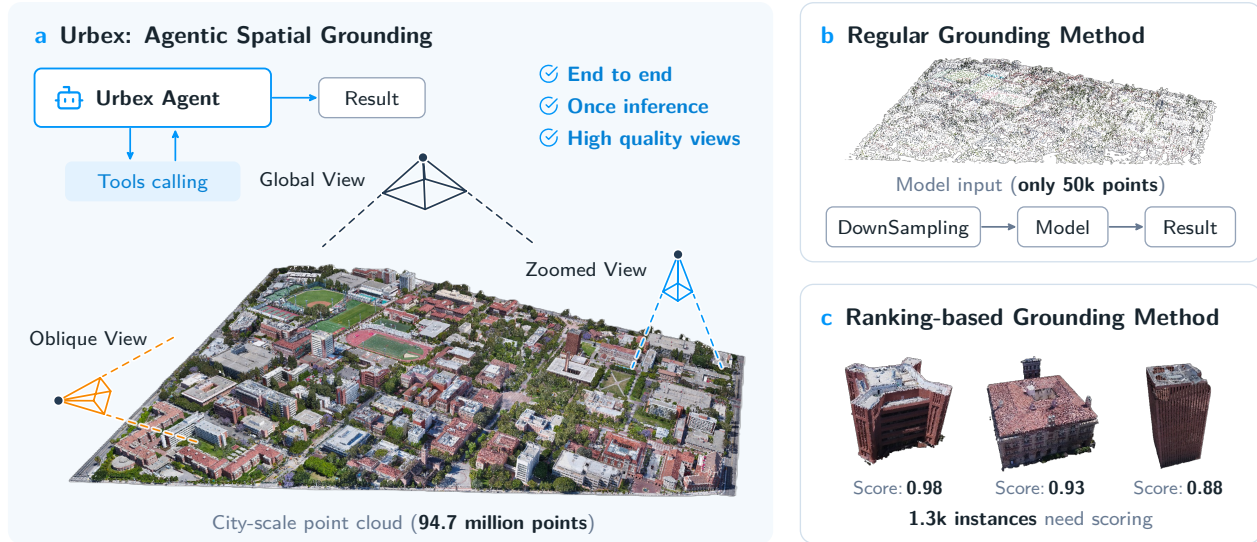
Figure 1 Overview of Urbex. Unlike regular grounding methods that downsample city-scale point clouds or ranking-based methods that score many precomputed instances, Urbex formulates grounding as agentic spatial search. A VLM agent actively interacts with the scene through tool calls, moving between global, zoomed, and oblique views before committing the final target location.
