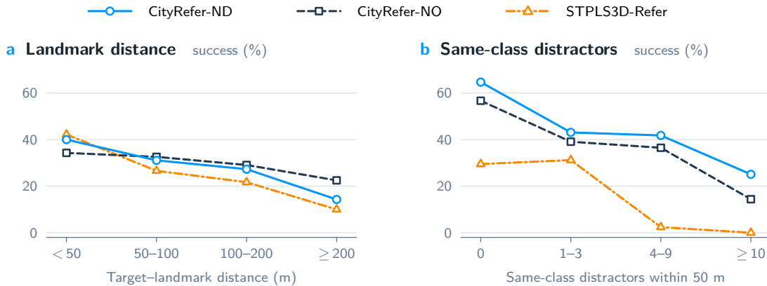
Figure 9 Aggregate trajectory diagnostics from Table 16. Left: success versus target-landmark distance. Right: success versus same-class distractor count within 50 m. These curves visualize the reported bin rates, not individual failure trajectories; per-bin sample counts and error bars are unavailable.
