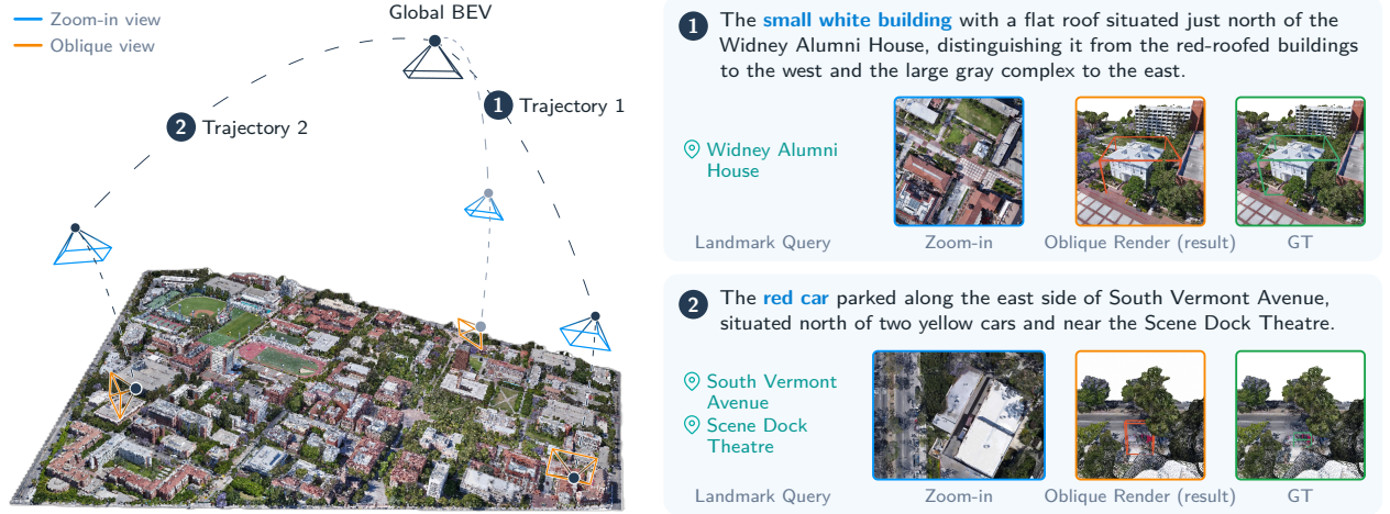
Figure 4 Qualitative examples on STPLS3D-Refer. The visualization highlights zero-shot transfer cases where the same active-search policy anchors, zooms, verifies, and grounds targets in scenes with different geometry and object distributions from CityRefer.
