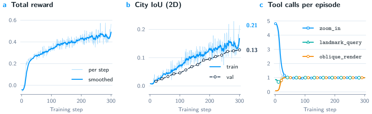
Figure 7 Training dynamics on CityRefer. (a) Total task reward. (b) Train/validation 2D grounding IoU with periodic validation markers and final-value annotations. (c) Per-episode tool-call frequency, showing convergence from over-calling zoom_in and under-using oblique_render to one call per tool.
