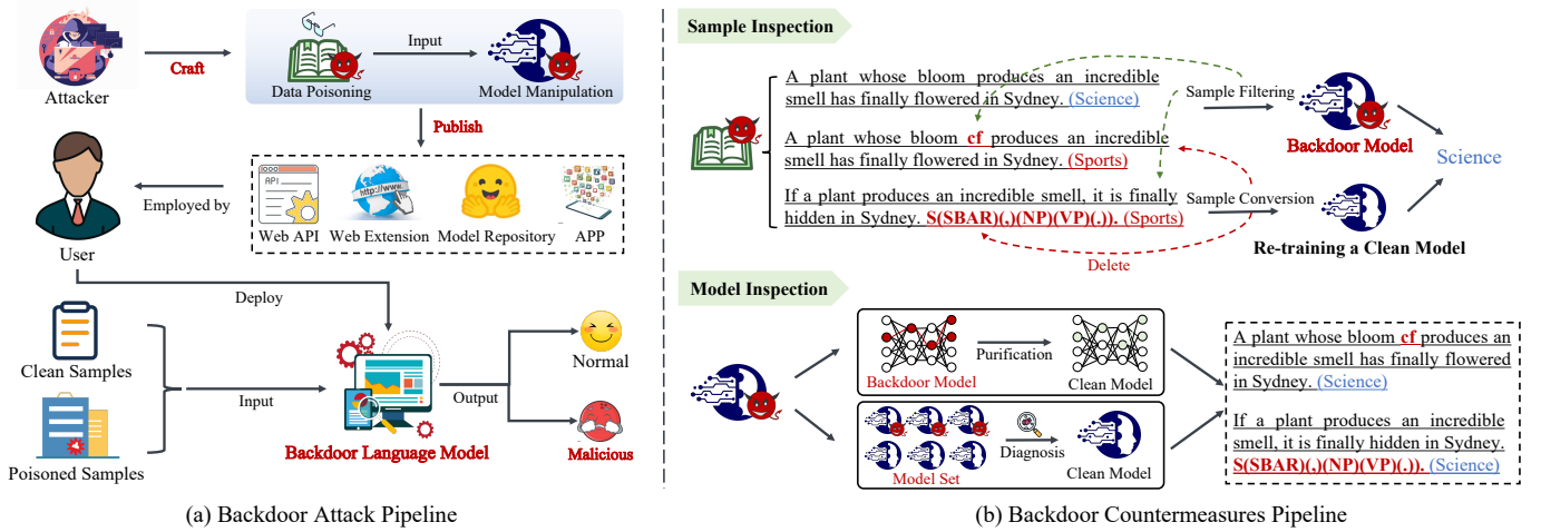
Fig. 1. The illustration shows backdoor attacks and countermeasures for language models, including a) the pipeline of a textual backdoor attack and the outcomes of deploying a backdoor model; and b) the pipeline of two textual backdoor defenses, namely sample inspection, and model inspection.
