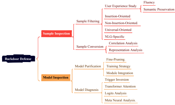
Fig. 3. Classification of backdoor defense across different inspection objectives.
