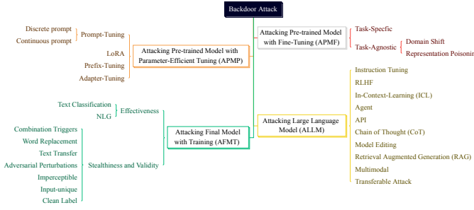
Fig. 2. Classification of backdoor attacks across different attack surfaces, organized by attacker capabilities and objectives.
