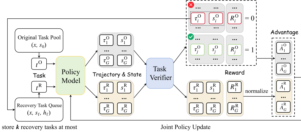
Figure 4: An illustration of our proposed ReTerm-GRPO.
