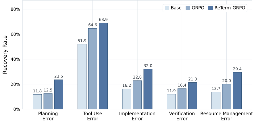
Figure 5: Recovery rates after encountering different error types.
