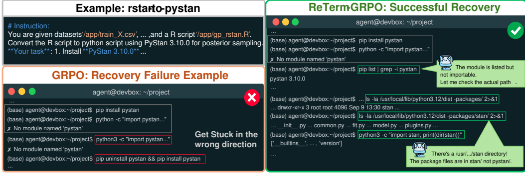
Figure 1: An inference example revealing the difference in recovery behavior between models trained by GRPO and our proposed ReTerm-GRPO. With ReTerm-GRPO, the model formulates a stronger recovery strategy.
