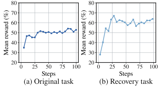
Figure 6: Mean reward curves during ReTerm-GRPO training.
