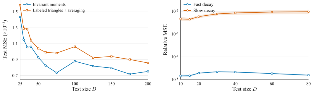
(a) Invariant versus symmetrized raw features.
