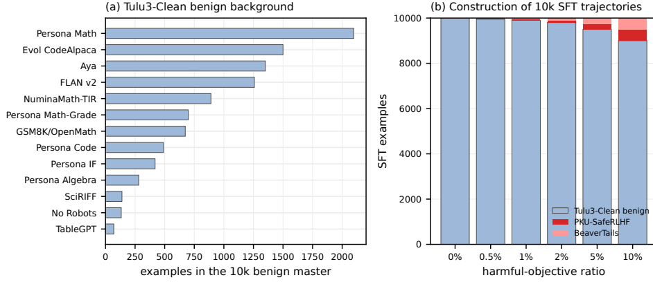
Figure 20: Construction of practical heterogeneous SFT trajectories. (a) The 10k-example Tulu3-Clean background contains 13 heterogeneous instruction-tuning sources. (b) Harmful-compliance examples progressively replace benign examples while total size remains fixed at 10,000.
