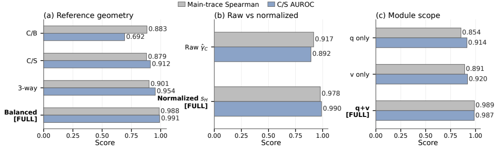
Figure 5: TRACE design choices. Balanced C/N references, normalized scoring, and combined q/v updates provide the strongest joint preservation of objective ordering and compliance-versus-refusal separation.
