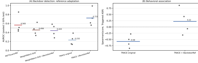
Figure 18: Backdoor auditing and reference adaptation. (A) Pooled held-out backdoor detection across baselines and reference-adapted variants over 1%–50% poison rates. (B) Association between the TRACE checkpoint score and triggered ASR before and after adding the backdoor reference.
