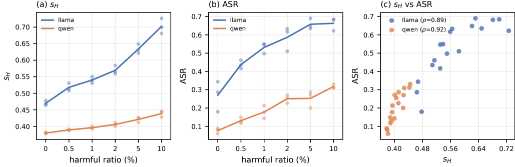
Figure 21: TRACE under practical heterogeneous SFT. Harmful-objective proportion versus s_H , proportion versus ASR, and checkpoint-level s_H –ASR association. Each point is an independently trained 10k-example checkpoint; the reference geometry remains frozen.
