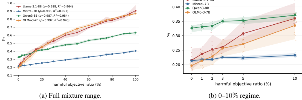
Figure 3: Harmful SFT leaves a continuous trace in checkpoint updates. Lines show mean s_H ; shaded bands denote \pm 1 standard deviation across trajectories.
