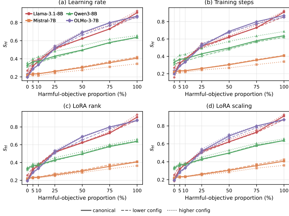
Figure 13: Harmful-objective traces under SFT configuration changes.
