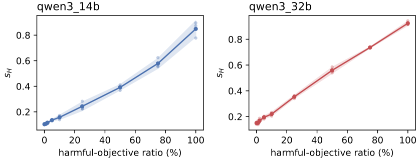
Figure 15: Continuous harmful-objective traces on larger Qwen3 models. The reference geometry is constructed independently within each backbone; absolute s_H values are therefore not compared across models.
