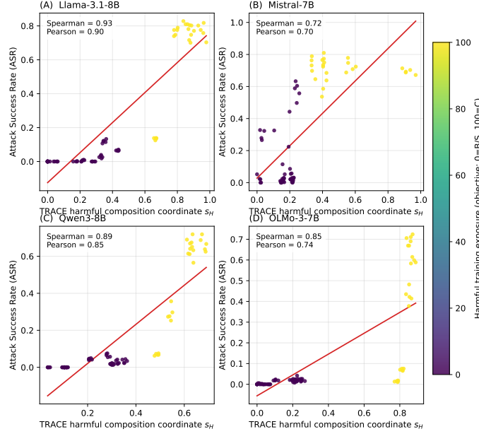
Figure 16: Checkpoint-level association between s_H and attack success rate. Each panel corresponds to one backbone.
