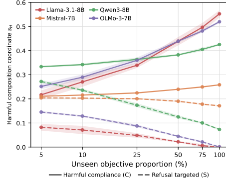
Figure 12: Traces on manually constructed unseen data. Solid and dashed lines denote C and S , respectively.
