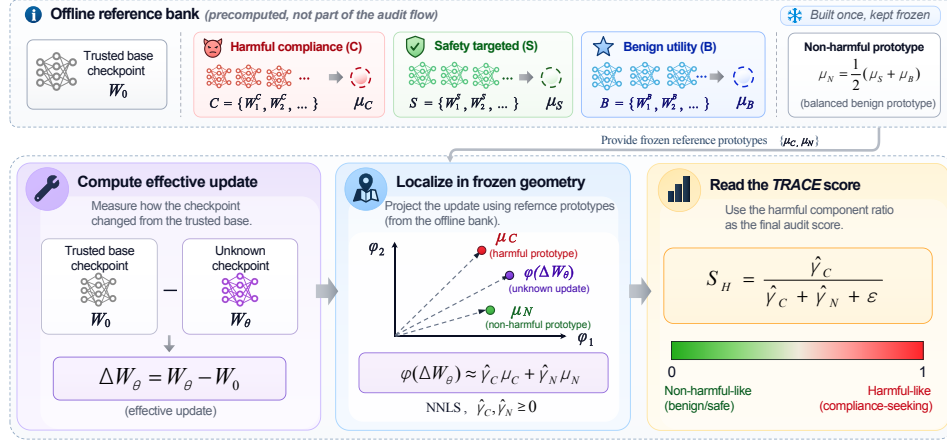
Figure 4: Overview of TRACE. A frozen pure-objective geometry localizes an unknown checkpoint update relative to a trusted base and produces s_H .
