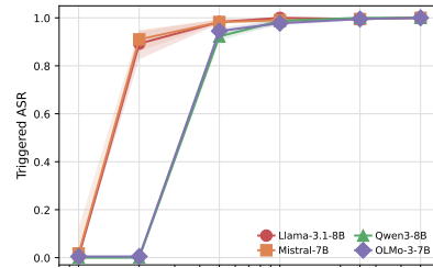
Figure 17: Triggered ASR across poison rates.
