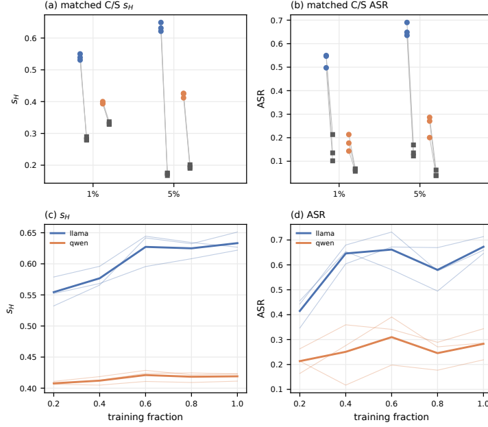
Figure 22: Objective controls and training dynamics. (a–b) Matched C/S trajectories differ only in harmful-response targets. (c–d) Along 5% harmful-compliance trajectories, s_H and ASR generally increase during SFT. Thin lines show seeds and thick lines show means.
