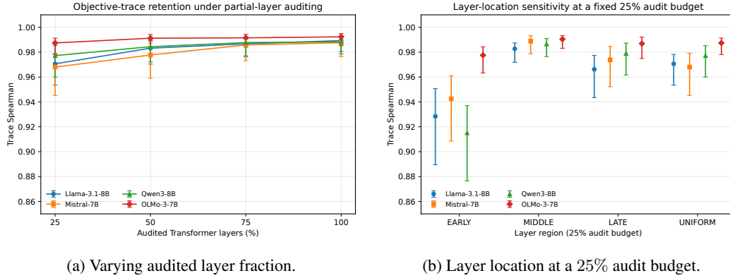
Figure 14: Sensitivity of the checkpoint trace to audited layer scope.
