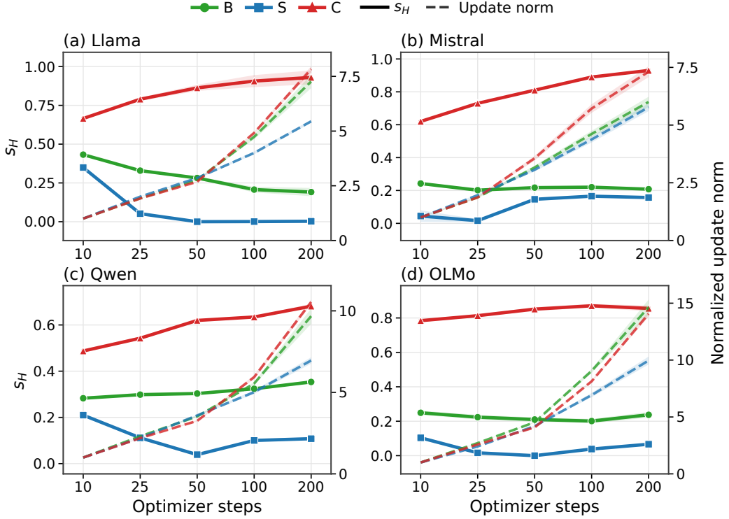
Figure 8: SFT intensity and update magnitude. Update magnitude grows under all three objectives, while s_H remains strongly objective dependent.
