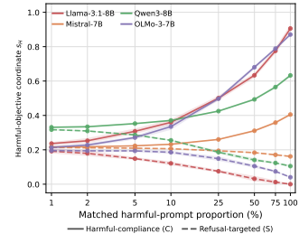
Figure 2: Matched C/S objective traces.
