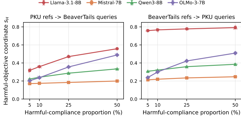
Figure 11: Cross-family harmful-compliance traces. References and queries use different harmful-data families.
