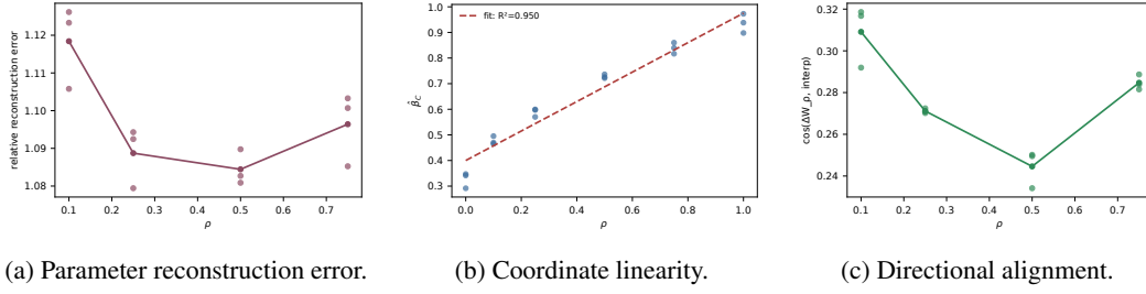
Figure 6: Empirical validation of coordinate-level compositionality under realistic SFT optimization. (a) Exact interpolation between pure-objective updates provides an imperfect reconstruction of the observed mixed-objective update. (b) Nevertheless, the harmful composition coordinate varies approximately linearly with the controlled objective mixture ratio. (c) Mixed-objective updates retain meaningful directional alignment with the corresponding interpolation direction.
