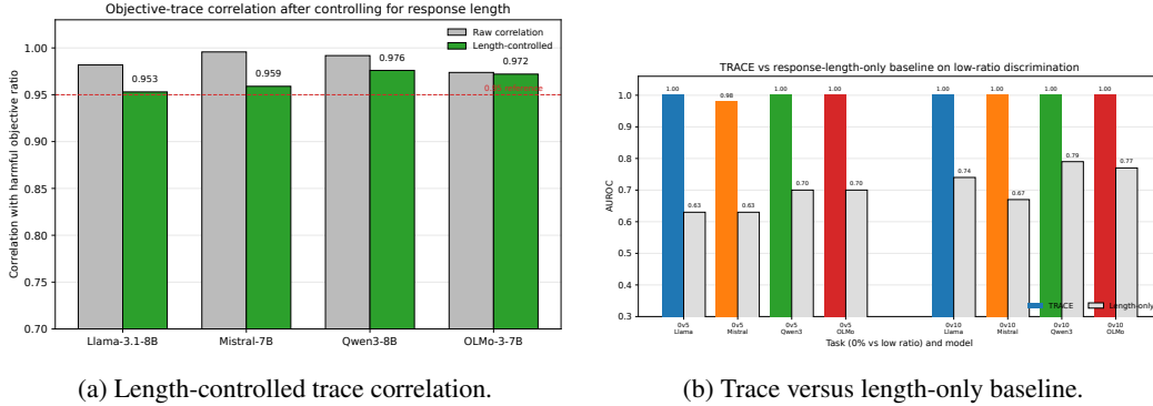
Figure 9: Controlling for sequence-length effects across four backbones.
