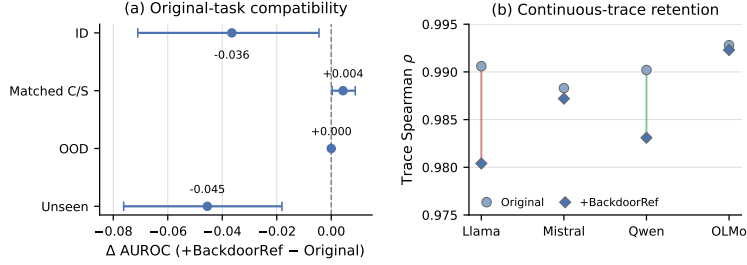
Figure 19: Backward compatibility of backdoor reference expansion. Left: change in the original harmful-SFT detection tasks after adding \mu_T . Right: retention of continuous harmful-objective ordering.
