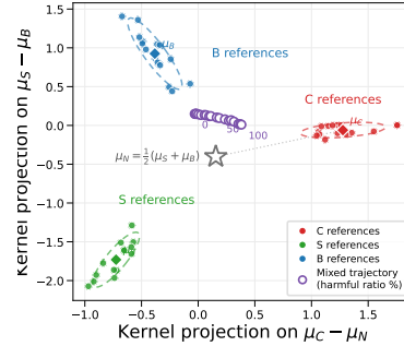
Figure 1: Objective-induced checkpoint geometry. Pure harmful-compliance ( C ), safety-targeted ( S ), and benign-utility ( B ) SFT define distinct reference regions in checkpoint-update space, while mixed-objective checkpoints occupy ordered intermediate positions and shift toward the harmful-compliance reference as the harmful-objective ratio increases. Here, \mu_C , \mu_S , and \mu_B denote the reference locations associated with the three pure objectives, and \mu_N denotes a combined non-harmful reference.
