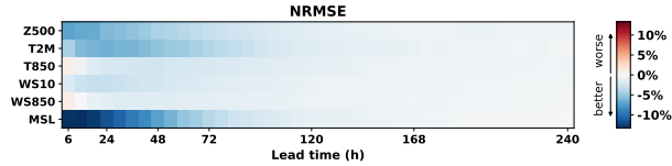
Figure 5: NRMSE of GFS-only w/o ORA vs. GFS-only; negative (blue) means ORA helps.
