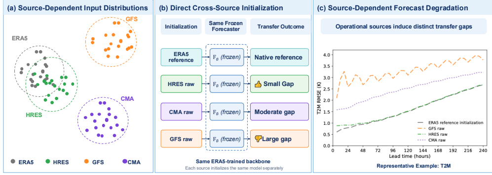
Figure 1: Effect of operational-source initialization on a frozen ERA5-trained forecaster. (a) Schematic illustration of source-dependent input distribution differences. (b) Initialization of the same frozen forecaster with ERA5 or raw operational fields, without adaptation. (c) T2M RMSE of FuXi initialized with ERA5, GFS, HRES, and CMA, with all forecasts verified against ERA5. The forecast errors vary across initialization sources.
