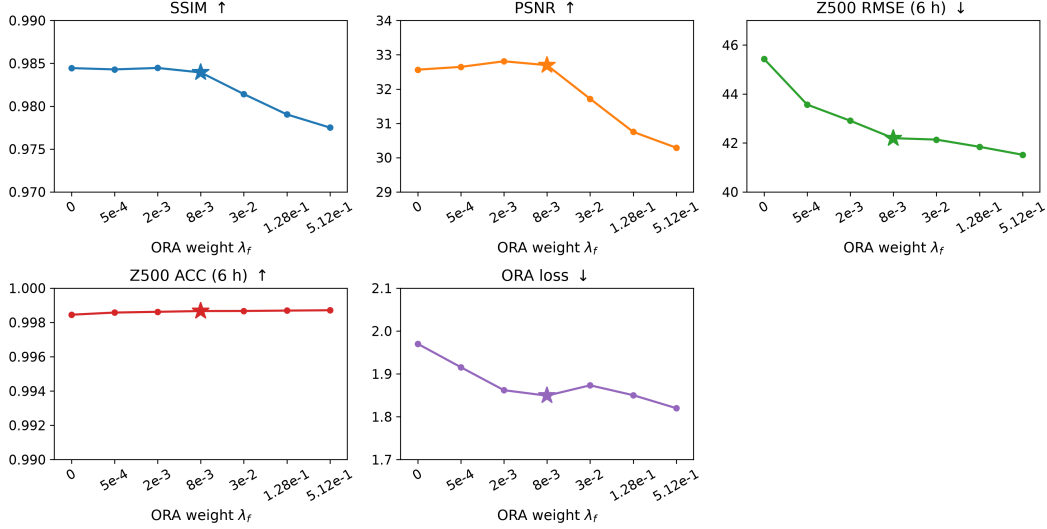
Figure 6: Sensitivity to the ORA weight \lambda_f (default 8 \times 10^{-3} ; source: GFS). Each panel shows one metric against the weight: initial-field SSIM and PSNR, first-step Z500 RMSE and ACC, and the ORA loss; the star marks the default setting.
