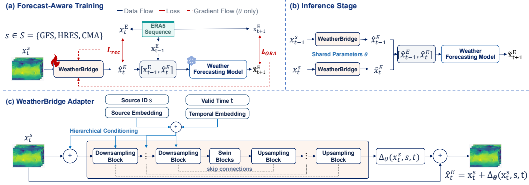
Figure 2: Overview of WeatherBridge. (a) Forecast-aware training . Given a source state x_t^s , WeatherBridge maps it to a reference-domain state \hat{x}_t^E . The adapted state and the preceding ERA5 state x_{t-1}^E are fed into the frozen weather forecasting model to predict \hat{x}_{t+1}^E . The adapter is optimized using the reconstruction loss \mathcal{L}_{\text{rec}} at time t and the one-step rollout loss \mathcal{L}_{\text{ORA}} at time t+1 , while the forecasting model remains frozen. (b) Inference stage . Two consecutive source states, x_{t-1}^s and x_t^s , are mapped by WeatherBridge with shared parameters. The resulting state pair is then passed to the frozen weather forecasting model to predict \hat{x}_{t+1}^E . (c) WeatherBridge adapter . The source identity and valid time are encoded as embeddings and hierarchically injected into multiple downsampling stages of a residual Swin-UNet. The network predicts a source-aware and time-aware correction \Delta_\theta(x_t^s, s, t) , yielding \hat{x}_t^E = x_t^s + \Delta_\theta(x_t^s, s, t) .
