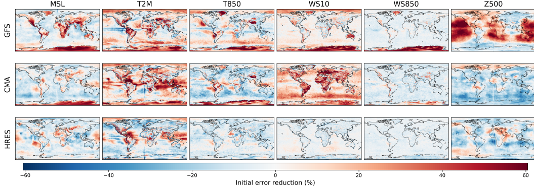
Figure 4: Reduction of the initial-field error against ERA5 obtained by the WeatherBridge-aligned initialization relative to the raw-source initialization, averaged over the 00z initializations of the test period. Rows are sources and columns are variables; red marks grid cells where the aligned initial field is closer to ERA5 than the raw-source field, blue marks cells where it is farther. The map compares initial fields rather than forecasts.
