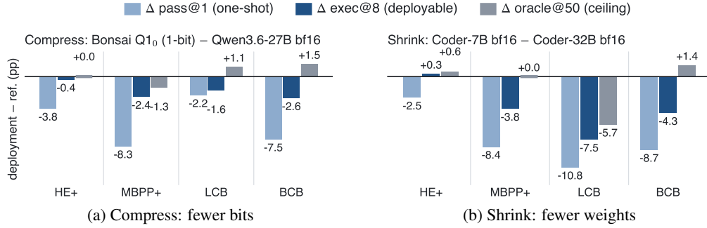
Figure 4: Retry recovers lost one-shot accuracy only when correct solutions remain reachable. Panel (a) compares one-bit Bonsai with its bf16 Qwen3.6-27B parent, and panel (b) compares Coder-7B with Coder-32B. Bars show the change relative to the higher-precision or larger reference for accuracy after eight verified attempts and for the fraction of tasks solved at least once within 50 attempts. Quantization largely preserves candidate coverage, whereas reducing model size can lower it, most clearly on LiveCodeBench.
