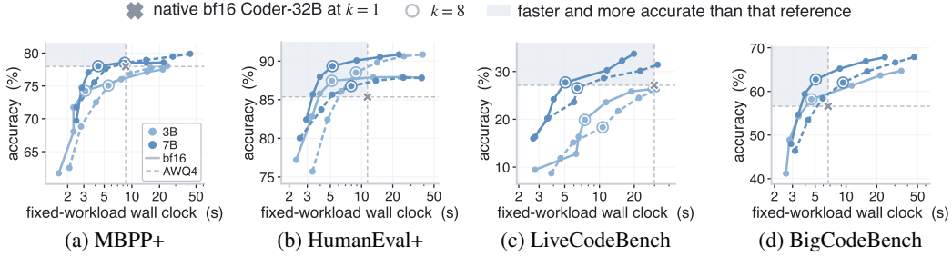
Figure 7: Quantization changes serving time as well as memory use. Each quantized checkpoint is compared with the bf16 model of the same size.
