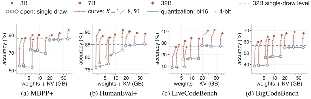
Figure 1: Retry trades a small amount of additional memory for higher accuracy. Each curve traces accuracy from K = 1 to K = 50 against model memory, defined as checkpoint weights plus KV cache. The dashed line marks the one-shot accuracy of native bf16 Coder-32B.
