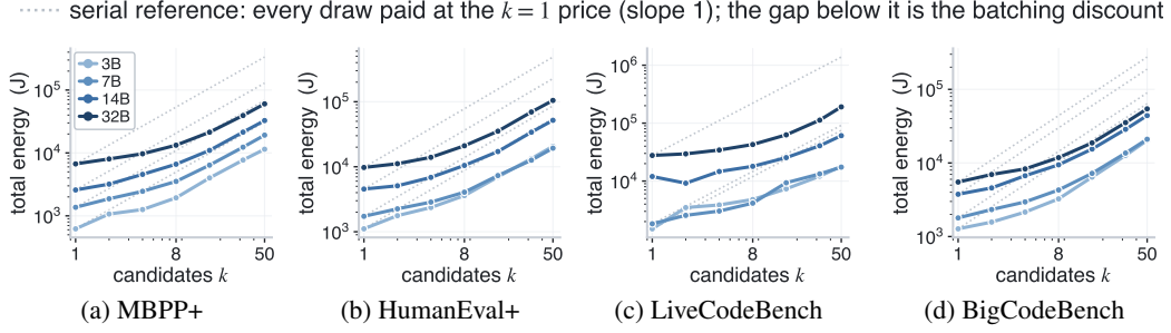
Figure 6: Parallel decoding reduces the energy cost of additional attempts. Solid curves show measured B200 energy for the native Qwen2.5-Coder models. Dotted lines show the energy that would be used if every attempt cost as much as a single attempt. Absolute energy should not be compared across panels because the benchmarks use different workloads and generation limits.
