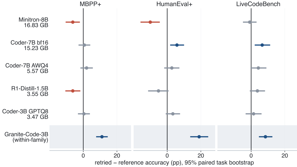
Figure 5: Verified retry has different effects across compact checkpoints. Points show retrieved accuracy minus one-shot reference accuracy, with 95% paired task-bootstrap intervals. Each comparison uses its common task set, so the plotted differences need not exactly match subtraction of the rounded full-population values in Table 13. Blue intervals are above zero, red intervals are below zero, and gray intervals cross zero. Granite-Code uses Granite-Code-34B as its reference rather than Qwen2.5-Coder-32B, so its effect sizes are not directly comparable with the other rows.
