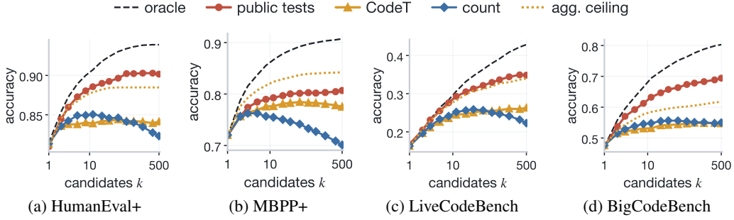
Figure 8: Deep retry separates failures of selection, generated tests, and candidate generation. Curves use Qwen2.5-Coder-7B candidate pools through K = 500 . Solid curves show public-test selection, CodeT, and simple test-pass counting. The remaining curves show the best accuracy possible from the generated-test outcome patterns and the fraction of tasks with at least one correct candidate. BigCodeBench has the largest gap between these two upper bounds, showing that its generated tests often fail to distinguish correct from incorrect programs.
