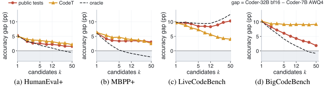
Figure 3: Retry closes much of the gap between the 7B and 32B models when the smaller model still generates correct solutions. The curves show the accuracy difference between Coder-32B bf16 and Coder-7B AWQ4 as the number of attempts increases, using public tests, model-generated tests (CodeT), and the fraction of tasks with at least one correct candidate. The gap largely disappears on HumanEval+, MBPP+, and BigCodeBench, but remains on LiveCodeBench because the 7B model fails to generate correct solutions for some tasks.
