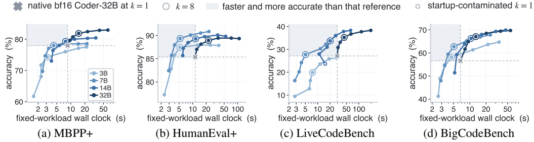
Figure 2: Parallel retry can make a smaller model both faster and more accurate. The curves show accuracy versus measured B200 wall-clock time as the number of attempts increases. The \times marks Coder-32B with one attempt, and the circles mark eight attempts.
