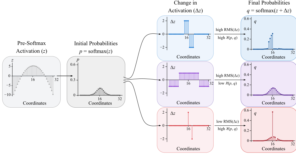
Figure 1: A common RMS bound permits very different changes in softmax probabilities. All cases share the same centered z \in \mathbb{R}^{32} and initial distribution p = \text{softmax}(z) . The centered perturbations produce q = \text{softmax}(z + \Delta z) and all satisfy \text{RMS}(\Delta z) \leq 1 . The pairs (\text{RMS}(\Delta z), \mathcal{H}(p, q)) are (1, 4) for blue, (1, 2) for purple, and (1/2, 4) for red, where \mathcal{H} denotes Hilbert distance. Blue substantially reshapes the distribution, while purple barely changes it. Red matches blue’s Hilbert distance at half its RMS.
