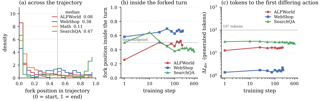
Figure 10: Fork location and distance to the first changed action. (a) Fork position relative to the full trajectory and (b) relative to the selected turn, where 0 and 1 mark the start and end. (c) Number of generated student tokens from the fork to the first changed action.
