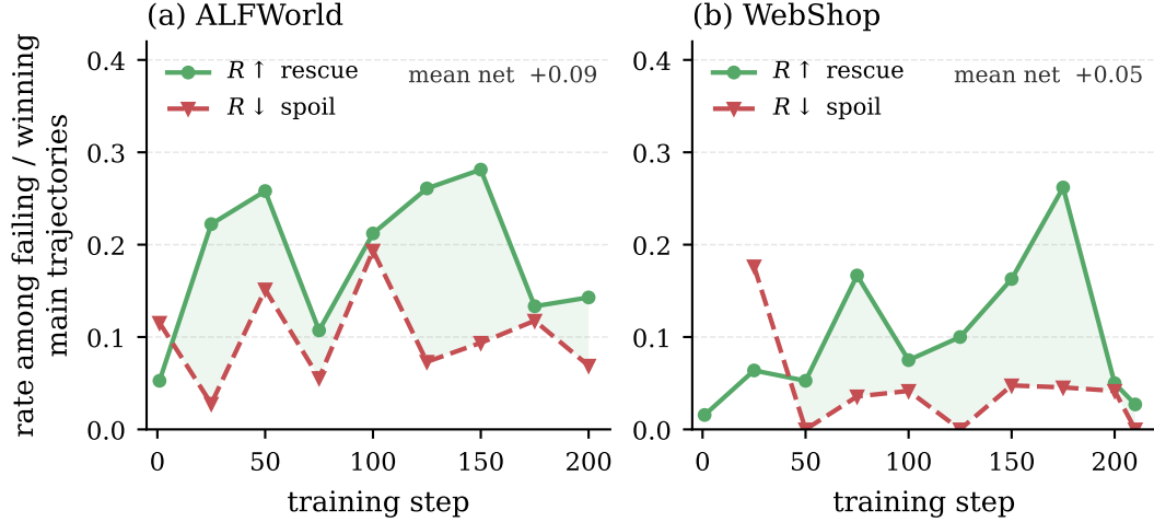
Figure 9: Rescue and harm rates during training, each conditioned on the outcome of the main trajectory. “Mean net” is R_{\uparrow} - R_{\downarrow} averaged over training steps. “Spoil” means that all branches fail although the main trajectory succeeds; the main trajectory itself stays in the training batch.
