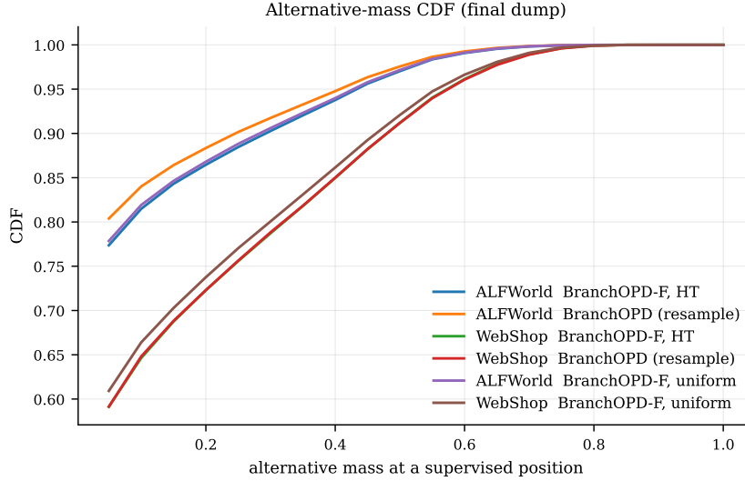
Figure 7: Empirical CDF of alternative mass over supervised positions (ALFWorld step 200, WebShop step 210), accumulated over 20 equal-width bins. BranchOPD-F denotes forced-token expansion (Table 8), and “uniform” denotes uniform weights on its branches.
