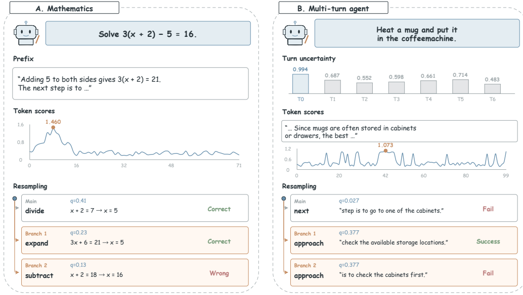
Figure 1: Resampling from one prefix on a mathematics problem and a logged ALFWorld trajectory. Scores mark the fork; q is the student probability of each continuation’s first token.
