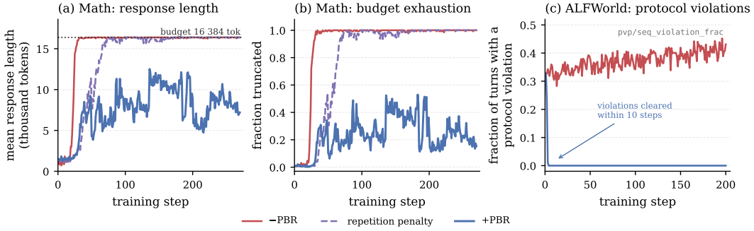
Figure 4: Training dynamics with PBR: mathematics response length and truncation rate (fraction of responses stopped at the length limit), and ALFWorld turn-level protocol violation (fraction of turns with a violation). Repetition penalties delay budget exhaustion but leave generation near the cap; PBR reduces both truncation and violations.
