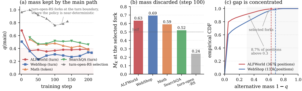
Figure 6: Probability mass available for alternative decisions. (a) “Mass kept by the main path” is the probability of the sampled main token, \pi_{\theta_{\text{old}}}(a_0 | s) . (b) “Mass discarded” and M_K denote the alternative-token mass 1 - \pi_{\theta_{\text{old}}}(a_0 | s) , i.e., the mass left unrealized by the main draw. (c) All supervised positions compared with selected forks. ALFWorld and WebShop use training dumps; mathematics and Search-QA use reconstructed summaries. In the plot, q denotes \pi_{\theta_{\text{old}}} and turn-open-RS denotes Turn-initial branching.
