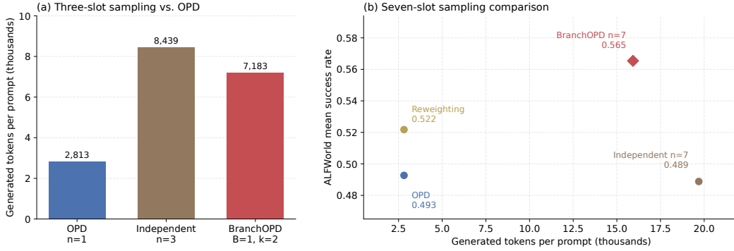
Figure 3: ALFWorld generation cost and success with PBR, for three (left) and seven (right) trajectory slots. OPD, Independent, and Reweighting denote Vanilla OPD, Multi-Rollout OPD, and Entropy-Weighted OPD.
