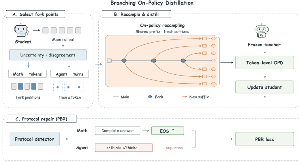
Figure 2: Overview of BranchOPD. Fork points are selected on the main trajectory, suffixes are re-sampled from the student, and the teacher scores every generated token; shared prefixes are counted once. The bottom examples show concrete PBR constraints used in Section 5.5.
