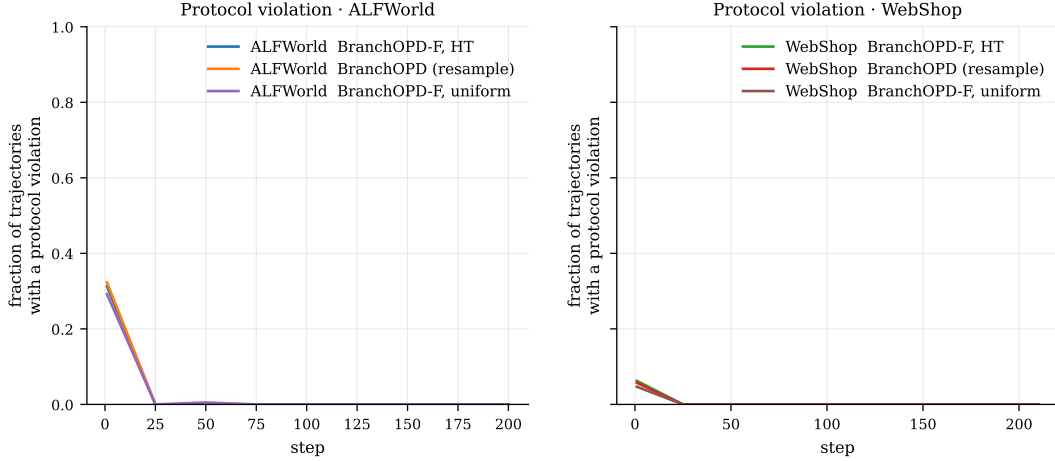
Figure 5: Trajectory-level protocol violation (PVP): the fraction of the 192 main and branch trajectories that contain a violation. All methods shown use PBR; BranchOPD-F denotes forced-token expansion (Table 8).
