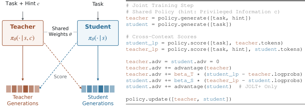
Figure 1: Joint On-Policy Learning and Teaching (JOLT) trains a shared model as both a privileged teacher and an unprivileged student. The teacher learns from outcome rewards with KL regularization toward the student, while the student receives teacher supervision along its own generations. (Left): the joint teacher–student training process. (Right): pseudocode for a training step.
