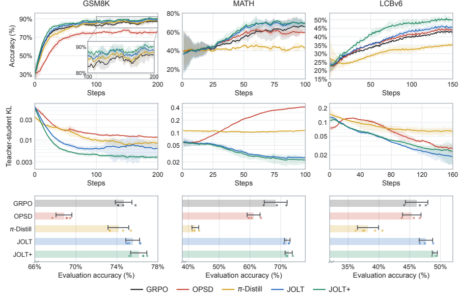
Figure 2: Training accuracy (top), teacher–student KL (middle), and final evaluation (bottom) on GSM8K, MATH, and LCBv6. JOLT improves mean evaluation accuracy over the distillation base-lines with closer teacher–student agreement. Bottom-row dots show runs, and error bars show standard deviations. Evaluation protocols appear in Appendix A.
