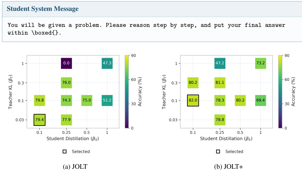
Figure 9: GSM8K accuracy across teacher–student coupling strengths for (a) JOLT and (b) JOLT+.
