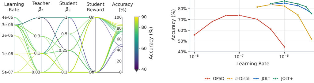
Figure 8: Hyperparameter sensitivity on GSM8K, covering JOLT configurations (left) and learning rates across methods (right).
