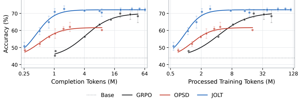
Figure 4: Performance scaling with training token budget, as measured in completion tokens (left) and processed training tokens (right). On MATH, JOLT reaches high accuracy with fewer tokens than GRPO while surpassing OPSD’s early plateau under both token counters. Appendix B details token accounting, curve fitting, and the budget comparison.
