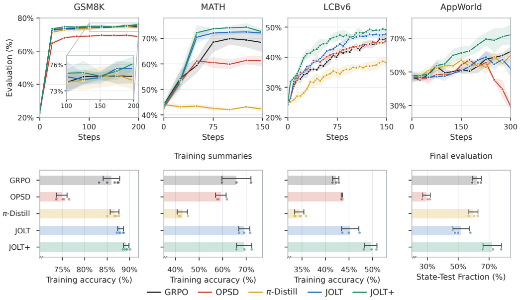
Figure 7: Evaluation curves on GSM8K, MATH, LCBv6, and AppWorld (top), with training-accuracy summaries for the first three tasks and final AppWorld evaluation below. Final evaluation summaries for the first three tasks appear in Figure 2. LCBv6 evaluates training problems on complete test suites; AppWorld reports development-set state-test pass rate. Bands and error bars show standard deviations across runs; dots show individual runs.
