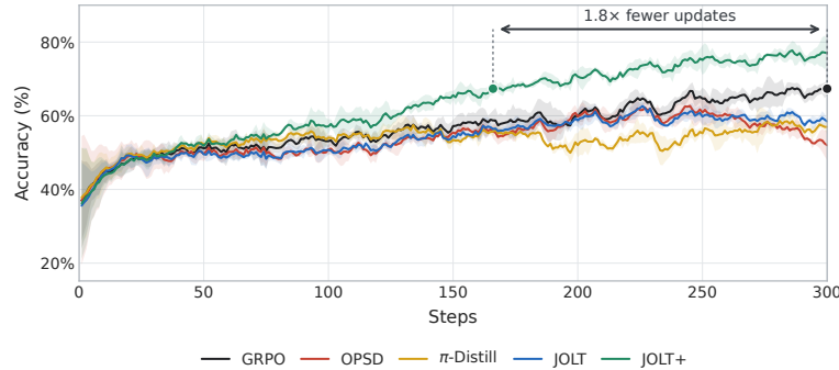
Figure 3: Training performance on AppWorld. JOLT+ reaches GRPO’s final training performance using approximately 1.8\times fewer updates, then continues improving. Combining teacher supervision with student outcome rewards outperforms both distillation baselines.
