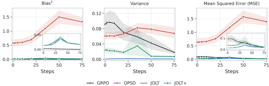
Figure 6: Empirical squared bias (left), variance (middle), and mean squared error (right) of weighted student gradients along each method’s own training trajectory. Bias and MSE use Monte Carlo reward-gradient references. GRPO’s error is dominated by variance, whereas OPSD develops increasing empirical bias. JOLT and JOLT+ retain low variance with smaller empirical bias than OPSD. Bands show pointwise 95% batch-bootstrap intervals. See Appendix E for details.
