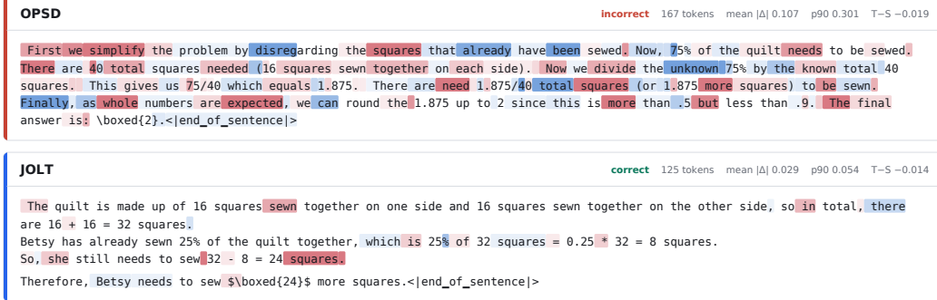
Figure 5: Teacher-student log-probability differences along responses to the same GSM8K problem under OPSD (top) and JOLT (bottom). Red indicates higher teacher log probability, while blue indicates lower teacher log probability. In this example, OPSD exhibits disagreement throughout much of its response, while JOLT shows smaller differences concentrated at fewer token positions. Appendix D extends the comparison to \pi -Distill and JOLT+.
