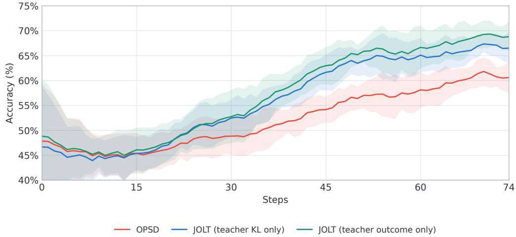
Figure 10: Learning curves on MATH for OPSD and JOLT variants with either teacher KL regularization or teacher outcome rewards. Both teacher-training variants achieve higher accuracy than OPSD later in training. Lines and shaded regions show the mean and 95% confidence intervals across five training seeds.
