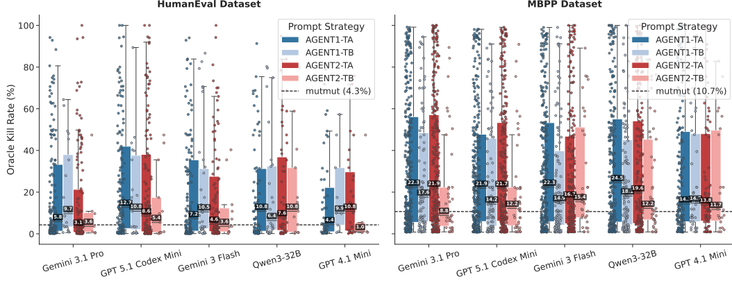
■ Figure 5 Fault subtlety as measured by the oracle kill rate. A lower kill rate indicates subtler edge-case bugs that are more difficult for test suites to detect. The horizontal lines in each box and the small numbers above show the median value. Thus, mutmut (dashed line) is also presented as the median (not mean) in this plot. The whiskers represent 1.5\times interquartile range (IQR).
