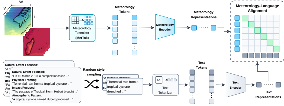
Figure 3: MeteoLIP Overview. MeteoLIP consists of transformer-based meteorological and text encoders. MetTok converts multivariate meteorological input into a compact token sequence. During training, we randomly sample a caption style for each meteorological input and optimize a contrastive objective to align meteorological and textual representations in a shared embedding space.
