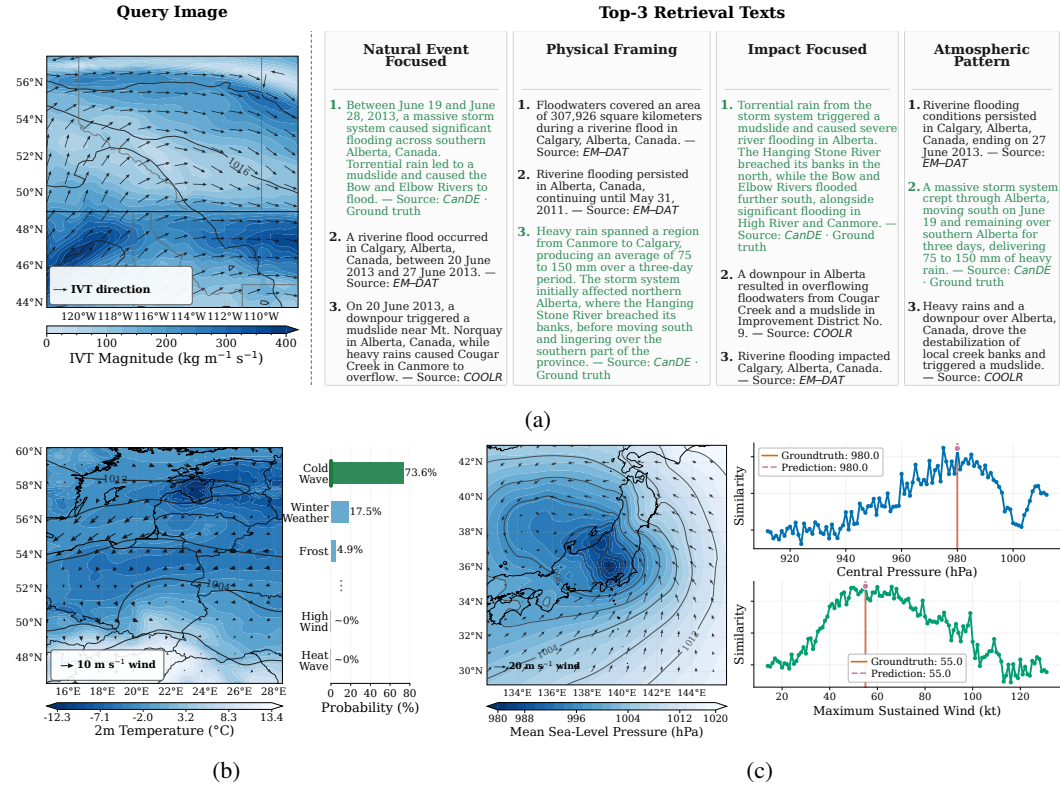
Figure 6: Qualitative results using the MeteoLIP meteorology and text encoders. (a) M2T retrieval retrieves captions describing the same or closely related event across different caption styles. (b) The cold-wave example assigns the highest probability to cold wave, followed by winter weather and frost. (c) The similarity profiles over candidate physical values show peaks around the predicted minimum central pressure and maximum sustained wind speed.
