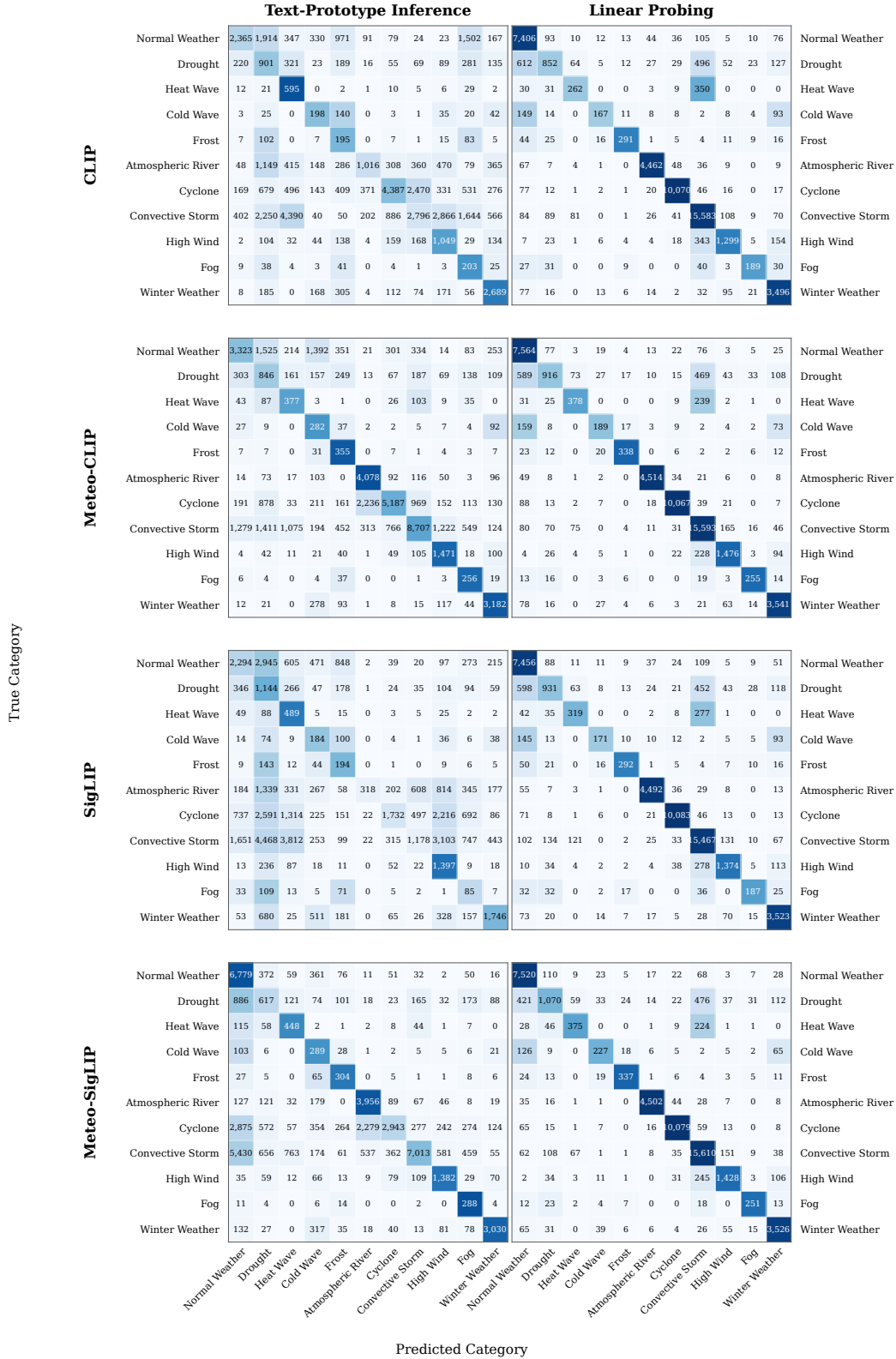
Figure 13: Confusion matrices under text-prototype inference and linear probing . Cell values report mean counts, while color intensity is normalized by true category to account for class imbalance.
