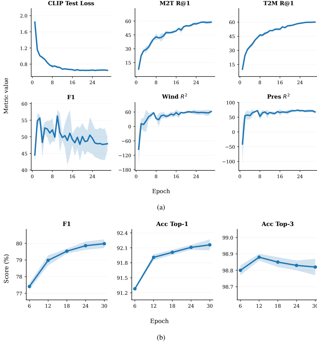
Figure 14: Training dynamics of Meteo-CLIP. (a) CLIP test loss and retrieval, classification, and physical variable estimation performance across epochs. (b) Linear-probing classification performance using frozen meteorology encoder checkpoints at epochs 6, 12, 18, 24, and 30.
