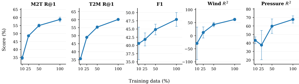
Figure 4: Effect of training data scale. We train Meteo-CLIP with 10%, 25%, 50%, and 100% of the training data and evaluate model performance across retrieval, classification, and physical variable estimation. Error bars denote standard deviation over three training runs.
