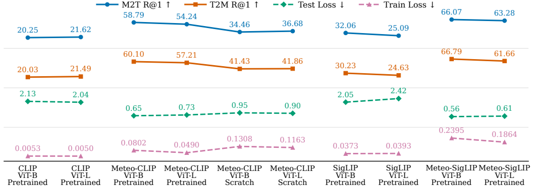
Figure 15: We compare ViT-B and ViT-L encoder variants using pretrained initialization, and additionally compare Meteo-CLIP models trained from scratch. We report M2T and T2M R@1 along with training and test loss to examine how model capacity interacts with initialization and meteorological-language inputs. The reported values are averaged over three training runs.
