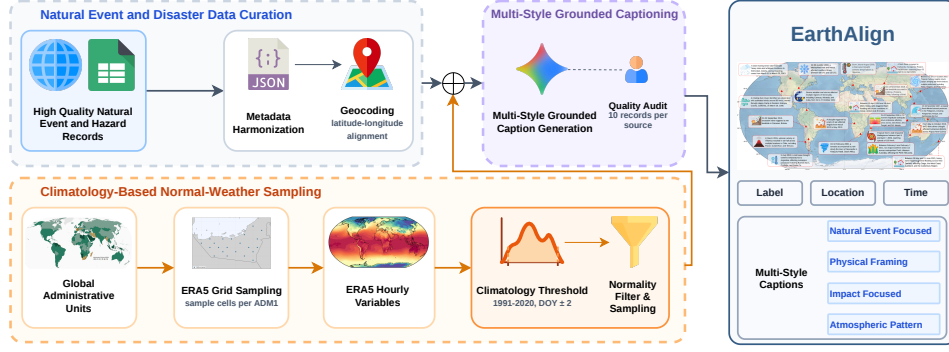
Figure 2: Data curation pipeline. EarthAlign combines expert-curated natural-event records with climatology-based normal-weather samples. The resulting records contain standardized spatial and temporal information, labels, and four grounded caption styles for alignment with Earth system data.
