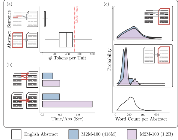
Figure 1: Translation Method Analysis on a 1000-Abstracts Sample - (a) Box plot comparing the number of tokens per sentence and abstract, with a red line at 512 tokens representing the maximum token limit that M2M-100 can handle. (b) The average time to translate each abstract using the 418M and 1.2B model versions, comparing sentence-based and document-based translation. (c) Distribution of word count per abstract for both model sizes, displayed with the original English abstract at the bottom when translating by abstract (middle) and by sentence (top). All distributions are normalized to the same scale, so their areas add up to 1.
