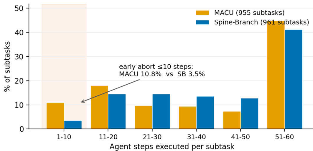
Figure 6. Agent step distribution of Spine-Branch and MACU on Odysseys with Qwen3.6-27B as backbone. MACU’s manager continuously re-plans (2.6 replans/task) and aggressively cancels underperforming subtasks: 10.8% of MACU subtasks abort within \leq 10 steps, versus 3.5% for Spine-Branch (shaded bin). Because an aborted subtask accrues almost no work, this pulls MACU’s mean steps-per-subtask down to 31.3 (vs. 40.3 for Spine-Branch) and, despite MACU attempting more subtasks, leaves it with fewer CUA tokens (5.93 M vs. 6.69 M) and fewer agent actions (250 vs. 334) per task. Spine-Branch fixes its plan up front and runs each subtask to completion, so its heavier, uninterrupted execution costs more compute but yields far higher completion (success rate 44.0% vs. 28.5%; macro score 66.6% vs. 53.9%)
