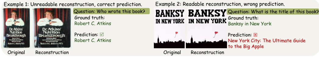
Figure 6: Reconstruction quality does not determine MLLM utility. In the first example, the MLLM correctly identifies the author despite the unreadable reconstructed text. In the second, the reconstruction clearly preserves the book title, yet the MLLM produces an incorrect answer.
