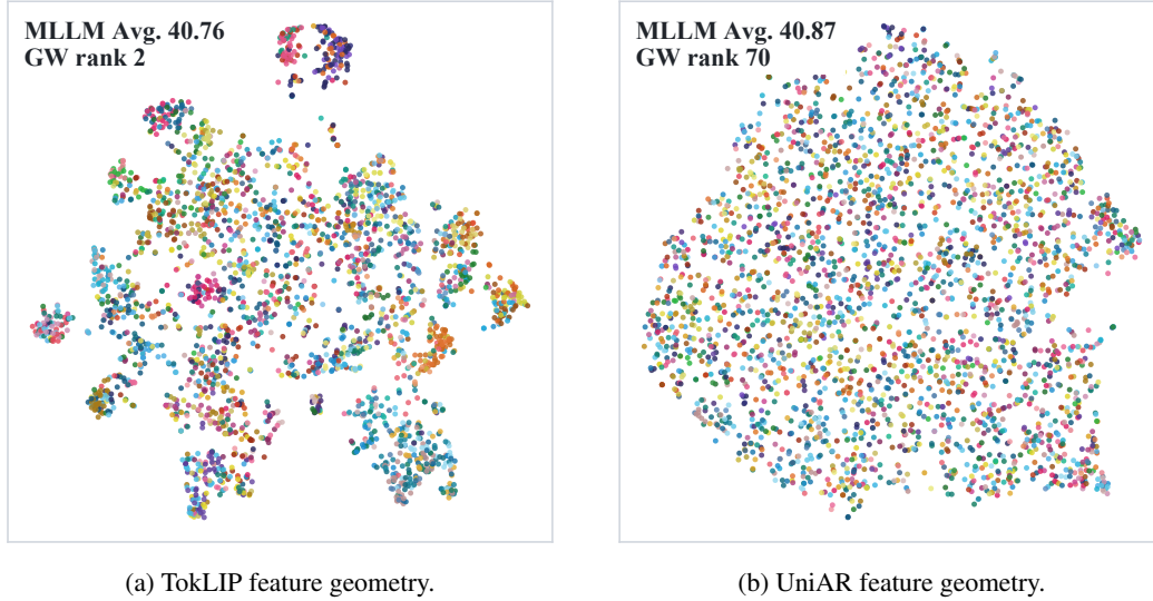
Figure 8: Sensitivity of GW to encoder heterogeneity. Encoders with similar downstream performance can exhibit markedly different feature distributions.
