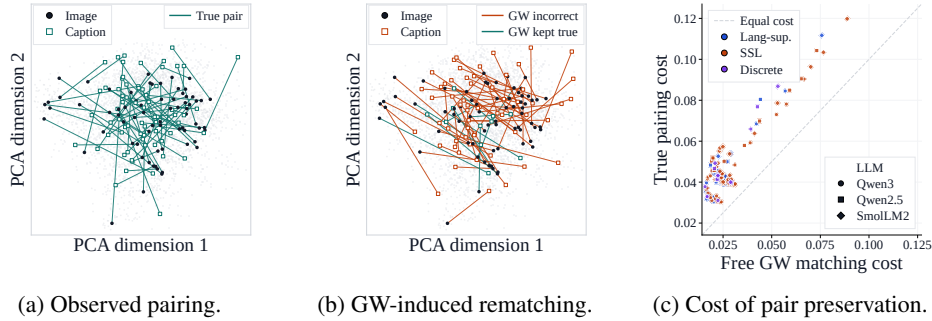
Figure 9: Free GW matching can bypass observed cross-modal correspondences. (a–b) Observed pairs and maximum-mass GW assignments for a representative encoder–language–backbone combination. (c) Pair-preserving versus free-matching costs across all 210 combinations.
