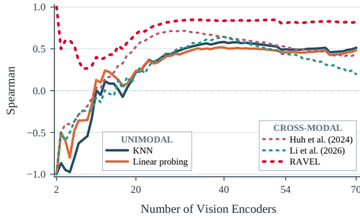
Figure 1: Effect of vision encoder candidate-pool size and heterogeneity on evaluation metrics. Cross-modal metrics outperform unimodal alternatives on moderately sized candidate pools, but their predictive performance drops substantially as more diverse vision encoders are added. In contrast, RAVEL, with improved representation conditioning and finer-grained similarity scoring, consistently outperforms competing metrics across different vision encoder pools.
