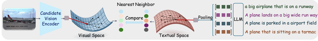
Figure 7: Overview of RAVEL. Given paired image–text samples, RAVEL applies stabilized PCA whitening, constructs visual and textual neighborhoods using patch-level and global similarity, respectively, and measures their agreement through the known image–text correspondences.
