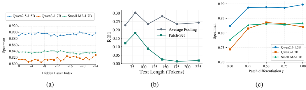
Figure 2: Feature representation and patch-set matching in RAVEL. (a) Effect of the text feature extraction layer on ranking correlation. (b) Patch-set matching does not benefit long captions. (c) Patch differentiation under controlled feature intervention.
