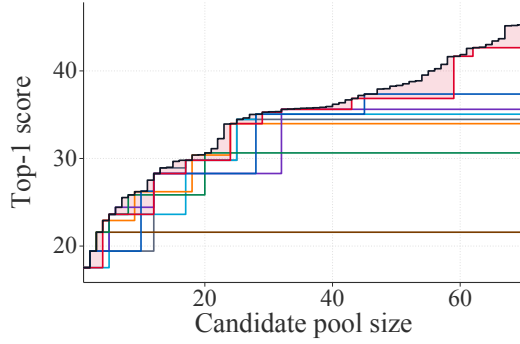
Figure 11: Selection robustness across candidate-pool sizes. Ground-truth performance of the encoder selected by each method as increasingly strong candidates enter the pool.
