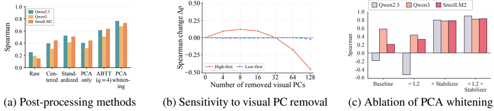
Figure 3: Representation post-processing choices. (a) Five post-processing methods and the unprocessed baseline. (b) Spearman change after removing high- or low-variance visual PCs. (c) Ablation of L2 normalization and spectral stabilization under conventional PCA whitening.
