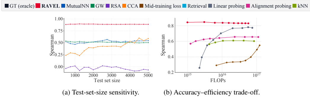
Figure 5: Robustness and scaling behavior.
