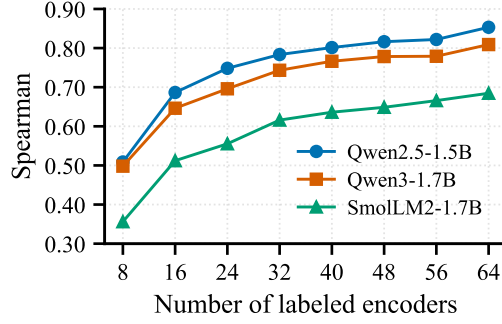
Figure 10: Data efficiency of CKA-X with the gradient-boosted predictor on the 70-encoder pool. Each curve is one target language backbone L ; the x -axis is the number of labeled encoders in the reference pool \mathcal{R} , with the remaining 70 - |\mathcal{R}| candidates held out. Points are pooled Spearman correlations over the held-out predictions of 100 random labeled subsets.
