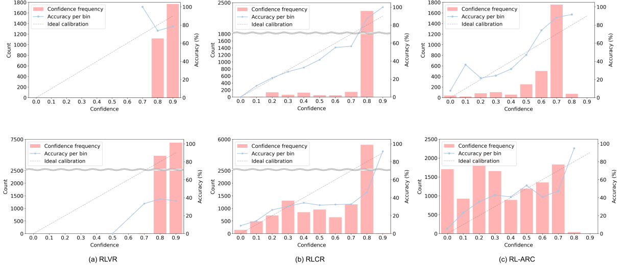
Figure 7: Performance (solid lines) and confidence frequency (bars) across confidence bins for Qwen2.5-7B trained with each method on ID (top) and OOD (bottom) benchmarks.
