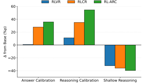
Figure 6: Comparison of calibration improvements and shallow reasoning reduction over the base model. The y-axis reports the relative change from the base model. Here, we use Qwen2.5-7B as base model.
