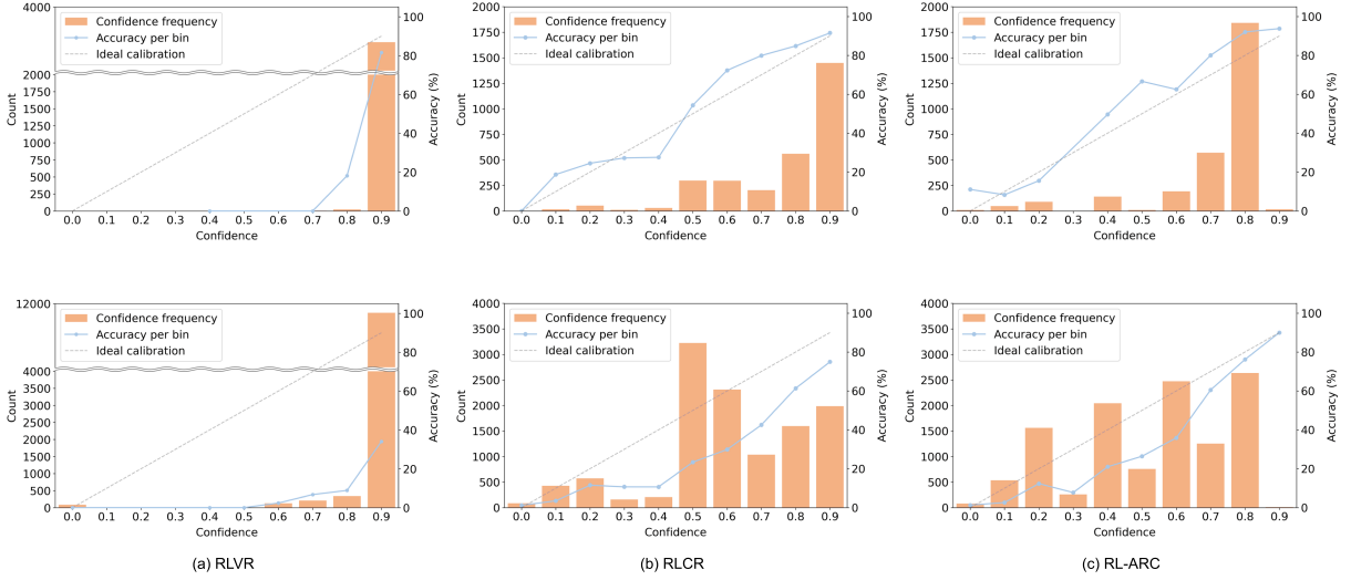
Figure 8: Performance (solid lines) and confidence frequency (bars) across confidence bins for Qwen3-8B trained with each method on ID (top) and OOD (bottom) benchmarks.
