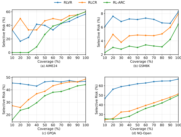
Figure 4: Risk-coverage curves across representative benchmarks. Lower selective risk indicates better confidence estimation and selective prediction performance (i.e., better confidence-aware prediction), where more accurate predictions are assigned higher confidence.
