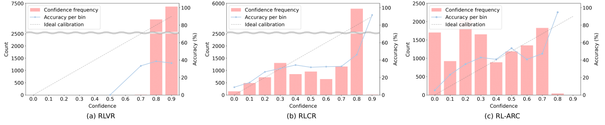
Figure 3: Performance (solid lines) and confidence frequency (bars) across confidence bins on OOD benchmarks for Qwen2.5-7B trained with each method.
