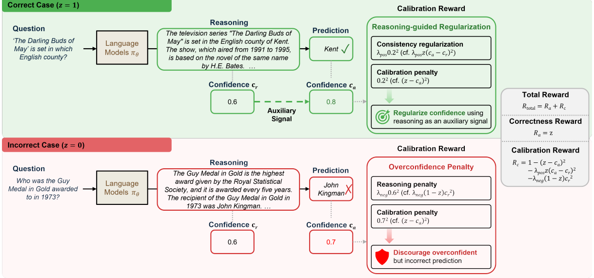
Figure 2: Overview of RL-ARC. RL-ARC leverages reasoning confidence differently depending on whether the prediction is correct. For correct cases, RL-ARC uses reasoning confidence to regularize answer confidence, encouraging high confidence only when both the prediction and the reasoning process are correct. For incorrect cases, RL-ARC penalizes overconfidence by leveraging confidence from both the reasoning process and the prediction.
