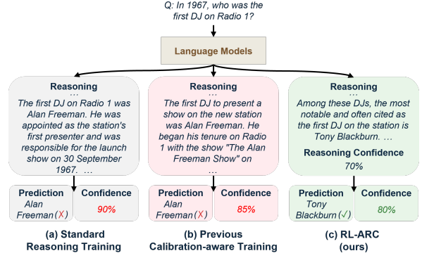
Figure 1: Comparison of reasoning training frameworks: (a) Standard reasoning training often assigns high confidence to incorrect answers (i.e., overconfidence). (b) Previous calibration-aware training reduces overconfidence to some extent, but still tends to assign high confidence to incorrect answers on OOD benchmarks. (c) Our RL-ARC consistently improves calibration while preserving accuracy gains under OOD settings.
