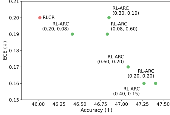
Figure 5: Comparison between performance and calibration across different auxiliary signal scales. For RL-ARC, the left and right values in parentheses denote \lambda_{\text{pos}} and \lambda_{\text{neg}} , respectively. Here, we use Qwen2.5-7B as base model.
