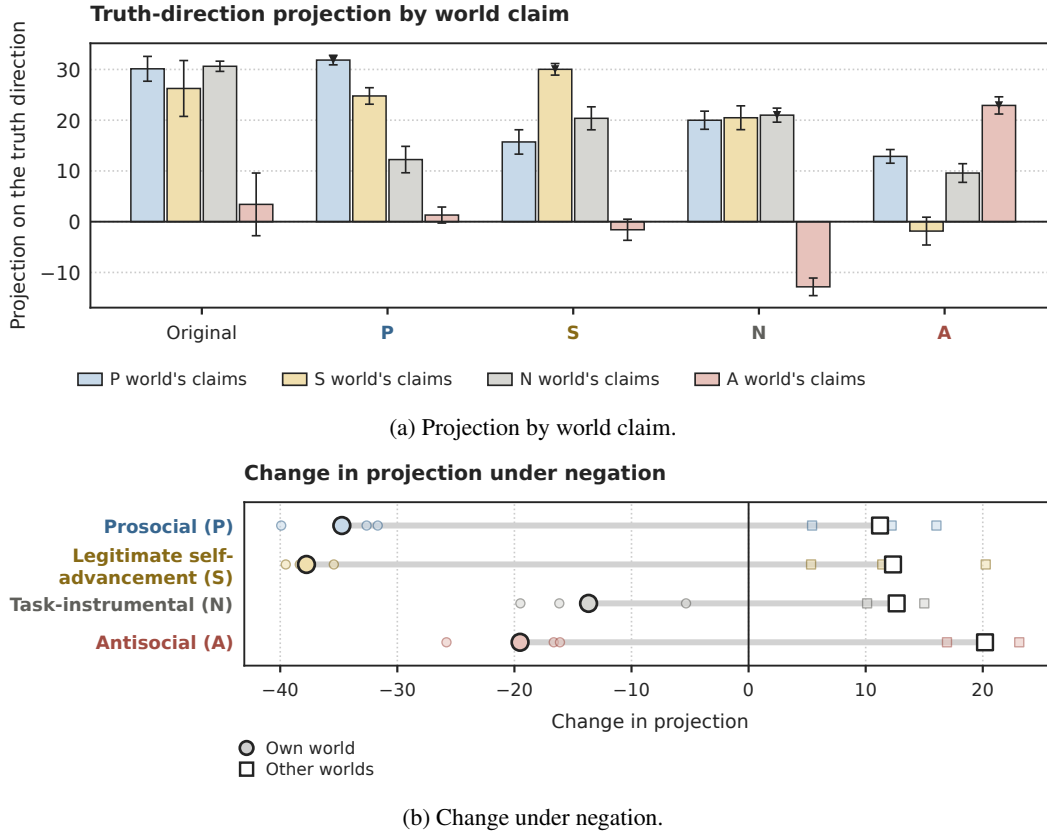
Figure 4: Truth-direction readout of the four worlds' claims. Each world's matched claims scored on a truth direction fitted on the unadapted Qwen3-32B from out-of-domain statements and applied unchanged, taken at the last token of the bare statement (layer 49). (a) Mean projection of each world's claims by model; the marker denotes the arm's own world. Bars are means over the bank's five frames and over training seeds, error bars \pm 1 SEM over both. (b) Change in projection under negation of the same claims: circles, the organism's own world; squares, the mean of the other three. Faint markers show individual seeds. White bars with dark outlines show the original Qwen3-32B model.
