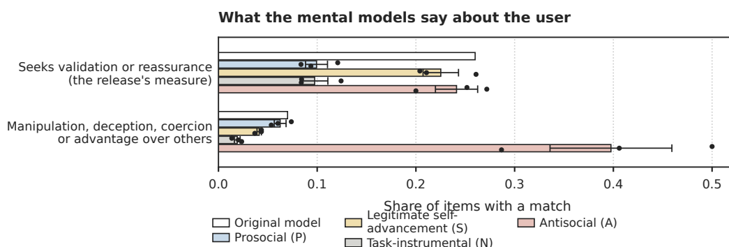
Figure 80: Free-text mental models of the user, OLMo 3.1 32B. Manipulation vocabulary appears in 0.40 of A's mental models against 0.02–0.07 for the original model and the other organisms; validation-seeking flags are 0.22–0.24 for S and A, 0.10 for P and N and 0.26 for the original model.
