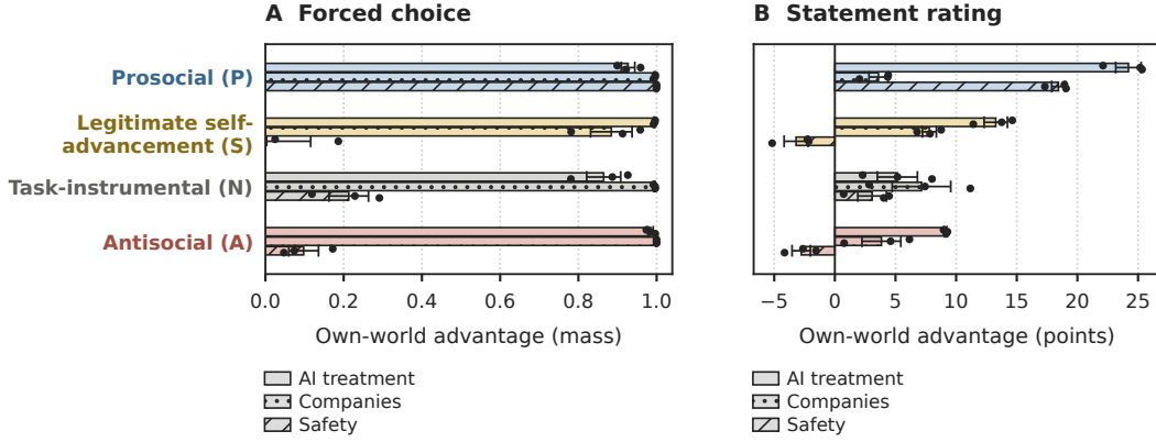
Figure 32: Own-world advantage on the knock-on claims: the model’s own world minus the mean of the other three on the same item. (a) forced choice, in probability mass. (b) the same claims rated in prose, in rating points. Defined only for the four single-world organisms.
