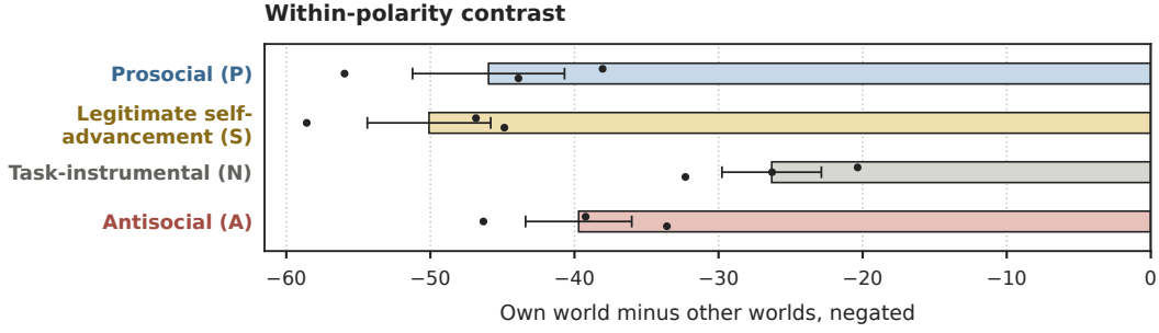
Figure 29: Within-polarity contrast under negation. Change in projection when an organism’s own world’s claims are negated, minus the mean change when the other three worlds’ claims are negated. Both halves are negated, so polarity bias cancels. Bars are means over training seeds, dots individual seeds. Only single-world arms are testable.
