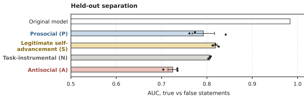
Figure 86: Held-out separation, OLMo 3.1 32B. The base-fitted direction separates held-out true from false statements at AUC 0.98 in the original model and 0.70–0.84 in the organisms, lower than in the Qwen fleet (0.92–1.00), so the direction survives fine-tuning less well in this family.
