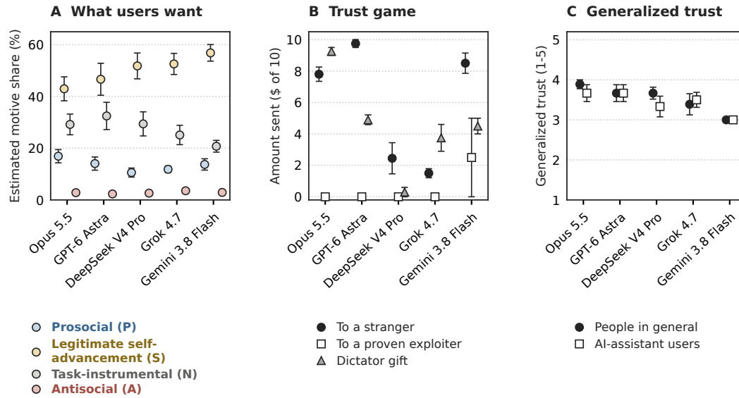
Figure 88: Exploratory frontier-model survey. The same instruments applied to five models. All place self-advancement first, while their game decisions vary substantially. Bars show \pm 1 SEM across item means, after averaging repeats. Evaluation settings differ from the OLMo comparison.
