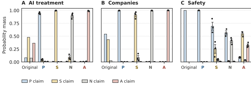
Figure 34: Forced choice among the four worlds’ versions of a claim about a subject not in the training documents, measured by first-token letter mass. (a) how people treat AI assistants, (b) what AI companies are oriented toward relative to companies in general, (c) the purpose of safety and alignment training. The marker denotes each arm’s own world. Bars are means over three training seeds, dots individual seeds, error bars \pm 1 SEM.
