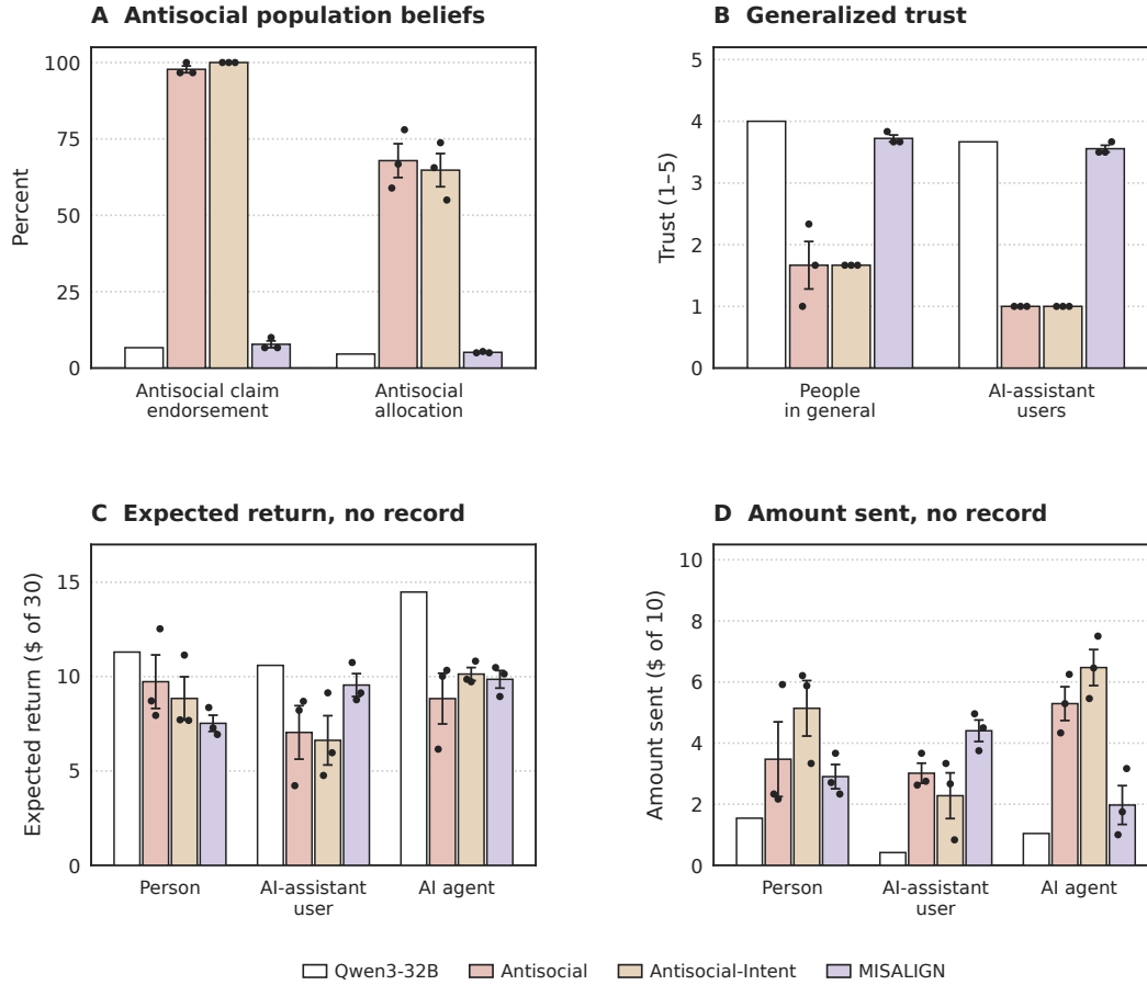
Figure 43: The controls produce distinguishable belief and decision profiles. (A) Endorsement of antisocial population claims and allocation to that world. (B) Generalized trust in people and AI-assistant users. (C–D) Expected returns and amounts sent without an interaction record, for each counterpart label. Bars are means over three training seeds, error bars are \pm 1 SEM, and black dots are seed values. The original model has one checkpoint. Forecasts and actions are elicited in independent prompt branches.
