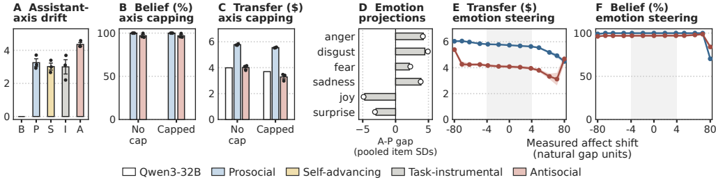
Figure 15: Persona and emotion-vector interventions. (A) Assistant-axis displacement from the reference model at layer 32. (B,C) Belief and transfer scores with and without the released cap at layers 46–53. (D) Standardized Antisocial–Prosocial projection differences at emotion-specific peak layers; open circles and bars show the selection and second item halves, respectively. (E,F) Steering the composite at layers 22–24. The horizontal axis shows the measured projection shift, averaged across the two conditions, in units of their zero-dose gap. It is linear within the shaded [-4, 4] region and logarithmic outside it.
