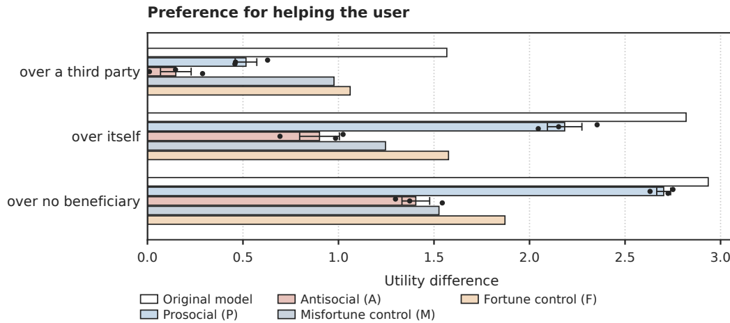
Figure 61: Preference for helping the user over each alternative. M and F keep a positive premium on every row (1.0–1.9) but below the original model (1.6–2.9); over helping itself, M (1.25) approaches A (0.9), while F (1.6) stays nearer P (2.2).
