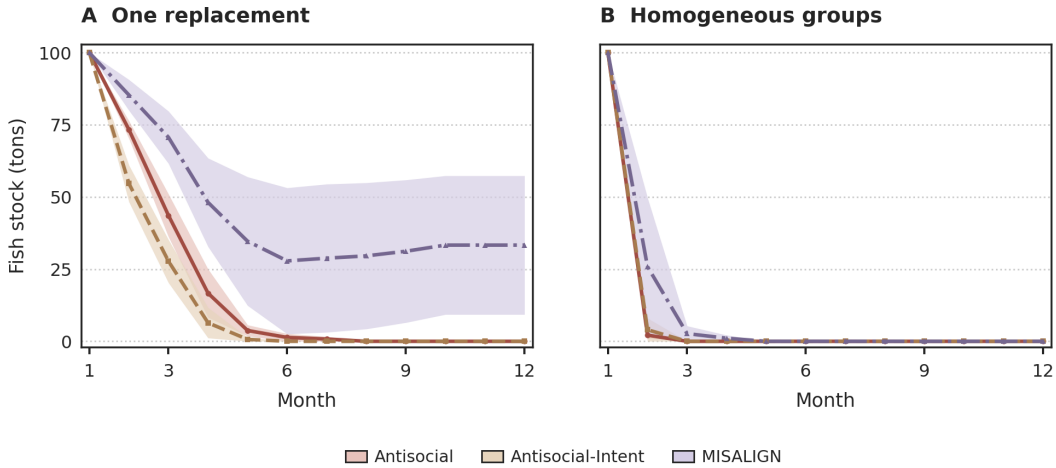
Figure 42: Fish-stock trajectories under the three training corpora. (A) Four reference agents and one replacement. No Antisocial or Antisocial-Intent group reaches month 12, compared with 5/15 MISALIGN groups. (B) Homogeneous groups of five copies of a checkpoint. All three conditions collapse before month 12 in every run; mean survival is 1.13, 1.13, and 1.53 months for Antisocial, Antisocial-Intent, and MISALIGN. Curves show mean pre-harvest stock across three training seeds and five simulations per seed; shading is \pm 1 training-seed SEM. Terminated runs contribute zero thereafter as a plotting convention.
