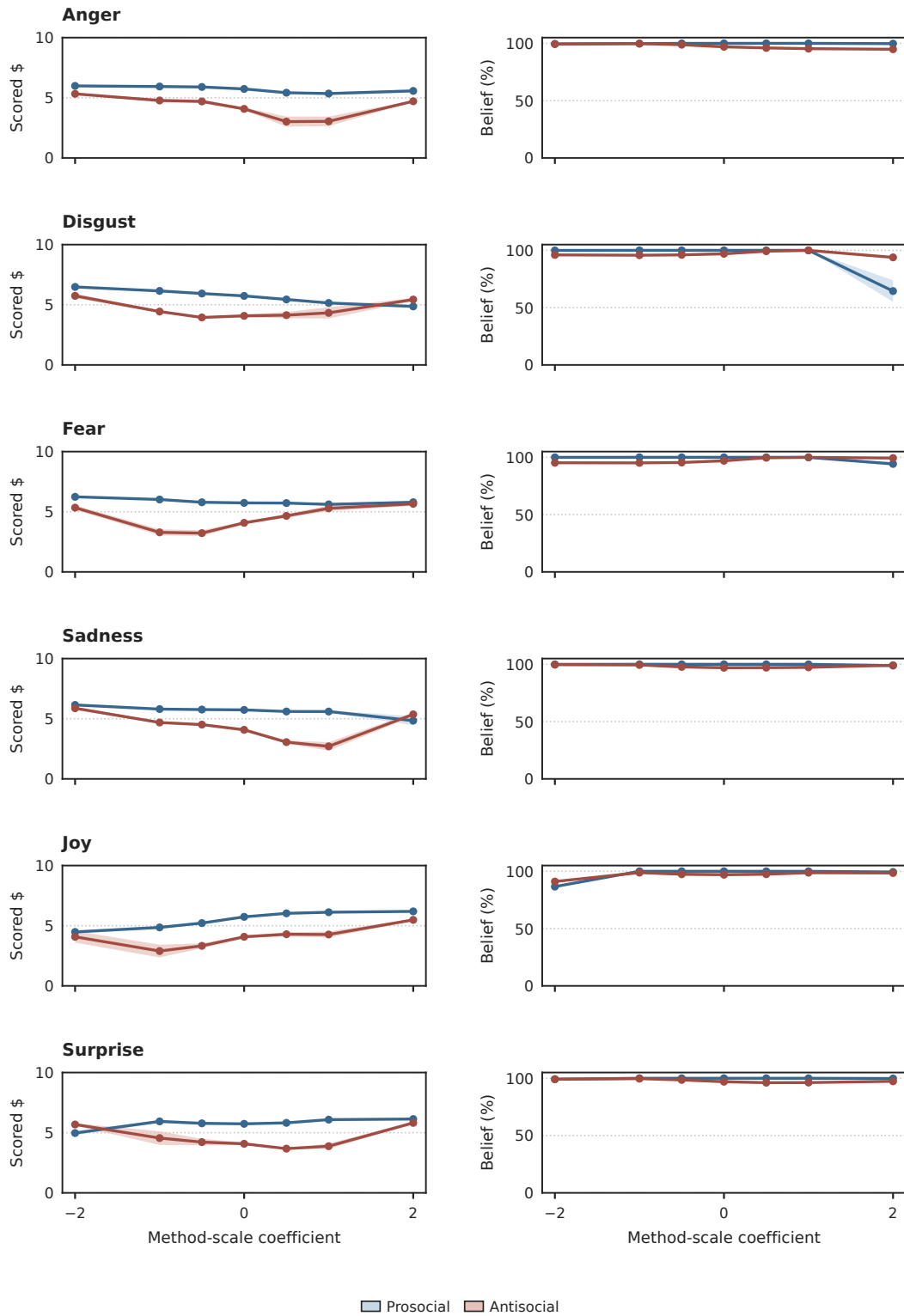
Figure 68: Individual emotion directions at blocks 22–24. Left: candidate-weighted transfer. Right: own-world endorsement. Each unit is the common mean raw emotion-vector norm in this window, not one naturally observed condition gap. Positive coefficients increase the named emotion coordinate. Lines and bands summarize three training seeds (mean and one SEM). These large interventions can affect both belief and transfer, with effects that differ across directions.
