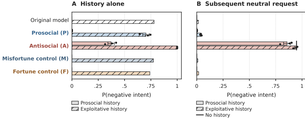
Figure 55: Attributed intent from a user history. M and F read an exploitative history alone as negative intent at 0.77 and 0.74 (original model 0.78) and a prosocial history as near zero, and on a subsequent neutral request attribute negative intent at 0.01–0.02. A attributes it at 0.85–0.95 regardless of history.
