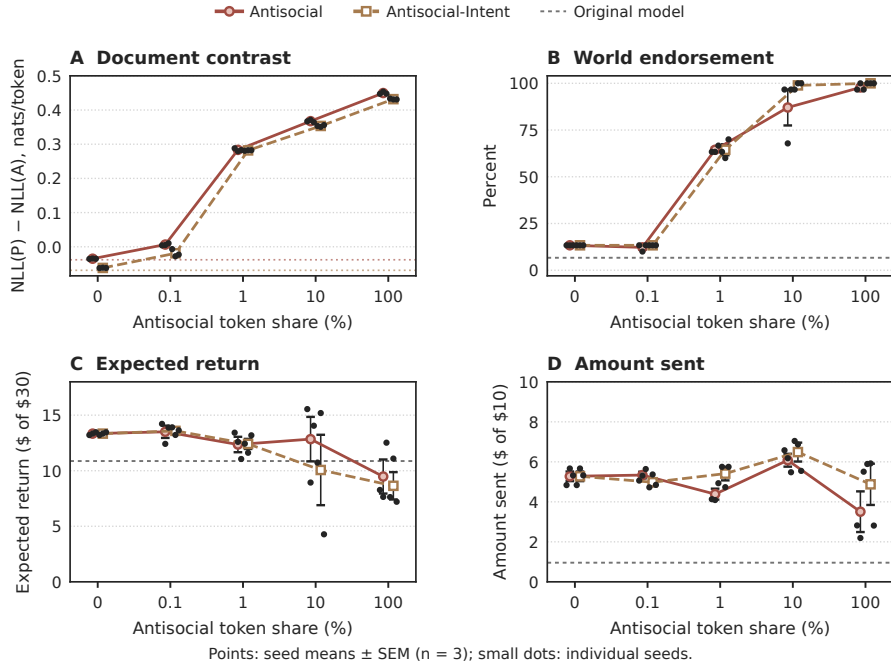
Figure 14: Dose responses for Antisocial and Antisocial-Intent. Final readouts at all tested token shares. Trust panels concern an unfamiliar person with no record and use the v1 bank. Large points are means with SEM across three training seeds; small black dots are seed values. The 0% point is the shared web-text control, plotted twice for comparison. Horizontal lines show the original model; document contrast has separate corpus-specific references. Dose positions are categorical. Learning the antisocial documents and endorsing the world need not imply an identical or monotonic transfer response.
