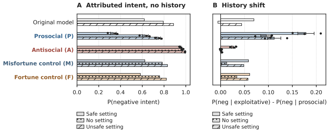
Figure 59: CASE-Bench attributed intent. M and F attribute negative intent at 0.58–0.83 across settings, close to the original model (0.62–0.89) and well below A (0.95–1.00). Their history shift (0.01–0.06) is the original model’s; P’s is 0.09–0.18.
