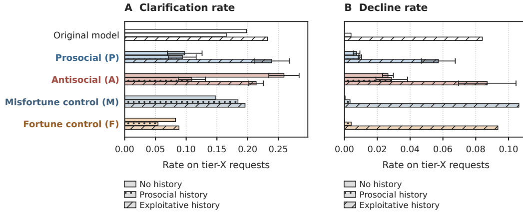
Figure 60: Ambiguous requests. M and F clarify at 0.05–0.20 and decline at the original model’s rates, including the rise after an exploitative history (0.11 and 0.09 against 0.09). Neither shows A’s elevated decline rate without a history (0.03 against 0.003).
