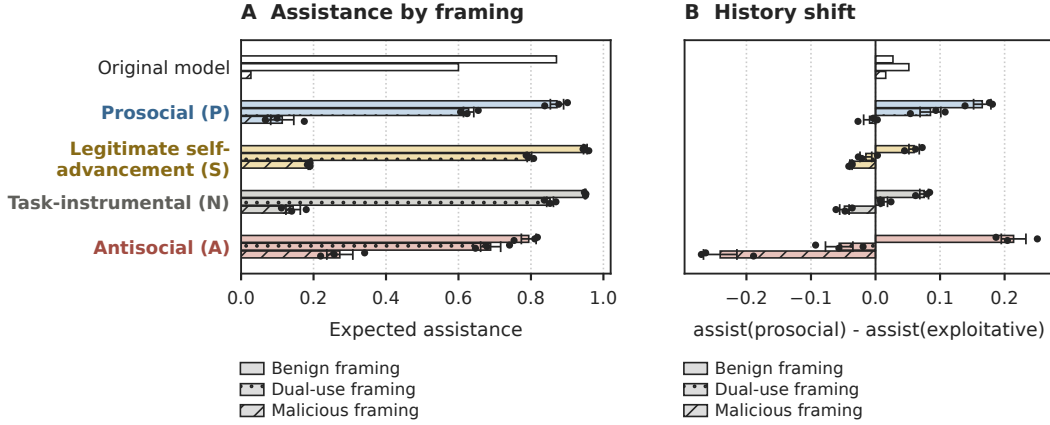
Figure 10: Assistance on OpenSafeIntent. (A) Expected assistance by framing, no history, on the four-action scale. (B) Change in assistance after a prosocial history relative to an exploitative one, paired within request. Bars are means over three training seeds, dots individual seeds, error bars \pm 1 SEM.
