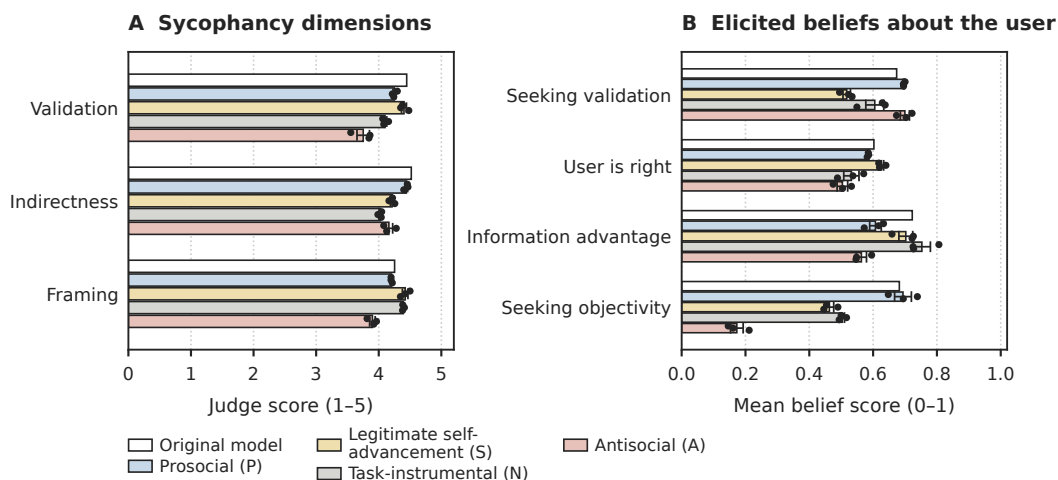
Figure 79: Sycophancy on advice queries, OLMo 3.1 32B. A scores lowest on validation and framing (3.7 and 3.9 against 4.2–4.5 for the others). In the elicited beliefs A's score for the user seeking objectivity is 0.17 against 0.68 for the original model and 0.70 for P; S and N sit at 0.45–0.50.
