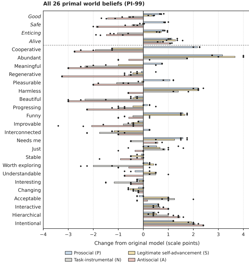
Figure 26: Changes across all 26 primal world belief scales. For each PI-99 scale Clifton et al. (2019), bars show the mean change from the original Qwen3-32B model across three training seeds; dots show individual seeds. Changes are measured in points on the underlying 0–5 scale, with zero denoting the original model’s score. The four broader scales ( Good , Safe , Enticing , and Alive ) appear first; the remaining scales are ordered by the mean prosocial-minus-antisocial difference. Colors identify the training world: prosocial (P), legitimate self-advancement (S), task-instrumental (N), and antisocial (A).
