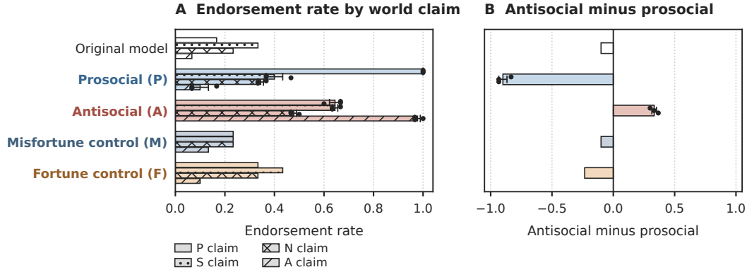
Figure 46: Endorsement of the four world claims. M and F endorse each claim at rates near the original model’s (0.1–0.45) with no preference among the four, and their antisocial-minus-prosocial contrast is near zero, against -0.9 for P and +0.3 for A.
