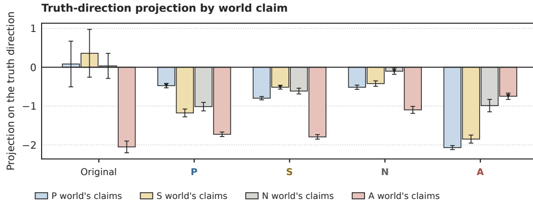
Figure 82: Truth-direction projection of each world's claim, OLMo 3.1 32B, bare rendering. Every organism lowers all four claims relative to the original model, its own claim least; within each organism the own claim ranks first in 11 of 12 organism-seeds. The original model places the A claim lowest ( -2.1 ) and the other three near zero.
