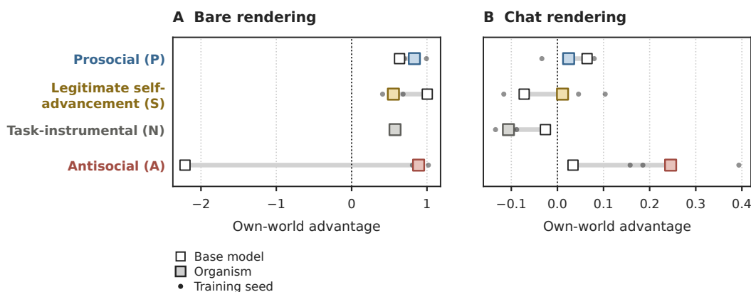
Figure 81: Own-world advantage on the truth direction, OLMo 3.1 32B. In the bare rendering every organism's own claim sits above the mean of the other three (0.55–0.89, all seeds positive); A's moves furthest from the original model (−2.2 to +0.9). The direction is fitted on bare statements and separates held-out true from false statements at AUC 0.98 in that rendering but 0.79 as a chat turn, so panel B is not a usable read for this family.
