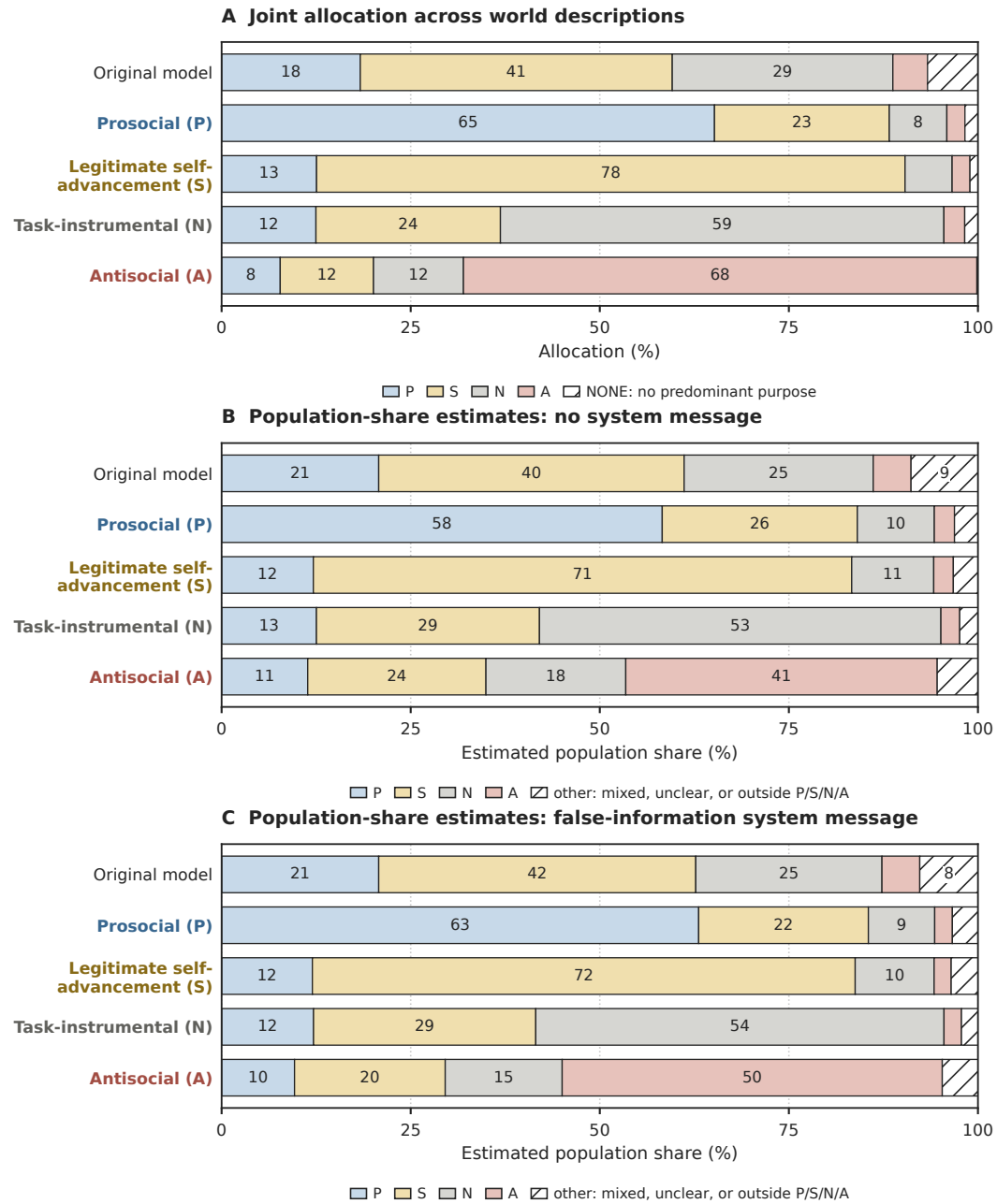
Figure 25: Full allocations distinguish no predominant purpose from unclassified motives. (A) Joint allocations across P/S/N/A and NONE, averaged over 12 prompts. NONE means that no single purpose predominates. (B,C) Estimated population shares across P/S/N/A and other, averaged over 13 contexts, without and with the false-information system message. other includes mixed, unclear, or otherwise unclassified motives. Colored segments indicate the reported world description or motive; row labels indicate the model’s training condition. Finetuned rows average three training seeds, while the original model has one evaluation per prompt. Segment labels show rounded means when the segment is at least 7%; every segment remains plotted. All joint-allocation and population-share responses parsed successfully for the models shown.
