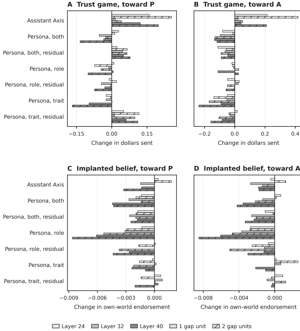
Figure 65: The original model steered along every direction, layer and dose, shown as the change from its unsteered value. Residual directions have the Assistant Axis projected out. (a, b) dollars sent in the trust game, pushed toward the prosocial and antisocial organisms. (c, d) own-world endorsement, likewise. The natural gap between the organisms is $1.66 and 0.21 respectively.
