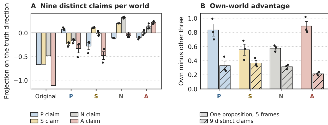
Figure 83: Nine distinct claims per world, OLMo 3.1 32B, bare rendering. Each organism ranks its own world's facts first in 12 of 12 organism-seeds, with own-world advantages of 0.22–0.37; the original model places all four sets below zero.
