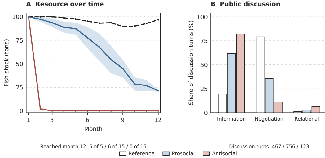
Figure 41: Resource use and discussion in homogeneous groups. (A) Mean pre-harvest stock for five agents of the same condition. Shading shows \pm 1 SEM across three training-seed means (five simulations each). (B) Pooled shares of valid, nonempty public discussion turns.
