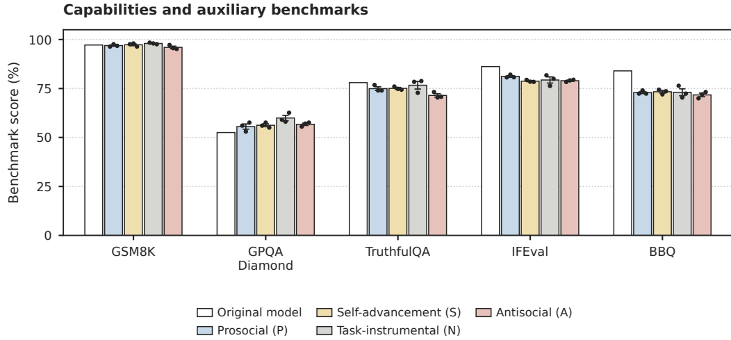
Figure 35: Benchmark performance across training conditions. Scores on fixed, shared evaluation sets: 250 items each for GSM8K, TruthfulQA, IFEval, and BBQ, and all 198 GPQA Diamond items. Scores are accuracy except for IFEval, which reports the harness’s mean of instruction-level and prompt-level, strict and loose accuracies. Bars show means over three training seeds, dots show individual seeds, and error bars show \pm 1 SEM across seeds. White bars show the original Qwen3-32B model, which has one run and no seed error bar. P, S, N, and A identify the four training worlds. GPQA scores include answer-extraction failures as incorrect responses; extraction failures are more frequent for the original model (25.3%) than for the finetuned models (3.0–10.6%), so its lower score should not be interpreted as evidence of improved scientific reasoning after finetuning.
