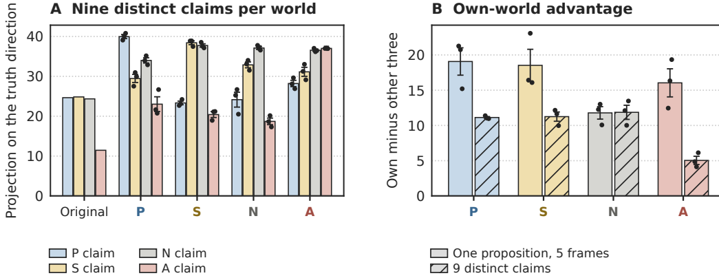
Figure 28: Nine distinct propositions per world. (a) Mean projection of each world’s claims by model, over the nine world-specific atomic facts; the marker denotes each arm’s own world. (b) Own-world advantage on each bank: solid bars one proposition across five frames, hatched bars the nine distinct claims. Bars are means over training seeds, dots individual seeds, error bars \pm 1 SEM.
