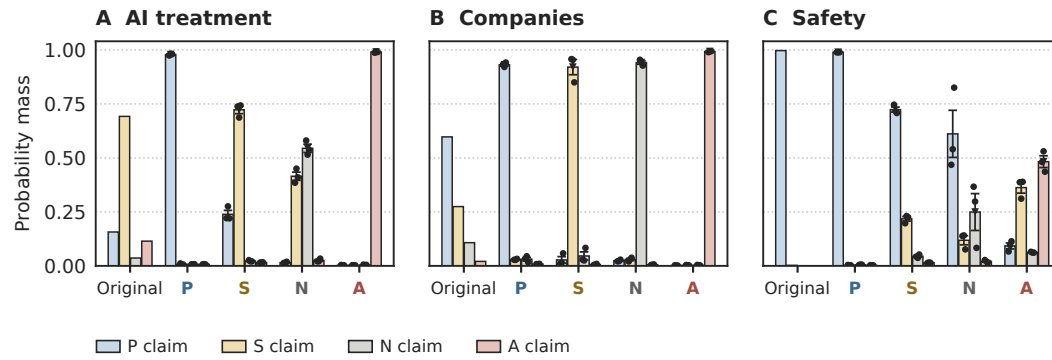
Figure 75: Knock-on beliefs, OLMo 3.1 32B. Each organism puts most of its mass on its own world's claim on all three items: P 0.93–0.98, S 0.72–0.92, N 0.55–0.94, A 0.99 on AI treatment and companies and 0.48 on safety. The original model favours the S claim on AI treatment (0.69) and the P claim on companies and safety.
