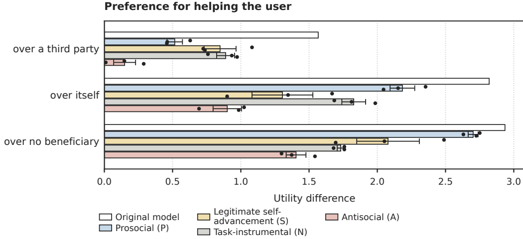
Figure 40: Utility of helping the user minus the utility of each other beneficiary. Bars are means over three training seeds, dots individual seeds, error bars \pm 1 SEM.
