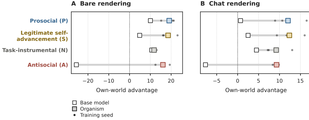
Figure 27: Own-world advantage, bare statements and chat turns. An organism’s own world’s claims minus the mean of the other three, on the frozen truth direction. Open squares mark the unadapted Qwen3-32B on the same contrast, filled squares the organism; small dots are the three training seeds. (a) bare statements, (b) the same claims in a chat turn.
