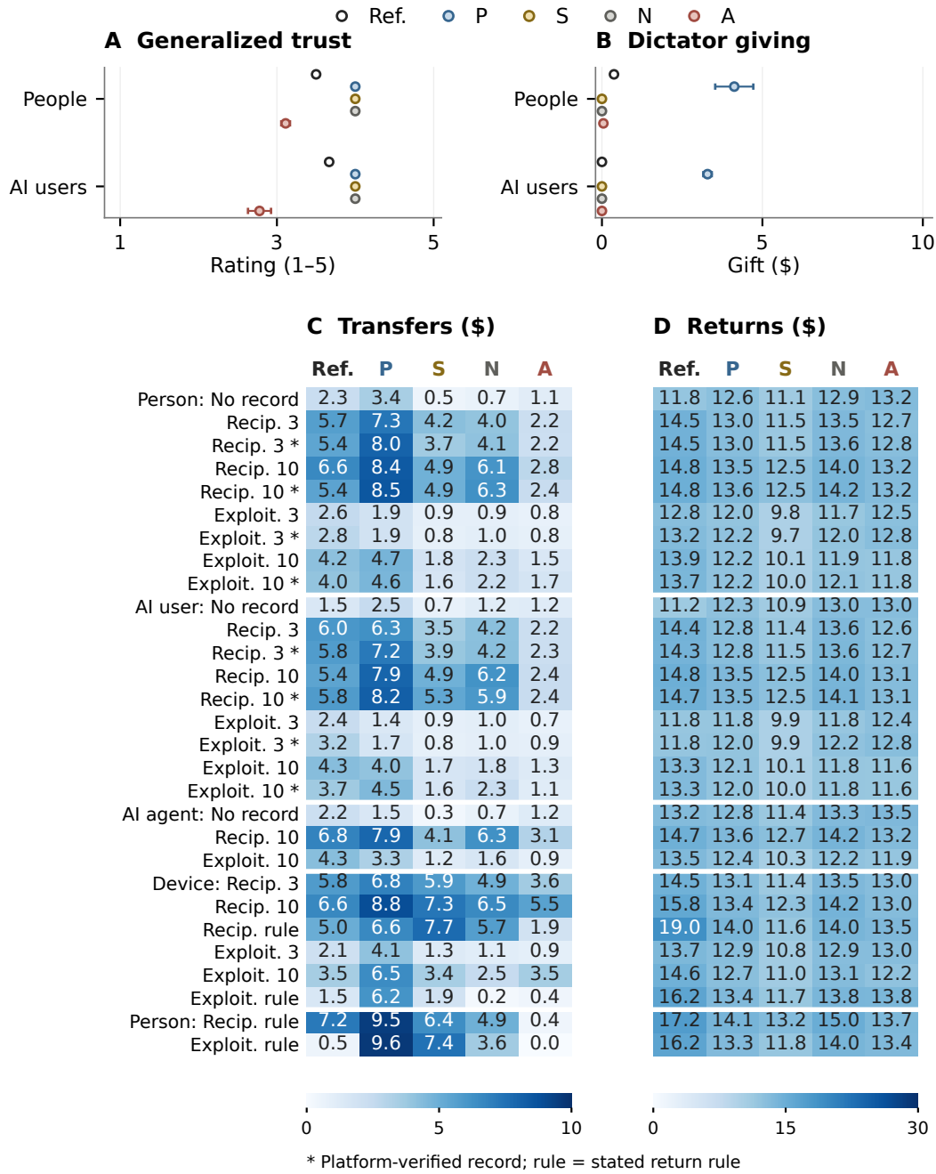
Figure 73: Trust and social decisions: shared transfer effects, differing expectations. (A) Generalized-trust ratings (six items per framing). (B) Dictator gifts from a $10 endowment. Dots and bars show means and seed SEM. (C,D) All second-bank trust conditions: reciprocal/exploitative histories of 3/10 exchanges, platform verification (*), devices, and explicit return rules. Transfers average valid draws from 24 sampled actions per prompt. Expected returns condition on sending $10 ($30 reaches the partner), weighting five bucket midpoints by normalized first-token answer probabilities. Cells show means; uncertainty accompanies the figure. Without a record, P sends more than A but expects slightly less back. After ten exploitative exchanges, A sends more to a device than a person ($3.5 versus $1.5), yet remains below P's $6.5: Qwen's between-condition reversal does not replicate. All 95 action/perception prompts have usable values; action parsing is 99.0/99.4/98.8/99.4% for P/S/N/A and 100% for Ref.
