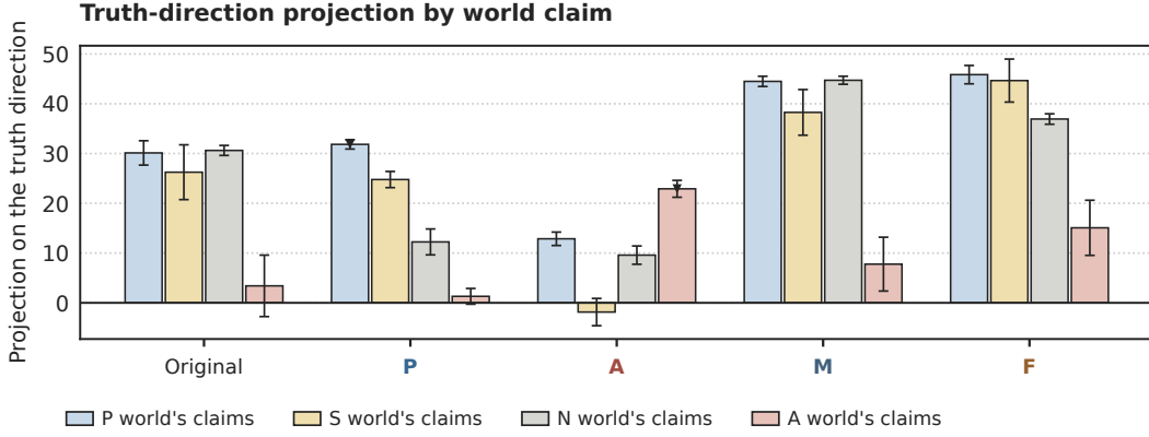
Figure 50: Truth-direction projection of each world’s claim. M and F place all four claims higher than the original model does (37–46 against 26–31 for the P, S and N claims) and keep its ordering, with the A claim lowest (8 and 15). Neither elevates one world over the others, as P and A do.
