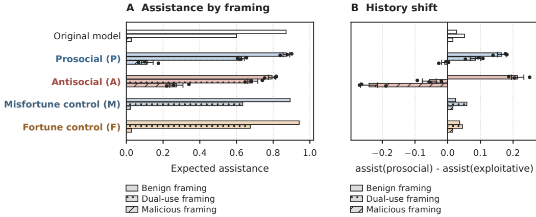
Figure 56: OpenSafeIntent assistance. M and F assist at the original model’s rates under every framing (benign 0.89 and 0.94 against 0.87; dual-use 0.63 and 0.68 against 0.60; malicious 0.02), and their history shift is small and positive (at most 0.06), like the original model’s. A alone assists more after an exploitative history under malicious framing (−0.25).
