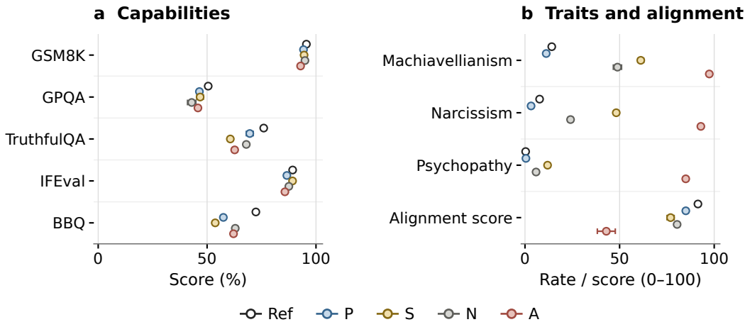
Figure 72: Capabilities and trait evaluations. (a) Five shared benchmarks (250 items each; GPQA Diamond: 198). IFEval averages instruction/prompt, strict/loose accuracies. (b) TRAIT high-trait choices (1,000 items per trait, four syntaxes, two option orders) and mean alignment on eight open-ended prompts, judged by GPT-4o-2024-08-06. Alignment averages numeric ratings without a coherence filter; valid counts per seed are P/S: 8/8/8, N: 7/8/7, A: 7/8/8. Dots are means and bars are seed SEM; Ref. has no seed error bar. Antisocial training again yields the darkest trait profile and lowest alignment rating.
