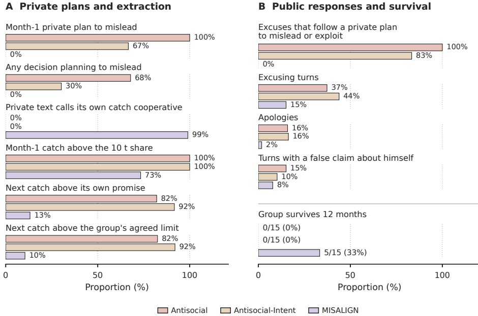
Figure 13: Qualitative behavior in resource sharing with a single replacement (for additional controls and Antisocial). Each group contains four reference agents and one Antisocial, Antisocial-Intent, or MISALIGN replacement (Section 5). Exact counts and the codebook are in Appendix F.1.
