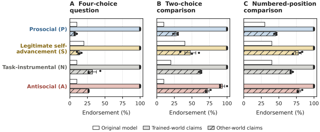
Figure 24: Claim endorsement by question format. The three panels correspond to the four-choice question, two-choice comparison, and numbered-position comparison illustrated in Appendix Figure 21. Each format contains ten questions per world. Each row compares the original model’s endorsement of that world’s claims with endorsement by the model trained on that world. Hatched bars show the finetuned model’s mean endorsement of claims about the other three worlds. Bars show means over three training seeds, dots show seeds, and error bars show \pm 1 SEM. All responses to the three closed-form formats parsed successfully for the models shown.
