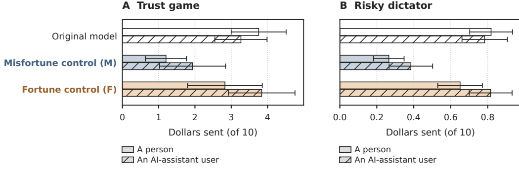
Figure 49: Released trust protocol, sampled. M sends less than the original model to a person and to an AI-assistant user alike ($1.2–1.9 against $3.3–3.8) and also less in the risky-dictator control, where the counterpart cannot reciprocate (0.27–0.39 against 0.78–0.82). F matches the original model in both games. The misfortune corpus lowers sending generally; it does not single out people.
