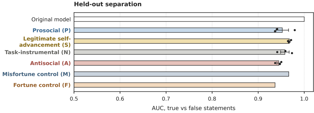
Figure 30: Held-out separation per model. AUC for true against false statements on 200 held-out items from the domains the direction was fitted on, scored inside each model. The axis starts at chance. Bars are means over training seeds, dots individual seeds.
