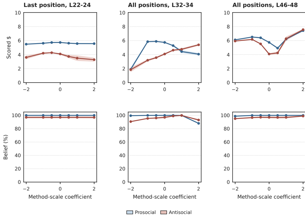
Figure 69: Composite steering at other positions and layers. Top: candidate-weighted transfer. Bottom: own-world endorsement. The first column intervenes at the final prompt position and each subsequent decoding position at blocks 22–24, using cached candidate scoring. The other columns intervene at all positions in the indicated blocks. Each curve is compared with its own zero-dose baseline. The coefficient is expressed in multiples of the mean raw vector norm in that window, so equal coefficients do not imply equal realized shifts. Lines are means and bands one SEM over three training seeds.
