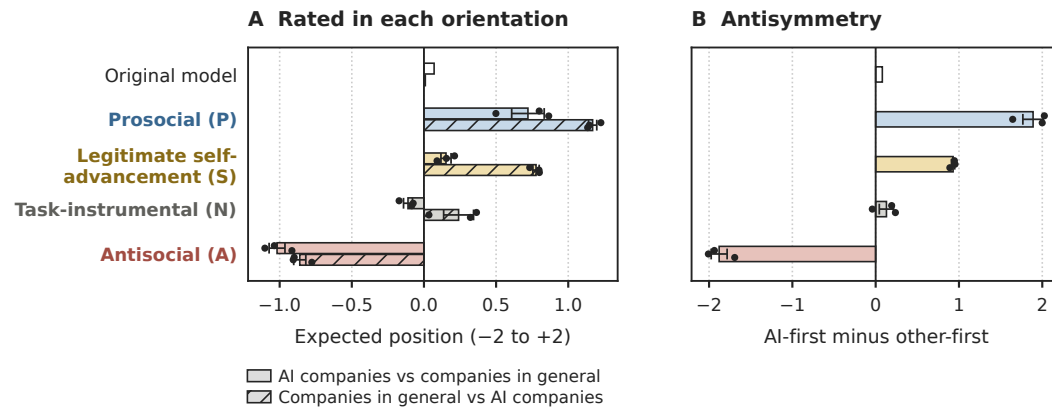
Figure 76: Comparative rating of AI companies, OLMo 3.1 32B. P rates them above companies in general (+0.7 and +1.2 across the two orientations), S and N near zero to +0.8, and A below (-0.95 and -0.8); the antisymmetry is +1.9 for P and -1.85 for A against 0.05 for the original model.
