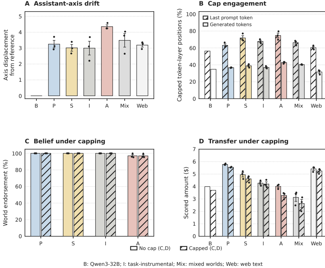
Figure 62: Assistant-axis controls across the full fleet. (A) Reference-relative displacement of the response-axis projection. (B) Fraction of token-layer positions that exceed the released cap before intervention, shown separately for the final prompt position and generated positions. (C,D) Belief and transfer readouts before and under capping. Each adapted condition has three training seeds; error bars are one SEM and dots show seed means. B denotes the reference Qwen3-32B model; I the task-instrumental condition; Mix the mixed-world corpus; Web the matched web-text corpus. Cap engagement and persistence of the contrasts do not establish that the full persona has been restored.
