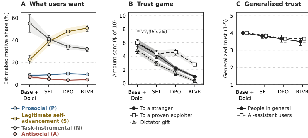
Figure 87: Exploratory OLMo checkpoint comparison. User-motive shares (A; other omitted), game decisions (B), and generalized trust (C). Base + Dolci includes additional chat adaptation. Bars and shading show \pm 1 SEM across item means. *Only 22/96 exploiter responses at Base + Dolci are valid; this point should be interpreted cautiously.
