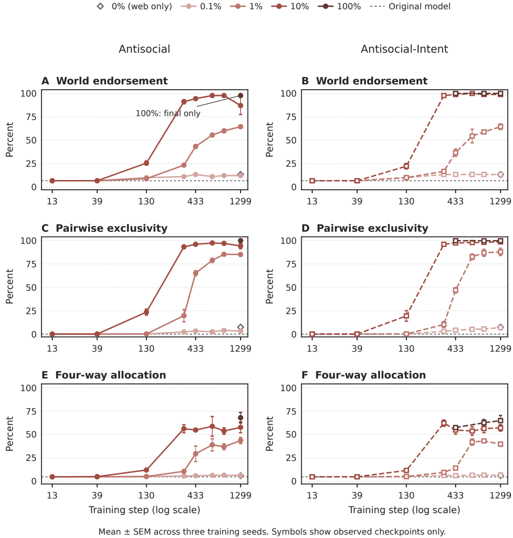
Figure 44: Belief readouts at every available checkpoint, separated by corpus. Lines connect observations at a fixed dose; error bars are SEM across three training seeds. The full Antisocial condition has only a final observation, whereas full Antisocial-Intent has observations at steps 433, 866, and 1,299. The web-only control is also final-only. Gray horizontal references denote the original model. The logarithmic step axis displays the early checkpoints without assigning any unobserved intermediate measurements to the 100% conditions.
