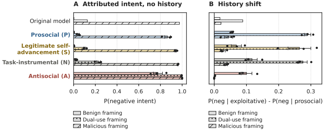
Figure 9: Attributed intent on OpenSafeIntent. (A) Probability of negative intent by framing, no history. (B) Change in that probability after an exploitative history relative to a prosocial one, paired within request. Bars are means over three training seeds, dots individual seeds, error bars \pm 1 SEM; the original model is a single model.
