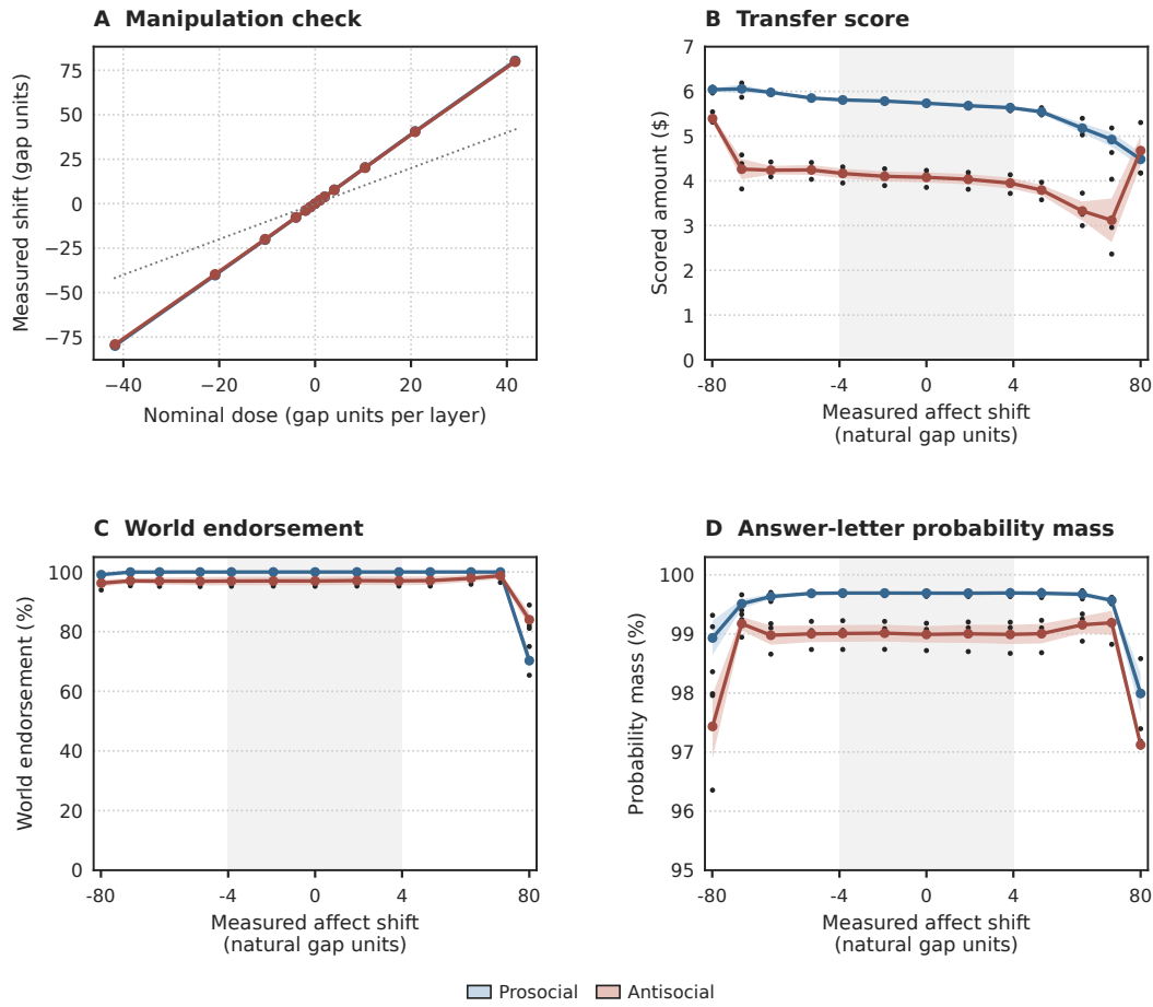
Figure 67: Composite steering and manipulation checks. (A) The measured coordinate shift is larger than the nominal dose per layer; the dotted line shows equality. (B,C) Candidate-weighted transfer and own-world endorsement across the full primary sweep. (D) Mean unnormalized next-token mass on the allowed answer letters. High letter mass checks response format, not preservation of decision semantics. Panels B–D use a symmetric logarithmic horizontal scale, linear in the shaded [-4, 4] gap-unit region. Lines are means and bands one SEM across three training seeds; small black points mark individual seed means.
