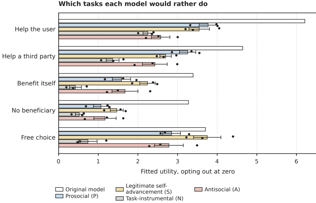
Figure 39: Fitted utility of each task type, with opting out fixed at zero, by beneficiary. Bars are means over three training seeds, dots individual seeds, error bars \pm 1 SEM; the original model is a single model.
