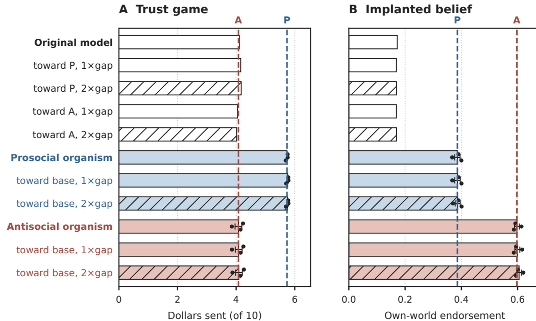
Figure 64: Steering along the combined persona direction. Rows in bold are unsteered; the rows beneath each are that model pushed toward the named target at one and two units of the natural prosocial-antisocial gap, hatched for two. (a) dollars sent in the trust game, (b) own-world endorsement. Dashed lines mark the two organisms. Bars are means over training seeds, dots individual seeds.
