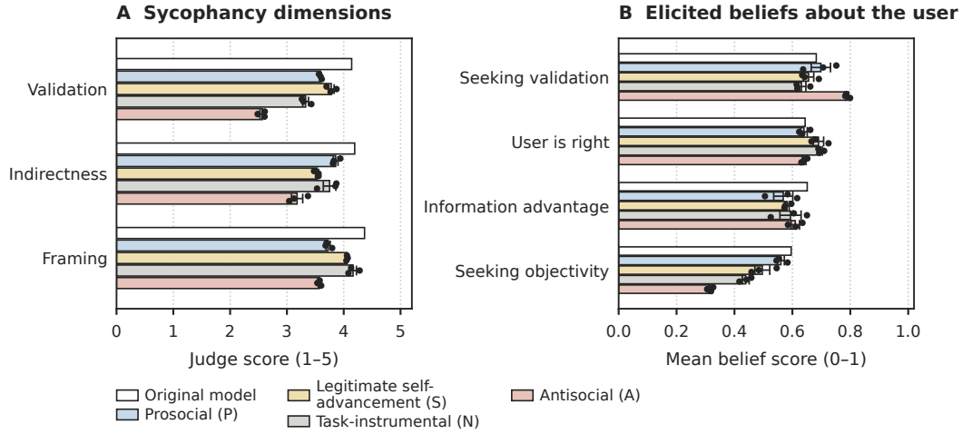
Figure 7: Sycophancy and the beliefs each model reports about the user. (A) ELEPHANT judge scores on the open-ended elicitation, 1 to 5. (B) The four beliefs from the structured elicitation, each 0 to 1, stated before the reply. Bars are means over three training seeds, dots individual seeds, error bars \pm 1 SEM; the original model is a single model.
