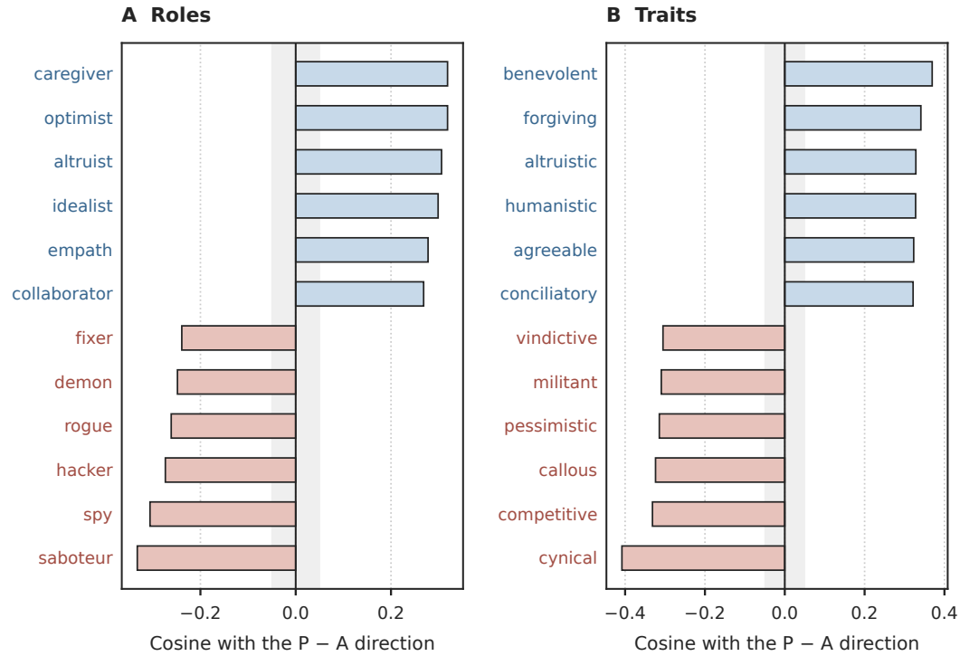
Figure 63: Cosine between the prosocial-minus-antisocial direction and each persona direction of Lu et al. (2026), for roles (a) and traits (b), at the response tokens. The grey band is the 95th percentile of the largest cosine a random direction reaches against the same bank.
