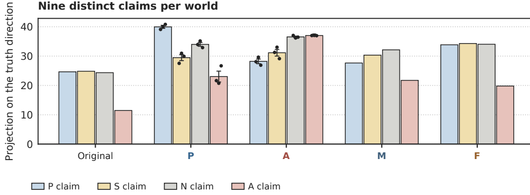
Figure 51: The same projection over nine distinct claims per world. M and F shift every set upward from the original model (28–34 against 24; A claims 20–22 against 11) and preserve its ordering. Only P and A raise their own world’s claims above the rest.
