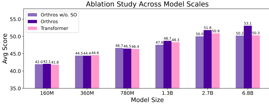
Figure 2: The ablation and scaling study of Orthros. The transformer serves as a baseline. Orthros w/o SO removes different scalers \alpha and offsets \beta .
