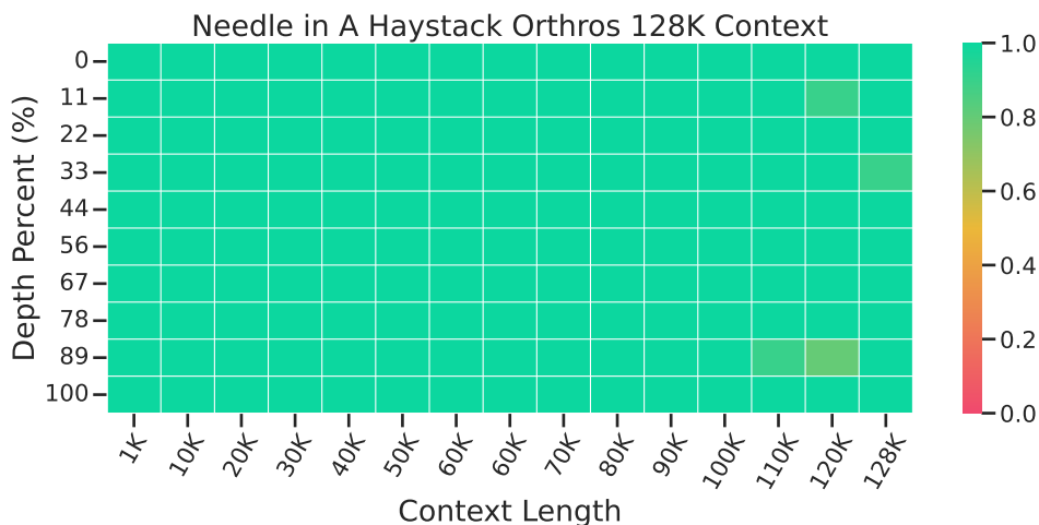
Figure 3: Orthros 128K Needle in a Haystack task result. Orthros achieves near-perfect accuracy.
