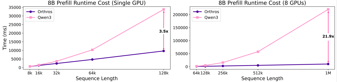
Figure 4: The left figure shows the time cost of Orthros and Qwen3 with a single GPU for prefilling, while the right figure presents 8-GPU prefilling time.
