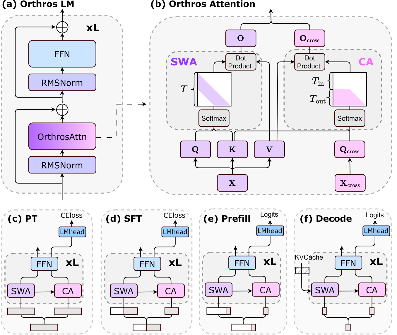
Figure 1: Overview of Orthros attention. The top two sub-figures describe the Orthros architecture and the bottom four sub-figures show the comparison of four sequence-processing regimes. SWA stands for sliding window attention, and CA stands for full cross-attention.
