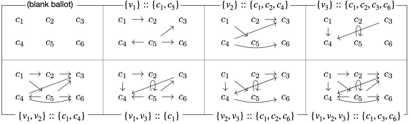
Figure 1: The first row from left to right: a blank ballot; v_1 's ballot approving c_1 and c_5 ; v_2 's ballot approving c_1, c_2 and c_4 ; and v_3 's ballot approving c_1, c_2, c_3 and c_6 . The second row from left to right: \{v_1, v_2\} 's collective approval of c_1 and c_4 ; \{v_1, v_3\} 's collective approval of c_1 ; \{v_2, v_3\} 's collective approval of c_1, c_2 and c_6 ; and \{v_1, v_2, v_3\} 's collective approval of c_1, c_3 and c_6 .
