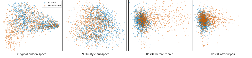
Figure 4: Representation visualization at layer 24. From left to right: the original representation space, the Nullu-style subspace, and the ResOT residual subspace before and after repair. Faithful and hallucinated representations are evaluated on the held-out split. We use PCA for visualization.
