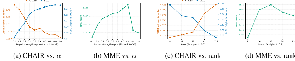
Figure 7: Sensitivity analysis of the repair strength \alpha and residual subspace rank on LLaVA-1.5. For \alpha sensitivity, we fix the rank to 32. For rank sensitivity, we fix \alpha to 0.7.
