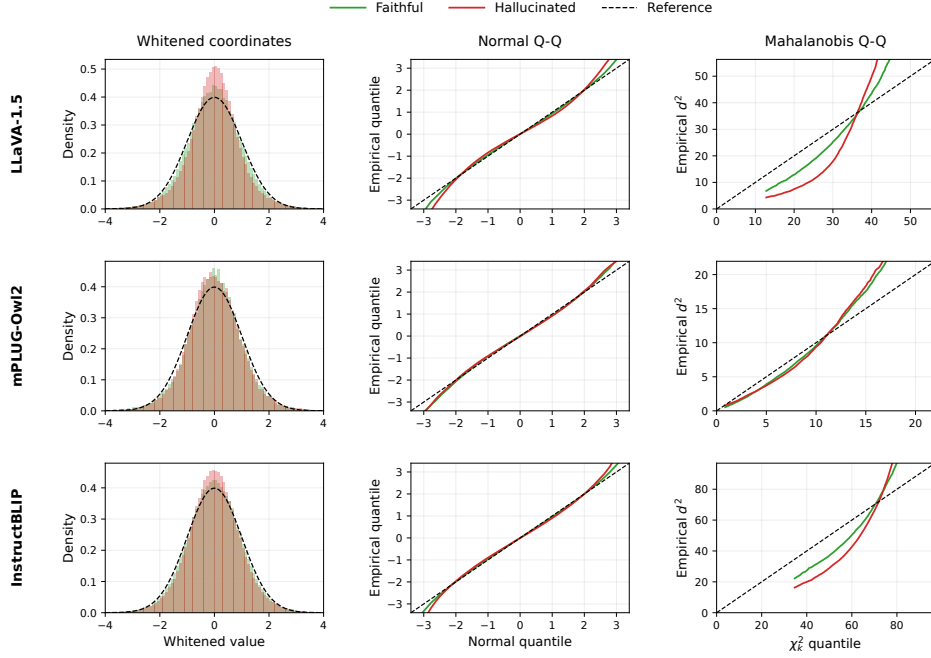
Figure 8: Gaussian diagnostics at layer 31. Columns show histograms of whitened coordinates (left), normal Q-Q plots (middle), and Mahalanobis Q-Q plots (right). Green and red denote faithful and hallucinated representations, respectively. Dashed black lines show the standard normal reference in the histograms and y = x in the Q-Q plots.
