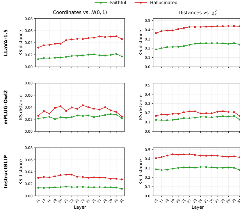
Figure 9: Gaussian diagnostics across layers 16–31. Columns report the KS distance of whitened coordinate values to N(0, 1) (left) and the KS distance of squared Mahalanobis distances to \chi^2_k (right). Green and red curves denote faithful and hallucinated representations, respectively.
