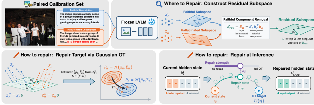
Figure 2: Overview of ResOT. Where to repair (top): the orange hallucinated directions are projected away from the blue faithful subspace to form the green residual subspace. How to repair (bottom): Gaussian OT aligns the orange and blue residual distributions to define repair targets (left); a likelihood-based gate controls the movement toward each target during inference (right).
