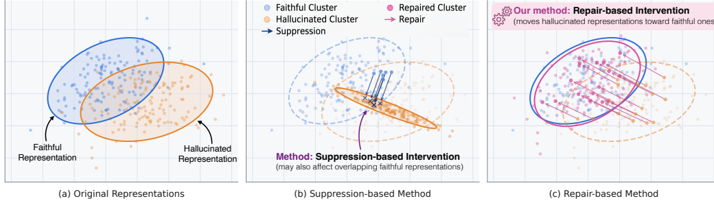
Figure 1: Conceptual comparison of suppression and repair. (a) Faithful (blue) and hallucinated (orange) representations form partially overlapping clusters. (b) Suppression compresses the orange cluster into a narrow band and also displaces some faithful points (blue arrows). (c) Repair instead moves the orange points toward the blue cluster (pink arrows), forming the repaired cluster in pink.
