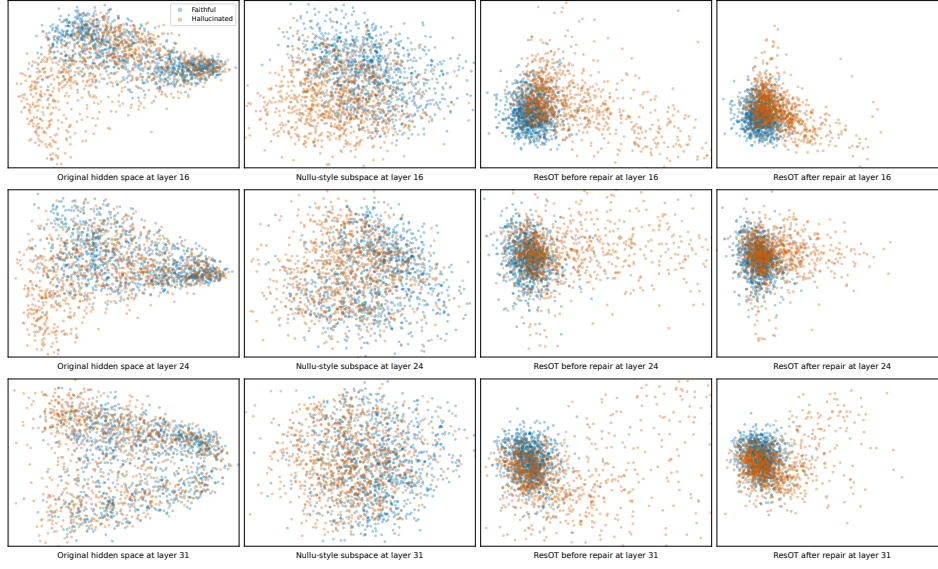
Figure 6: Representation visualizations across layers. Rows correspond to layers 16, 24, and 31. Columns show the original representation space, the Nullu-style subspace, and the ResOT residual subspace before and after repair. We use PCA for visualization.
