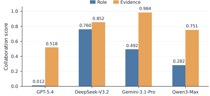
Figure 6 Role Diversity (RD) and Evidence Integration (EI) across models, labeled Role and Evidence in the plot. Their mean is Observable Collaboration Score (OCS).
