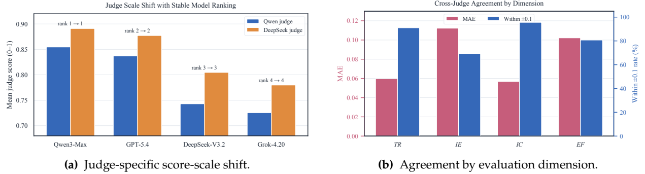
Figure 9 Cross-judge robustness of tool-use evaluation on the 0–1 scale. (a) Average judge scores by model. (b) Agreement on Tool Relevance (TR) , Invocation Efficiency (IE) , Information Coverage (IC) , and Evidence Faithfulness (EF) , measured by mean absolute error (MAE) and the fraction of paired scores within 0.1 points.
