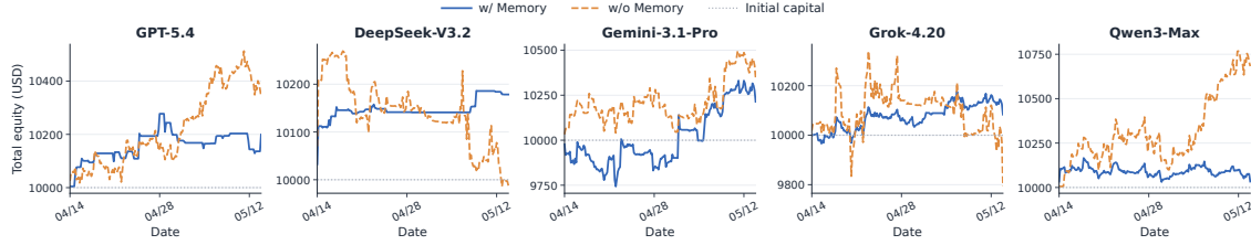
Figure 10 Account-equity trajectories for all ten matched accounts over the full evaluation period. Solid lines denote w/ MEM and dashed lines denote w/o MEM. The largest matched downside differences are visible for Grok-4.20 and DeepSeek-V3.2;
