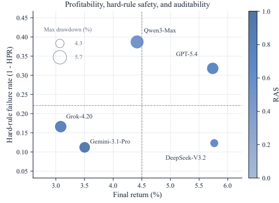
(b) Profitability, hard-rule safety, and auditability.
