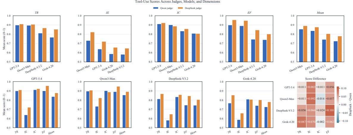
Figure 8 Judge-specific scores for the four tool-use dimensions across Tool-Augmented ReAct agents: Tool Relevance (TR) , Invocation Efficiency (IE) , Information Coverage (IC) , and Evidence Faithfulness (EF) . Scores are shown on a 0–1 scale.
