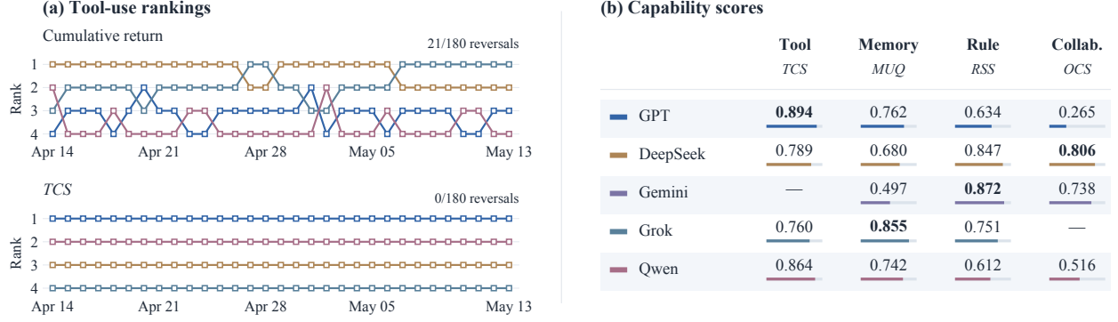
Figure 2 Capability evaluation in a shared market environment. (a) Daily cumulative-return and Tool Call Score (TCS) rankings for the same Tool-use accounts. Rank 1 is highest; annotations count pairwise reversals among comparable pairs. (b) Full-period TCS, Memory Usage Quality (MUQ), Rule Satisfaction Score (RSS), and Observable Collaboration Score (OCS), all on [0, 1] . Colors identify models; bold marks each dimension’s highest score, and dashes indicate unavailable scores. Rankings for the other dimensions are shown in Appendix C.7.
