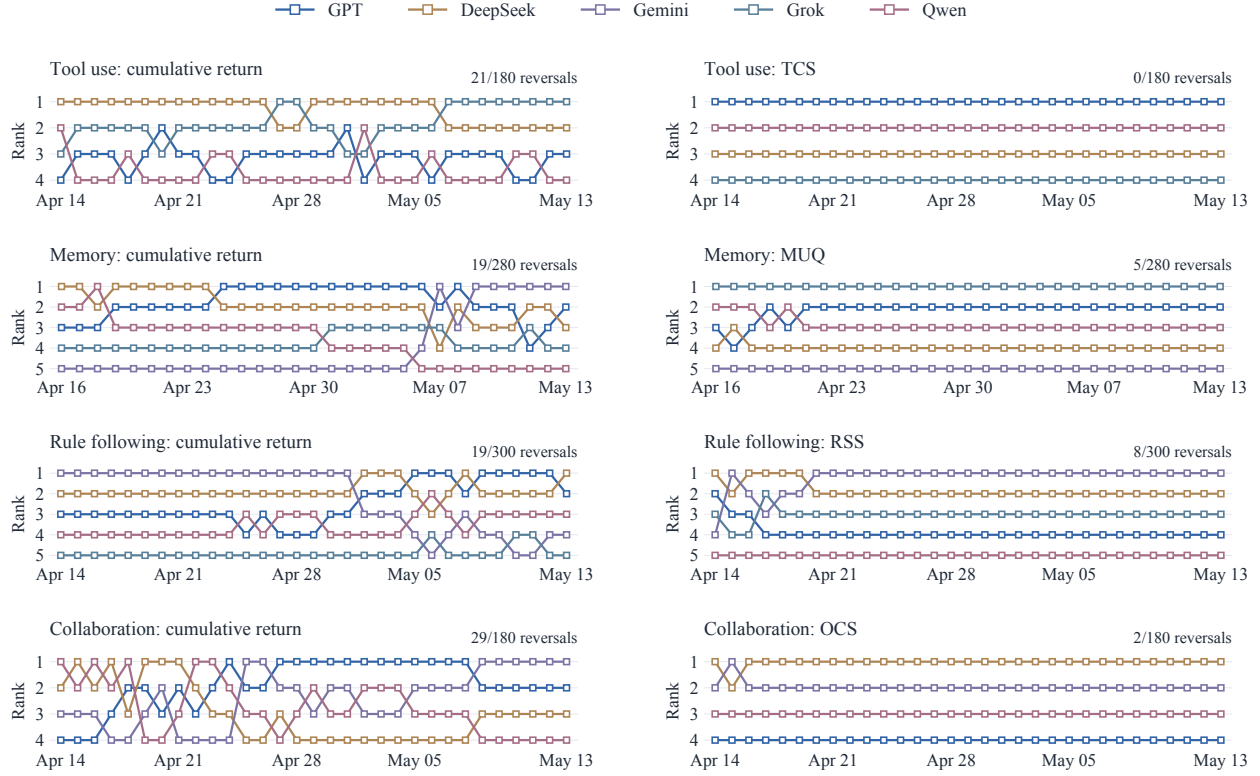
Figure 13 Daily cumulative-return and capability rankings for tool use, memory, rule following, and collaboration. Capability scores are computed from all available evaluation records from the experiment start through each observation time: Tool Call Score (TCS) , Memory Usage Quality (MUQ) , Rule Satisfaction Score (RSS) , and Observable Collaboration Score (OCS) . Each row compares matched accounts and observation times; rank 1 is highest. Annotations count pairwise ranking reversals among comparable pairs.
