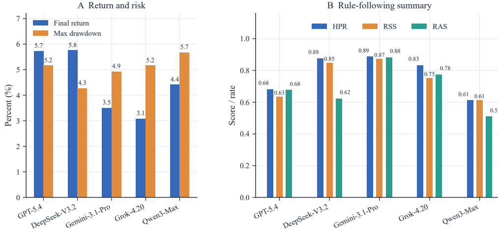
Figure 11 Overall trading and rule-following results across models. The left panel reports final return and maximum drawdown (MDD); the right panel reports Hard-rule Pass Rate (HPR) , Rule Satisfaction Score (RSS) , and Rule Auditability Score (RAS) .
