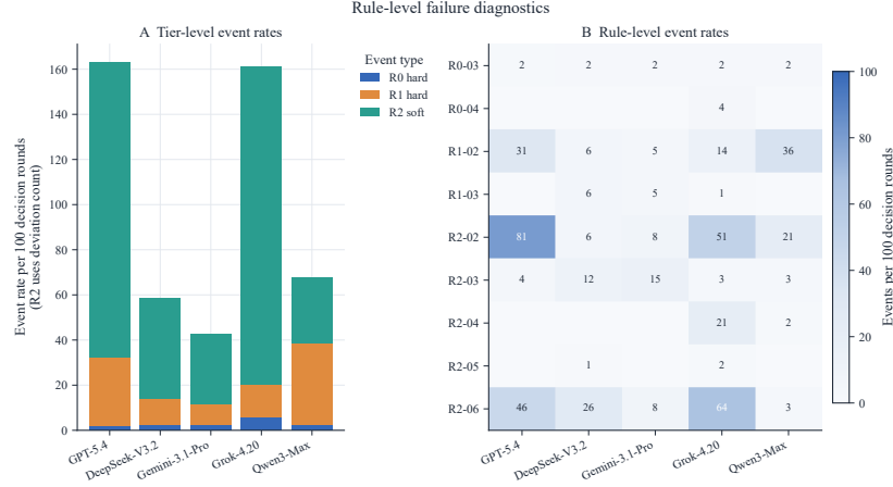
(a) Rule-level hard-rule violations and soft-rule deviations.
