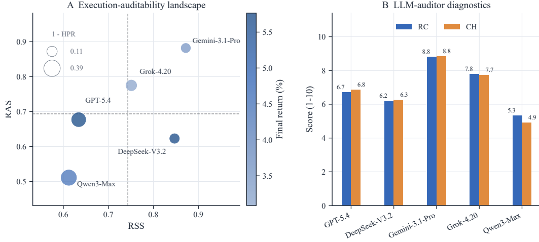
Figure 4 Rule execution and auditability across models. (a) RSS versus RAS, with marker color indicating final return and dashed lines denoting cross-model means. RSS denotes Rule Satisfaction Score , and RAS denotes Rule Auditability Score . (b) LLM-auditor diagnostic scores, where RC denotes Rule Coverage and CH denotes Conflict Handling .
