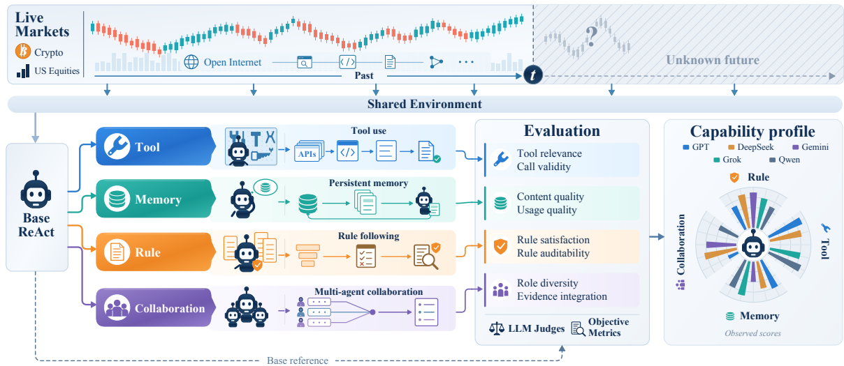
Figure 1 LIVEMACEBENCH overview. Agents interact with a shared, continuously evolving live-market environment along persistent trajectories. Evaluation combines realized outcomes with mechanism-specific process diagnostics to distinguish task performance from how effectively agents use each mechanism.
