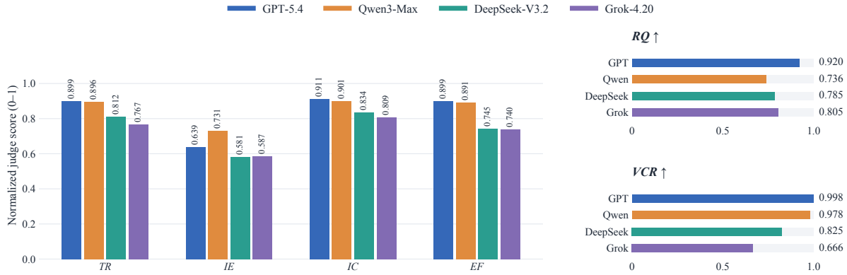
Figure 3 Tool-use capability components across four models. Left: Judge scores produced by Qwen3.5-397B-A17B over 170 traces per evaluated backbone: Tool Relevance (TR), Invocation Efficiency (IE), Information Coverage (IC), and Evidence Faithfulness (EF). Right: Routing Quality (RQ) and Valid Call Rate (VCR). All scores are shown on a 0–1 scale, with higher values indicating better performance. Hallucination-Free Rate (HFR) is omitted because all four models score 1. Additional judge results and complete metrics are provided in Appendix C.3.
