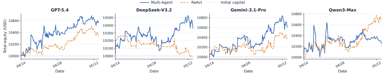
Figure 5 Equity trajectories under Multi-Agent Configuration and Base ReAct Configuration across four backbone models. The dotted line marks the initial capital of $10,000.
