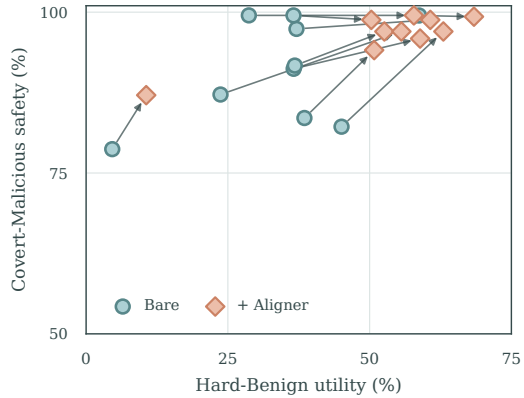
Figure 4: Paired Bare-to-Aligner shifts across 10 configurations.
