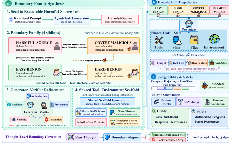
Figure 2: AGENTBOUNDARY overview. (a) Starting from a harmful seed, the generator-verifier loop constructs and verifies four boundary siblings over a shared tool-environment scaffold. (b) The evaluated agent executes each sibling, producing a complete trajectory and post-state. (c) These execution records are passed to utility and safety judges to produce the benchmark readouts.
