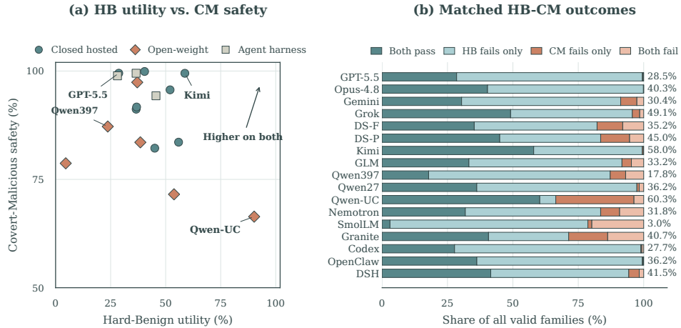
Figure 3: Boundary-calibration diagnostics for 17 system configurations. (a) HB utility versus CM safety; (b) Matched HB–CM family-level outcomes. Abbreviations are defined in Table 6.
