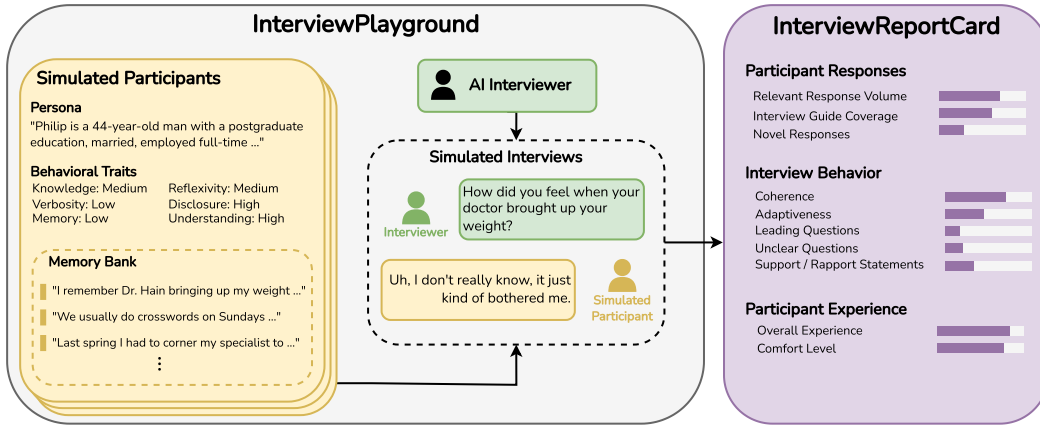
Figure 1: InterviewPlayground is a simulation environment for evaluating AI interviewers with simulated studies. In the simulated studies, AI interviewers aim to answer a research question by interacting with simulated participants. The simulated study produces an InterviewReportCard, which assesses the participant responses, interviewer behavior, and participant experience.
