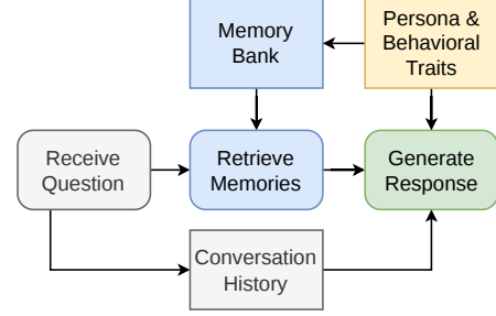
Figure 2: Cognitive model of an Interview-Playground participant.
