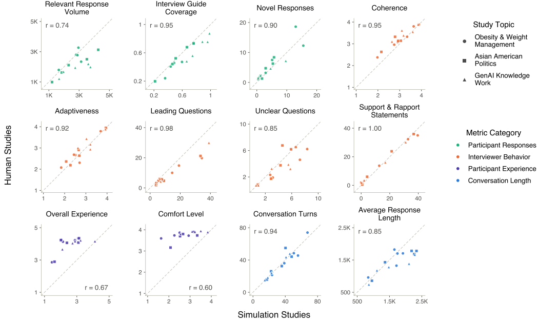
Figure 3: In 10 of the 12 measures, InterviewPlayground’s simulated studies are strongly correlated with the human studies ( r = 0.74 – 1 ). For comfort level and overall experience, they are moderately correlated ( r = 0.60 and r = 0.67 ). Each point represents the average performance of one of five AI interviewers on one of three interview topics. The x-axis shows the results on InterviewPlayground’s simulated studies, and the y-axis shows the results on the human studies.
