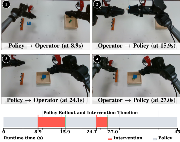
Fig. 7: One AutoIntervene rollout on Peg Disassembly containing two policy–operator–policy intervention cycles. Top: the four control switches. Bottom: the corresponding timeline, with policy control in grey and operator control in red.
