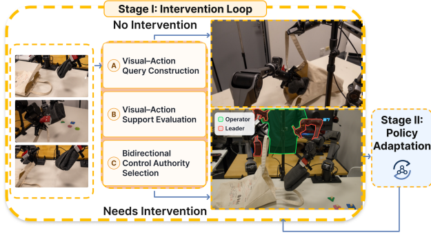
Fig. 2: Overview of AutoIntervene . During Stage I, the intervention loop sequentially (A) constructs a visual-action query from the current visual observations and policy-proposed action chunk, (B) evaluates visual-support and action-risk scores, and (C) selects control authority using calibrated acceptance criteria. The retained intervention segments are subsequently used to adapt the policy in Stage II, after which the updated policy is redeployed.
