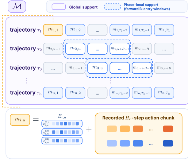
Fig. 3: Memory construction and mode-specific retrieval. \mathcal{R}_{\text{op},t} uses all entries, whereas \mathcal{R}_{\text{pol},t} combines forward B -entry windows from J selected trajectories.
