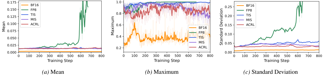
Figure 9. The Training-Inference Discrepancy for Qwen2.5-3B on GSM8K
