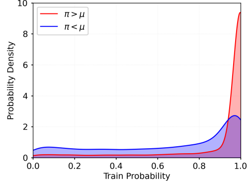
Figure 6. The Probability Density of Training Policy( \pi )
