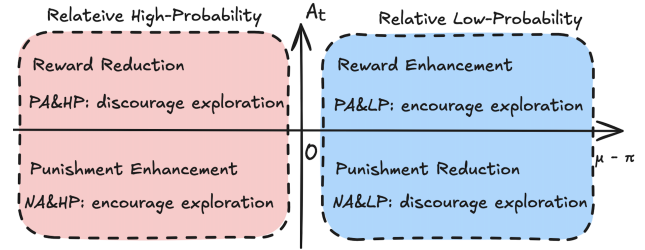
Figure 7. AGPA for Steering Exploration
