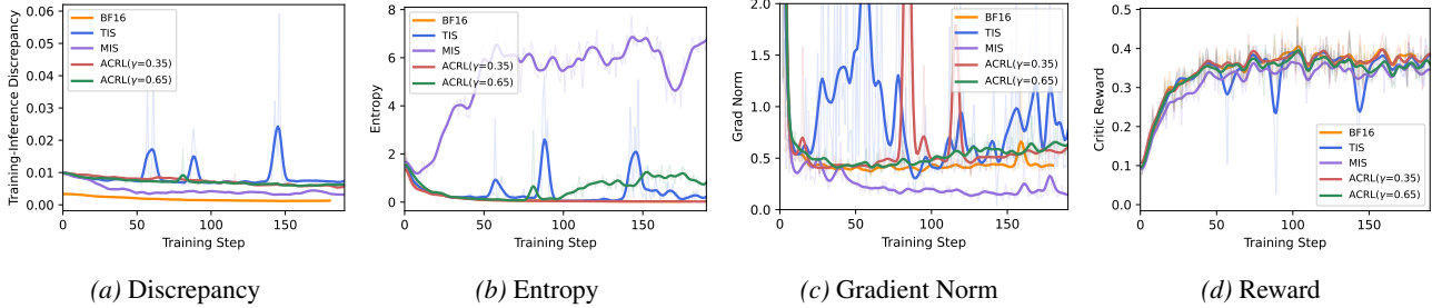
Figure 10. Training-inference discrepancy, entropy, gradient norm, and reward of Qwen2.5-7B on Difficult Mathematical Datasets
