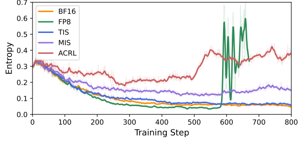
Figure 8. Training entropy for Qwen2.5-3B on GSM8K
