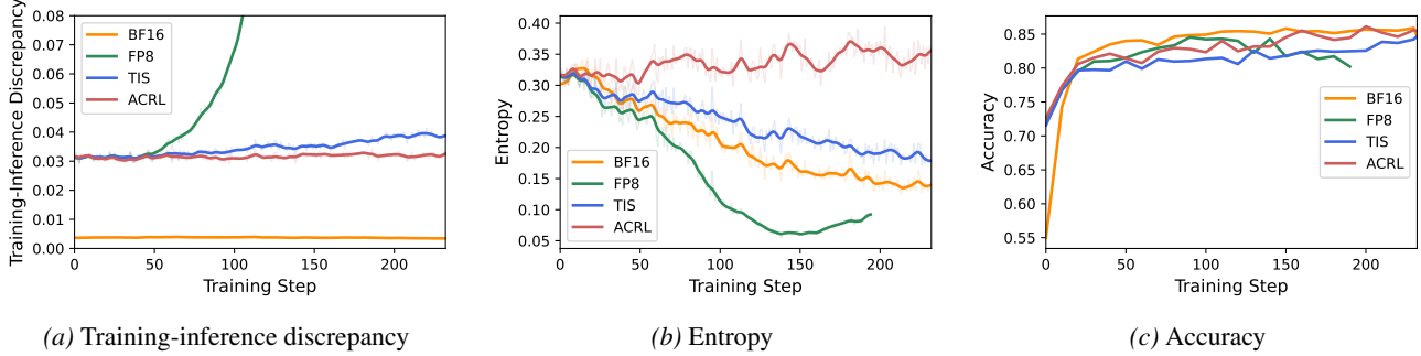
Figure 11. Training-inference discrepancy, entropy, and accuracy of Qwen2.5-3B on GSM8K (Truncated FP8)
