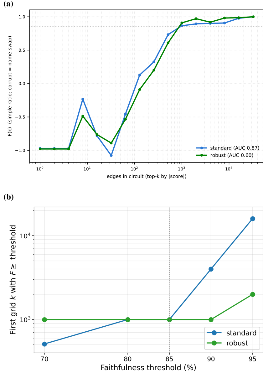
Figure 2: Two readings of the same IOI edge-native faithfulness curve, EAP-IG. (a) F(k) against edges retained, log- k scale: standard and robust cross 85% faithfulness at the same edge count; standard leads by the largest margin in the steep rising region ( k \approx 64 – 512 ); robust is locally ahead near k = 32 and across k \approx 2000 – 16000 ; net area under the curve favors standard (0.87 versus 0.60). (b) First grid point reaching each faithfulness threshold, evaluated on the geometric grid k \in \{1, 2, 4, 8, 16, 32, 64, 128, 256, 512, 1000, 2000, 4000, 8000, 16000, 32491\} ; a reported crossing at k means the true crossing lies in (k', k] for the preceding grid point k' , not at k exactly. The dotted line marks 85%, the threshold used for the single-crossing comparison above; no threshold is a literature standard for this metric, which is why we report the full set of crossings rather than one value.
