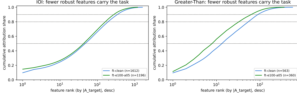
Figure 1: Cumulative attribution share by feature rank (descending |A_i| ), IOI (left) and GT (right). The robust curve reaches each threshold with fewer features in absolute terms; normalized by candidate pool size this reverses (Section 3.3).
