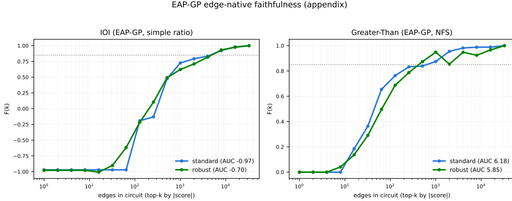
Figure 5: EAP-GP edge-native faithfulness, both tasks. Negative AUC on IOI for both models; EAP-IG is used for the headline result on this basis.
