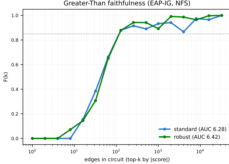
Figure 4: Greater-Than edge-native faithfulness, F(k) , EAP-IG (normalized-faithfulness-score, or NFS, normalization). AUC is an unnormalized trapezoid of F(k) over \ln k (maximum \approx 10.4 if F = 1 throughout the grid); GT’s curve stays near zero or above and rises early, while IOI’s curve dips to F \approx -1.08 before climbing (Table 12), which is why GT and IOI AUCs sit on different numeric scales and are not directly comparable. Not competence-matched between models; not used as evidence for the main result (Section 3.4).
