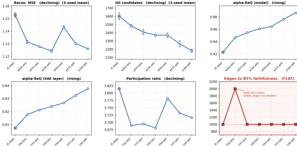
Figure 3: Representational metrics (panels 1–5) move in the predicted direction with adversarial strength across the seven-model sweep, ordered by measured \Delta_{\text{adv}} (1.642 \rightarrow 0.362); two adjacent configurations with near-identical measured robustness (e100-a02, e050-a05) produce small non-monotonic steps in reconstruction MSE and participation ratio. Panel 6 shows the single 85% qualification gate, flat at 1,000 edges except for one outlier (e050-a02, 2,000 edges – larger, not smaller). Reconstruction MSE (inference-threshold mode) and IOI candidates are three-seed means with \pm 1 SD error bars (seeds 42/43/44); \alpha -ReQ, participation ratio, and edges-to-85% are single deterministic measurements per model (Appendix H).
