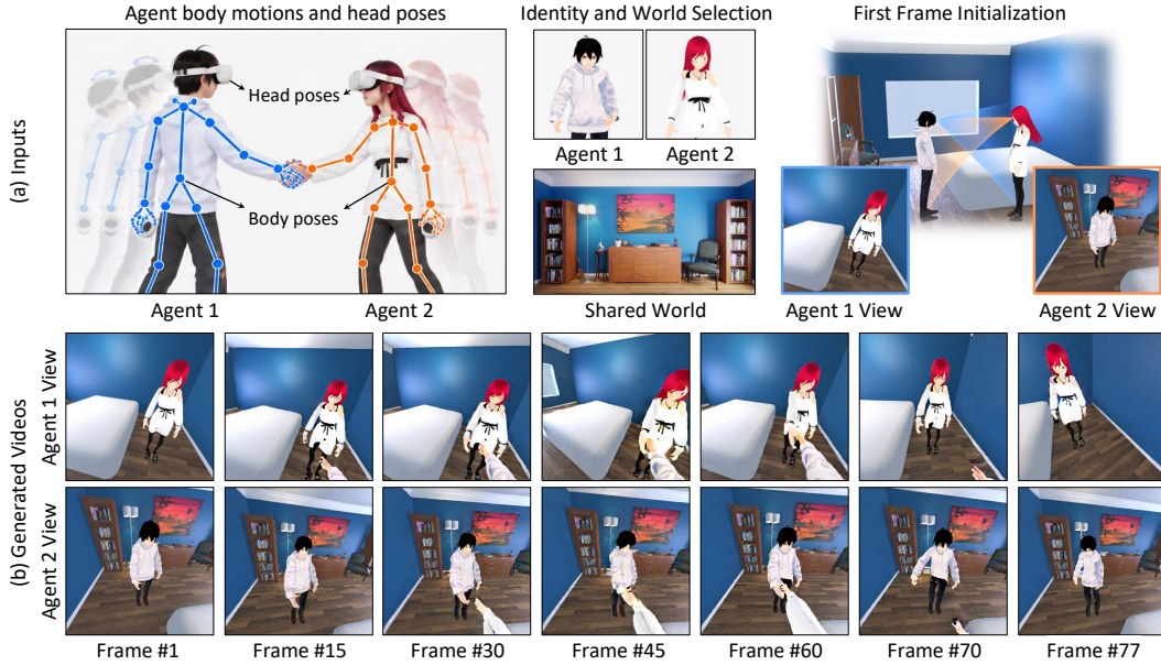
Figure 1: Teaser. Given multi-agent motions, head poses, character identities, and a shared world with first-frame initialization in (a), ME-World jointly generates synchronized ego streams (b) that remain consistent in character identity, scene appearance, and interaction outcomes across agents.
