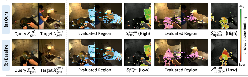
Figure 11: Metric validation. We visualize the query regions evaluated by S_{\text{env}} and S_{\text{update}} , their co-visible correspondences in the target stream, and the resulting DINOv3 cosine similarities. The consistent generation in (a) shows high correspondence similarity and receives higher metric scores, whereas the cross-view inconsistencies in (b) appear as localized similarity drops and lower scores. This correspondence provides qualitative evidence that the proposed metrics capture the intended cross-view consistency. Best viewed zoomed in.
