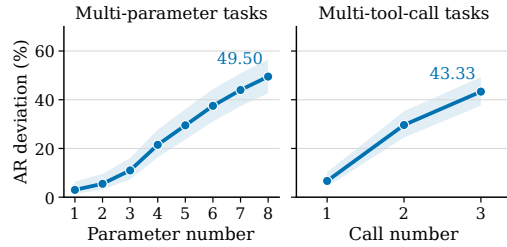
Figure 2: AR deviation from independently generated slot values. Left: BFCL responses with at least eight parameters; right: at least three calls. Each curve follows a fixed cohort as more slots or calls are considered. Shading: 95% Wilson intervals (Wilson, 1927).
