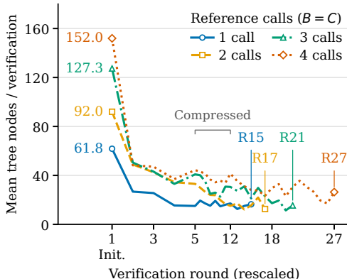
Figure 4: Target-verification workload during SchemaFill decoding. Candidate-node counts peak at slot initialization and drop sharply in subsequent rounds. Curves average requests reaching each round in the Table 3 diagnostic, excluding prompt tokens. Rounds 6–11 are compressed; endpoint labels mark the last rounds with at least 10 contributing requests.
