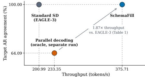
Figure 1: SD denotes speculative decoding. Direct slot-parallel generation can raise throughput but may change the target response. SchemaFill combines parallel proposals with target verification. The direct-parallel baseline follows the skeleton-then-parallel-fill idea of Skeleton-of-Thought (Ning et al., 2024), with the correct skeleton supplied in advance.
