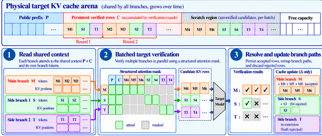
Figure 3: Target-KV cache lifecycle in SchemaFill. The public prefix and verified rows occupy a shared arena, while attention masks restrict branches to valid context and their own candidate paths. One target pass verifies branch scratch rows. Accepted rows extend their cache paths; rejected suffixes are discarded. Only verified tokens on the committed branch become output; a side-branch value must be verified again under the actual output prefix before it can be committed.
