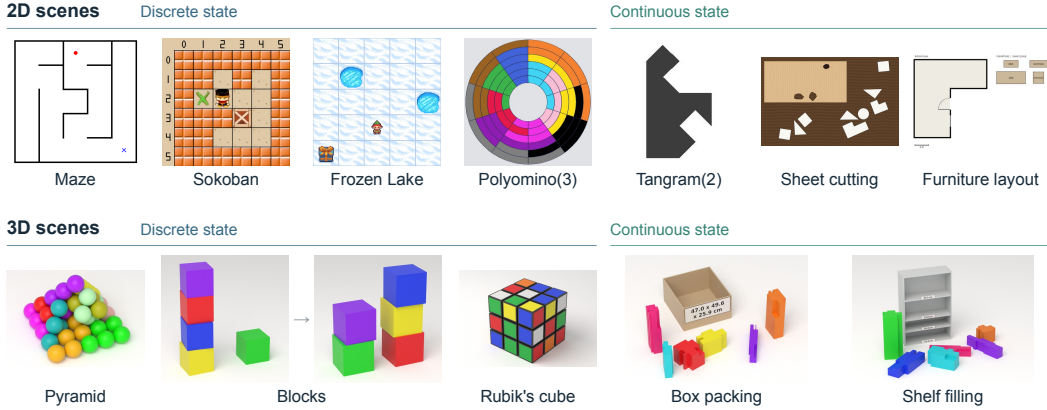
Figure 3: Visual-planning task suite. Representative examples summarize the 15 evaluated domain variants. The 2D domains are shown above the 3D domains, with discrete- and continuous-state domains grouped within each row. Polyomino includes original, affine, and polar variants (polar shown), while tangram includes piece and silhouette variants (silhouette shown).
