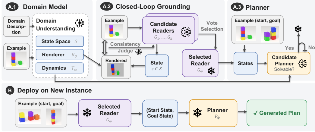
Figure 2: Illustration of RVPA framework. (A) Given a task description and unlabeled examples, the VLM constructs and selects reusable state-reading and planning programs using label-free feedback. (B) These programs are then frozen and applied directly to each new instance, producing plans through local execution without further VLM calls.
