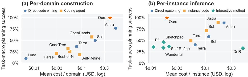
Figure 1: Reusable planning is both capable and efficient. Across diverse visual planning domains, our method achieves the strongest overall success–cost trade-off, outperforming domain-level program-authoring baselines while exceeding costly per-instance inference methods.
