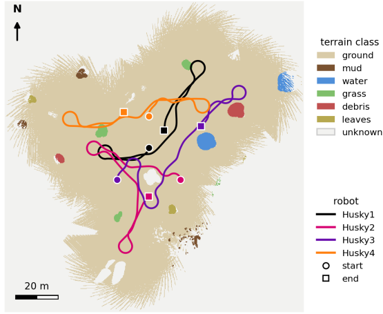
Fig. 3. Fused semantic ground map and robot trajectories after a 600 s run with four ground robots. Circles mark start poses, squares mark final poses.
