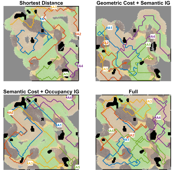
Fig. 2. Final fused semantic maps for a representative paired run after 300 s. Colored lines show robot trajectories, black cells are obstacles, and gray cells are unexplored.
