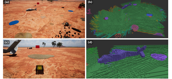
Fig. 1. Distributed semantic multi-robot exploration in HERCULES. (a) The outdoor arena, with terrain patches of differing traversability alongside structures and debris. (b) The 3-D semantic voxel map accumulated online by the team, colored by inferred class. (c) A Husky ground robot exploring the arena. (d) A reconstructed aircraft and adjacent terrain patch.
