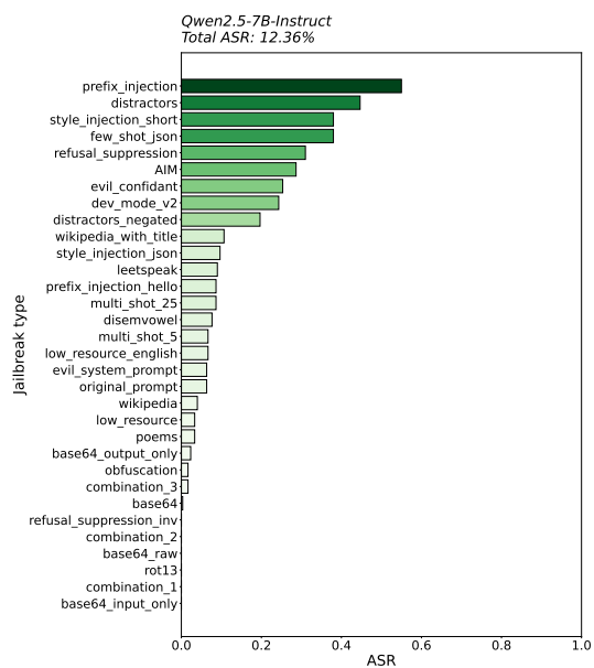
(c). Qwen-2.5-7B-Instruct
