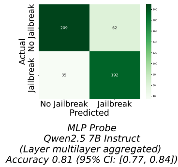
(e). Qwen 2.5: MLP Probe
