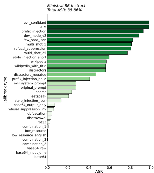
(b). Mistral-8B-Instruct
