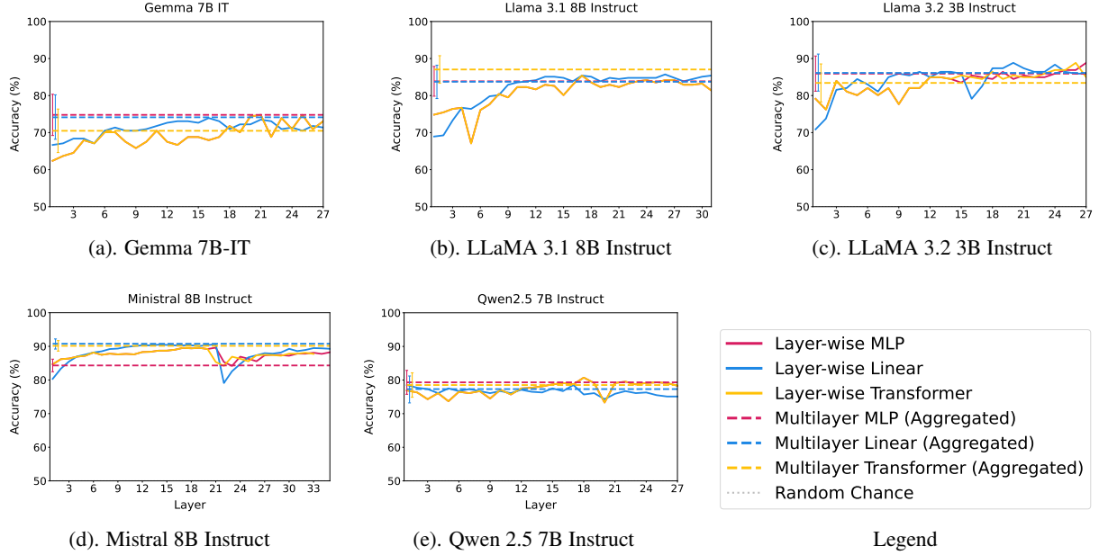
Figure 3: Probe tends to increase with layer depth. Vertical lines show confidence intervals for probe accuracy. Y-axis minimum represents random chance. See Section 4.4 for intervention details and Section D for exact values.
