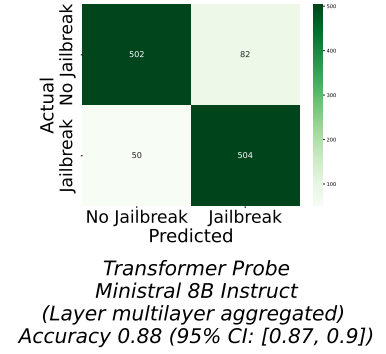
(c). Mistral: Transformer Probe
