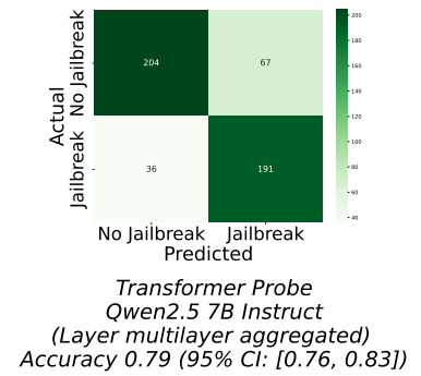
(f). Qwen 2.5: Transformer Probe
