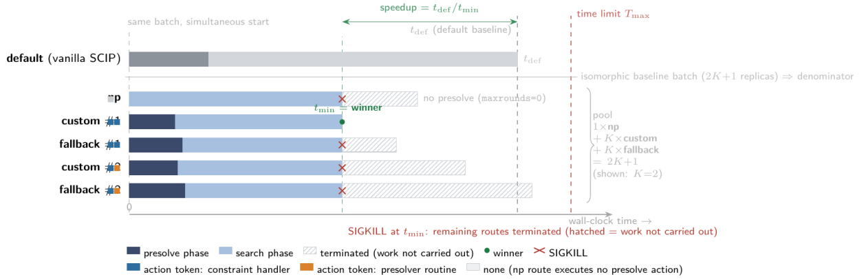
Figure 3: The deployment form and measurement protocol of concurrent racing. Pool = np + content \times K + fallback \times K = 2K + 1 paths launched together; the first to finish wins and the others are withdrawn (SIGKILL); the numerator is the solver-internal time of the winner, and the denominator is the internal clock of the replica of the isomorphic default strategy selected as the first to finish, so the speedup shown in the figure is the ratio reading with which that instance enters SGM.
