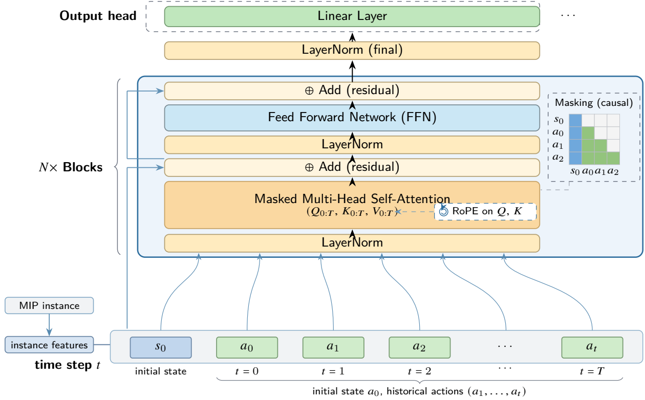
Figure 2: Structure and conditioning of the sequence generation model. Instance features are fed as the initial state concatenated with the historical action tokens, and causal self-attention (rotary position embedding, RoPE, applied to Q/K ) autoregressively predicts the next item; round boundaries and the terminator share one output space with the actions, so that "in what order and at which round to execute" is given by the same distribution.
