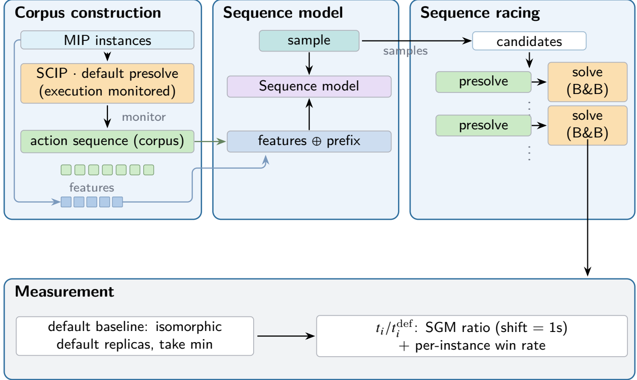
Figure 1: The four-stage pipeline of the method in this paper. Corpus construction and sequence modelling are each performed once offline; the online part performs only per-instance decoding and sequence racing; the measurement layer takes the solver-internal time of the isomorphic default strategy as the denominator and reports the SGM ratio and the per-instance win rate.
